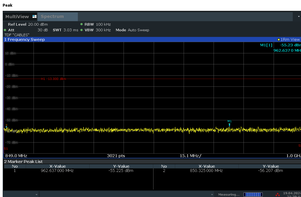
Plot 7-20. Conducted Spurious Plot (WCDMA Ch. 4132)
