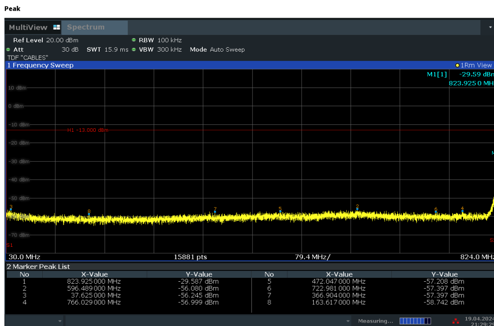
Plot 7-19. Conducted Spurious Plot (WCDMA Ch. 4132)
