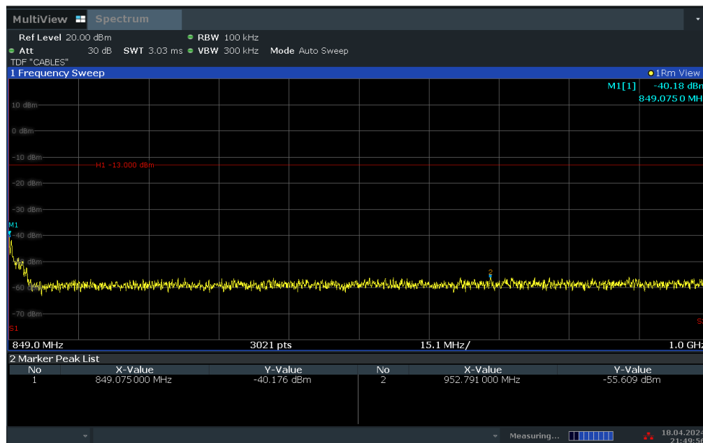
Plot 7-17. Conducted Spurious Plot (LTE Band 26/5 - 10MHz QPSK - RB Size 1, RB Offset 0 - High Channel)
