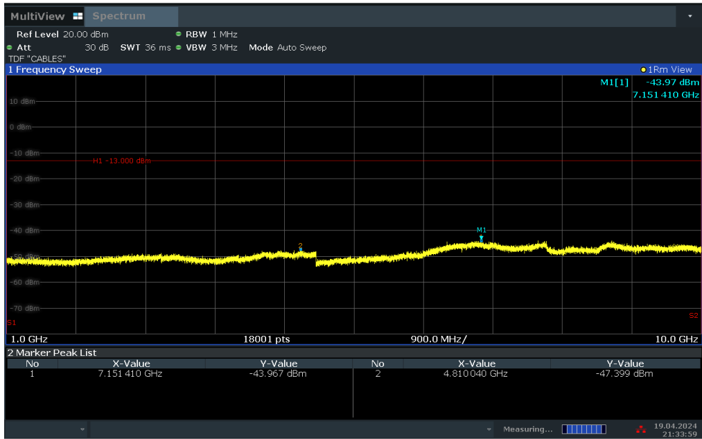
Plot 7-27. Conducted Spurious Plot (WCDMA Ch. 4233)
