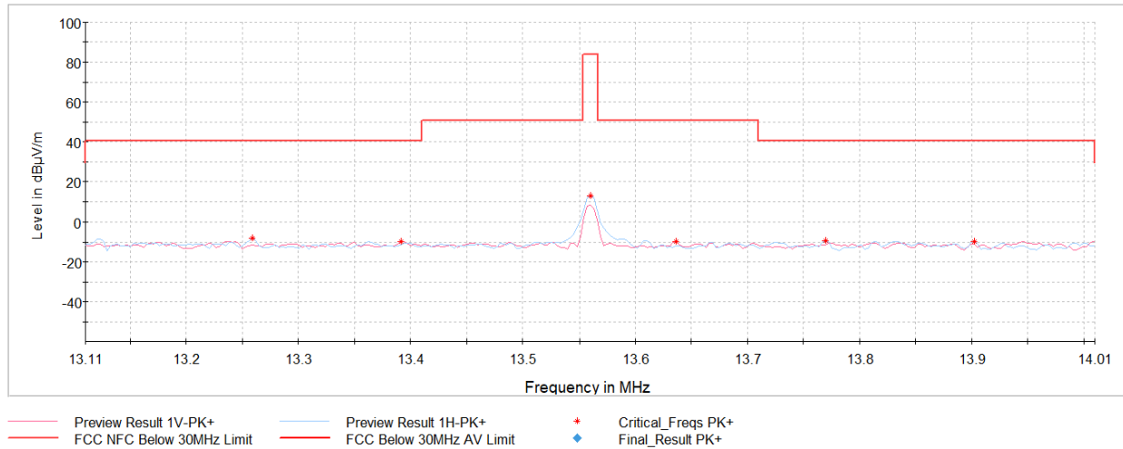
Plot 7-6. In Band Radiated Spurious Emissions (CE F 212kbps, with AC/DC Adapter and Magnetic Charger)
