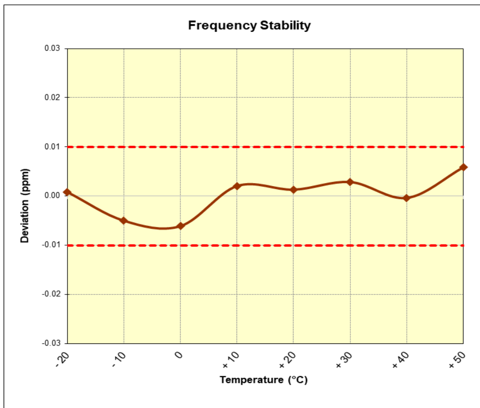
Figure 7-4. Frequency Stability Plot (Reader Type A 848 kbps)
