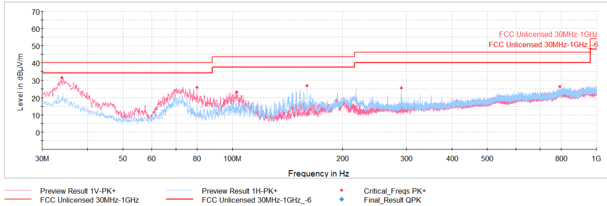
Plot 7-10. Radiated Spurious Emissions 30MHz – 1GHz (CE F 212kbps, with AC/DC Adapter and Magnetic Charger)
