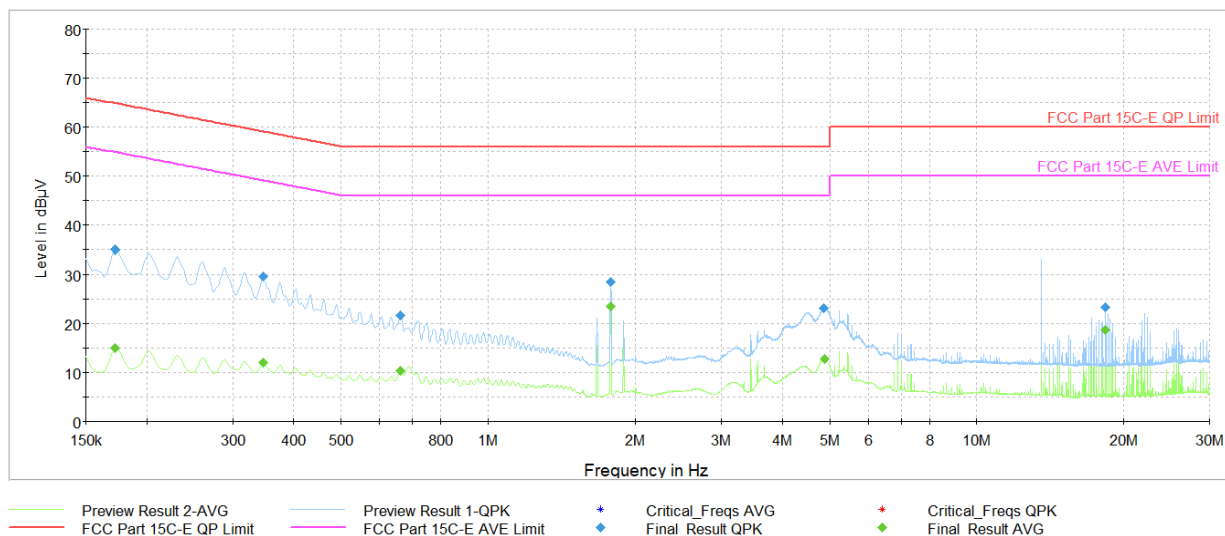
Plot 7-12. AC Line-Conducted Plot (L1, CE F 212kbps, with AC/DC Adapter and Magnetic Charger)
