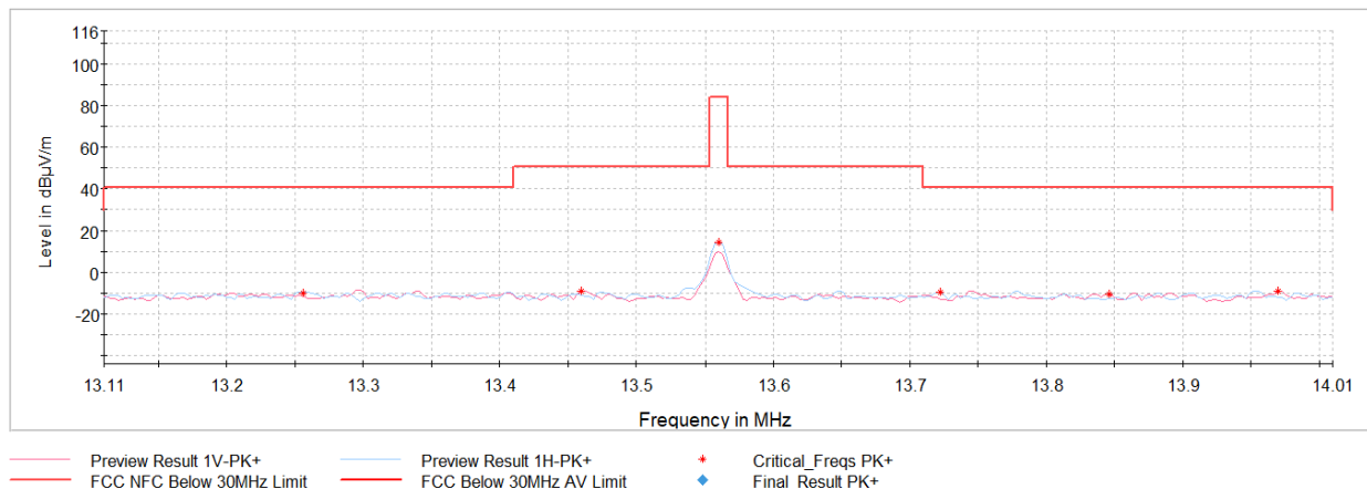
Plot 7-7. In Band Radiated Spurious Emissions (Reader A 848kbps, with AC/DC Adapter and Magnetic Charger)
