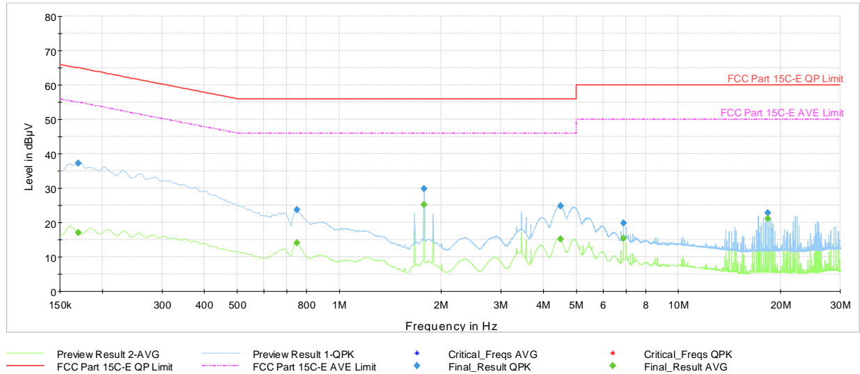
Plot 7-45. AC Line-Conducted Test Plot (N, GFSK ePA – Ch.39, with AC/DC Adapter + Magnetic Charger)
