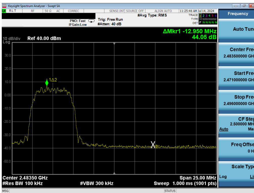
Plot 7-22. Band Edge Plot (Bluetooth (HDR8), ePA – Ch. 73)
