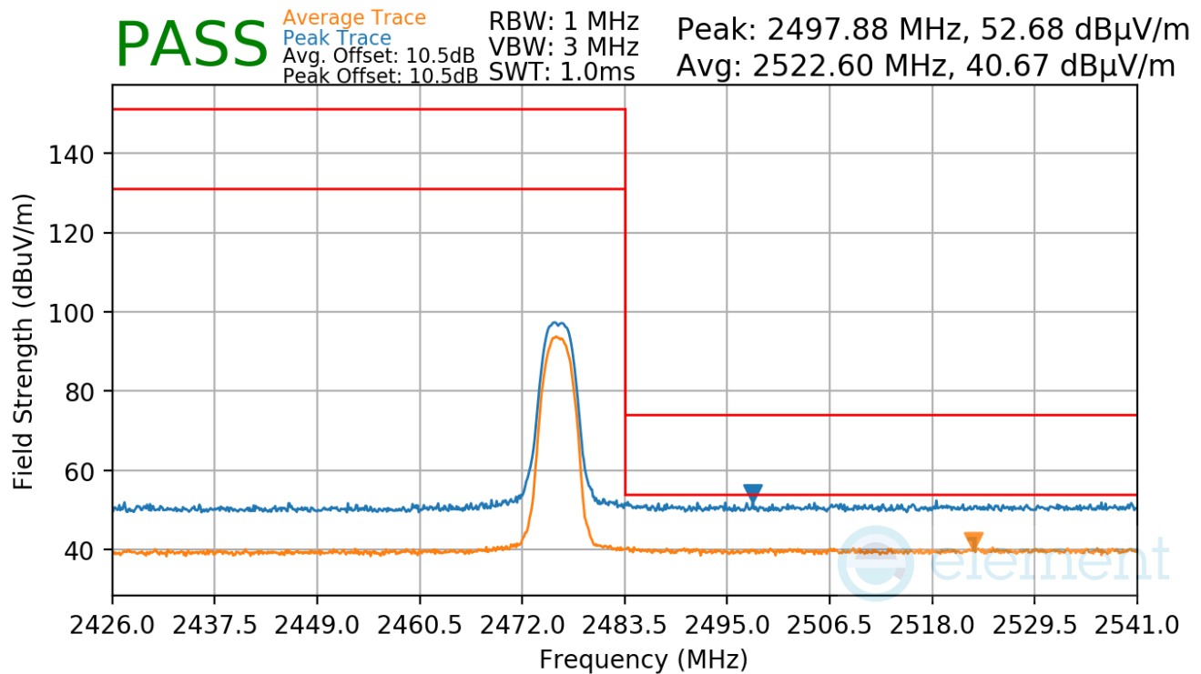
Plot 7-35. Radiated Restricted Upper Band Edge Measurement
