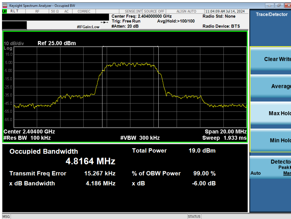
Plot 7-4. 6dB BW & 99% OBW Plot (Bluetooth (HDR8), 8Mbps, ePA – Ch. 1)
