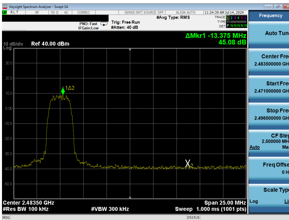
Plot 7-20. Band Edge Plot (Bluetooth (HDR4), ePA – Ch. 73)
