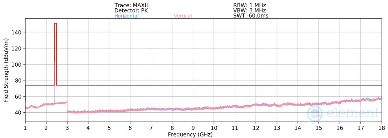
Plot 7-29. Radiated Spurious Emissions 1-18GHz (4Mbps, HDR4, ePA – Ch. 1)
