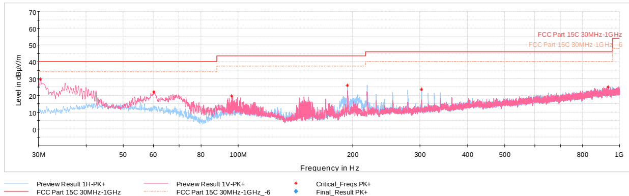
Plot 7-37. Radiated Spurious Emissions Below 1GHz (4Mbps, ePA – Ch.38 with AC/DC Adapter + Magnetic Charger)
