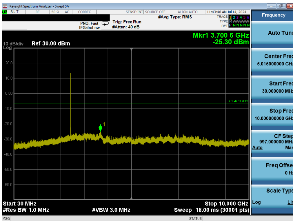
Plot 7-25. Conducted Spurious Plot (Bluetooth (HDR4), ePA – Ch. 38)
