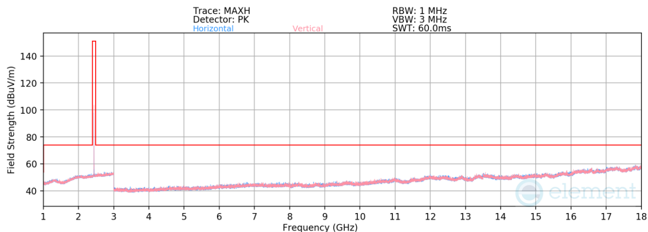
Plot 7-30. Radiated Spurious Emissions 1-18GHz (4Mbps, HDR4, ePA – Ch. 38)
