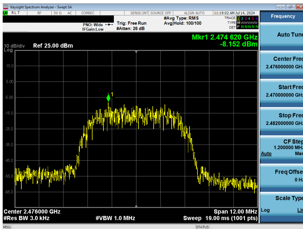
Plot 7-18. Power Spectral Density Plot (Bluetooth (HDR8), 8Mbps, iPA – Ch. 73)
