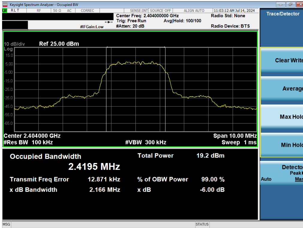
Plot 7-1. 6dB BW & 99% OBW Plot (Bluetooth (HDR4), 4Mbps, ePA – Ch. 1)
