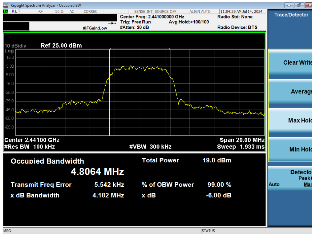
Plot 7-5. 6dB BW & 99% OBW Plot (Bluetooth (HDR8), 8Mbps, ePA – Ch. 38)
