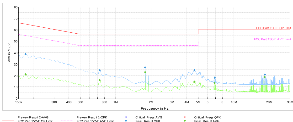
Plot 7-38. AC Line Conducted Plot with Bluetooth HDR (L1, 4Mbps ePA - Ch.38 with AC/DC Adapter + Magnetic Charger)
