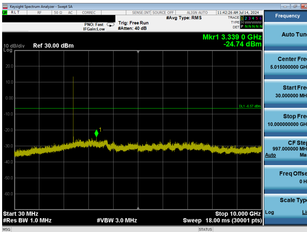
Plot 7-23. Conducted Spurious Plot (Bluetooth (HDR4), ePA – Ch. 1)
