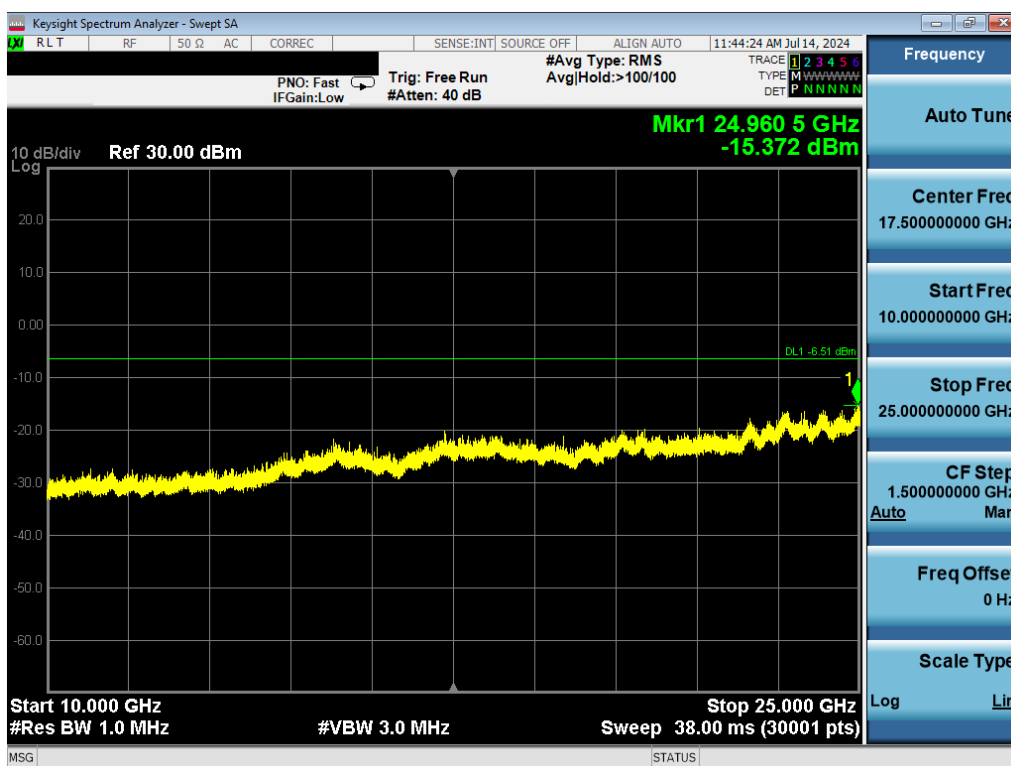
Plot 7-26. Conducted Spurious Plot (Bluetooth (HDR4), ePA – Ch. 38)
