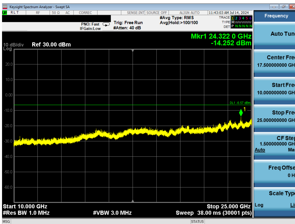
Plot 7-24. Conducted Spurious Plot (Bluetooth (HDR4), ePA – Ch. 1)
