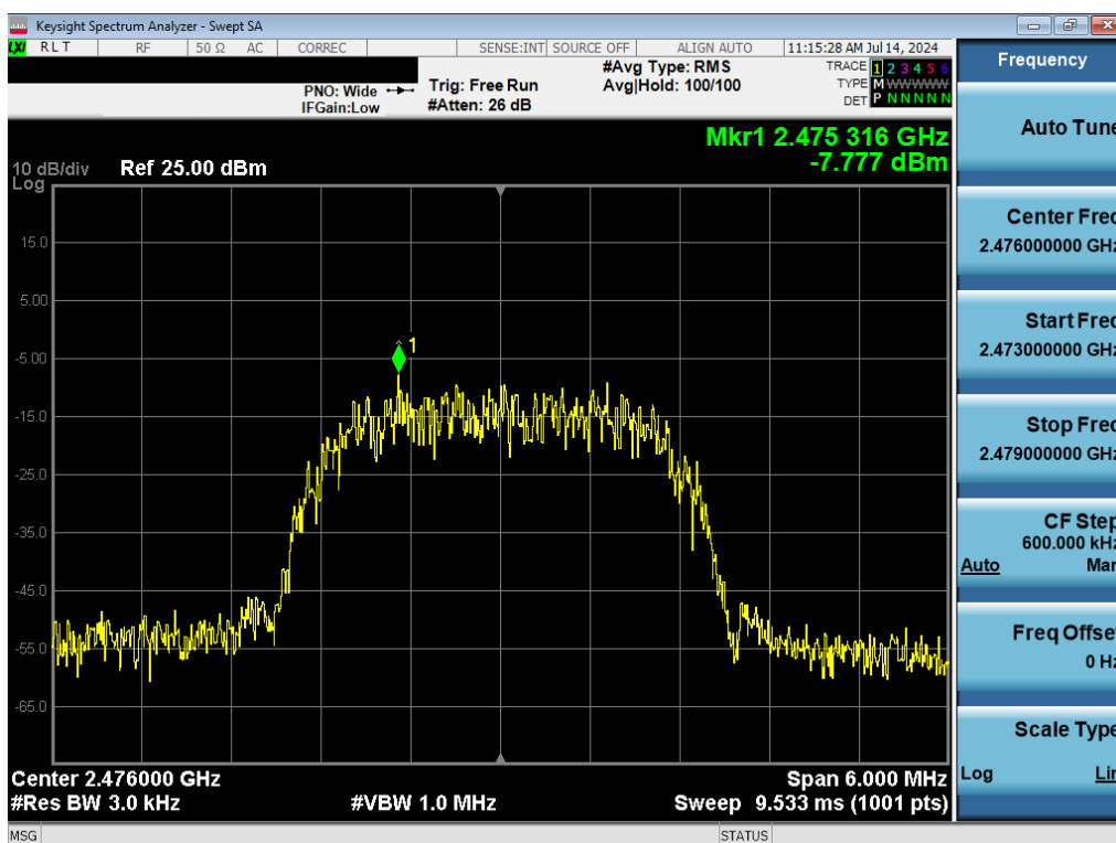
Plot 7-12. Power Spectral Density Plot (Bluetooth (HDR4), 4Mbps, iPA – Ch. 73)
