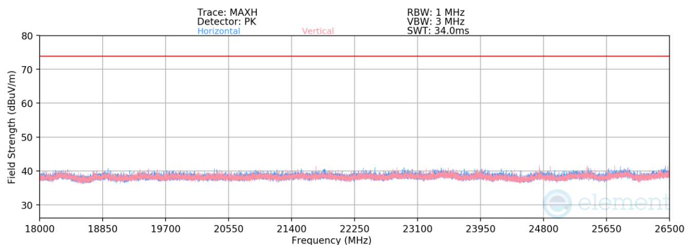
Plot 7-31. Radiated Spurious Emissions Above 18GHz (4Mbps, HDR4, ePA – Ch. 38)
