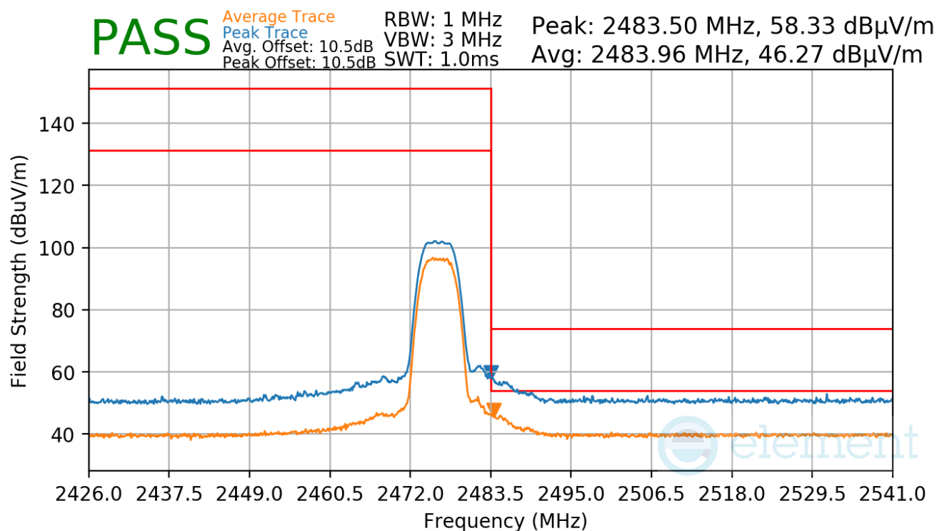
Plot 7-36. Radiated Restricted Upper Band Edge Measurement
