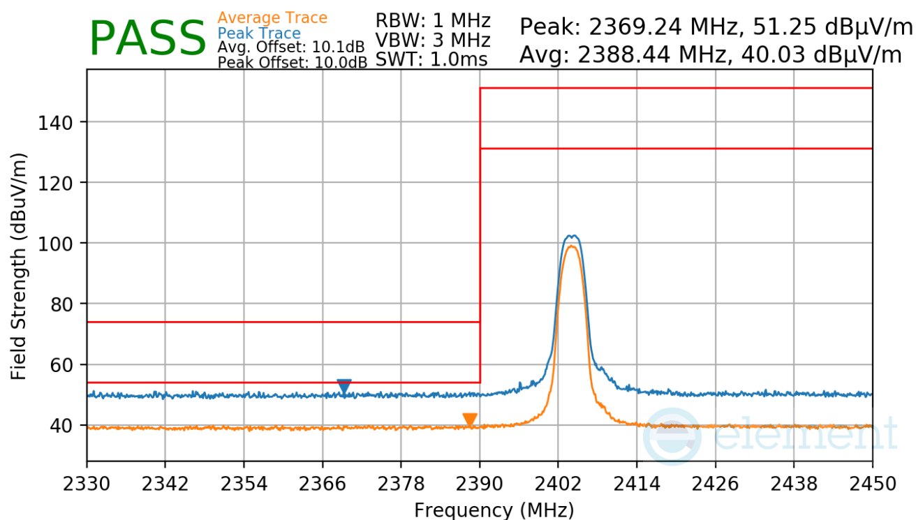
Plot 7-33. Radiated Restricted Lower Band Edge Measurement
