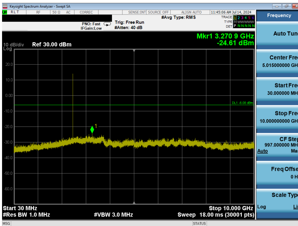
Plot 7-27. Conducted Spurious Plot (Bluetooth (HDR4), ePA – Ch. 73)
