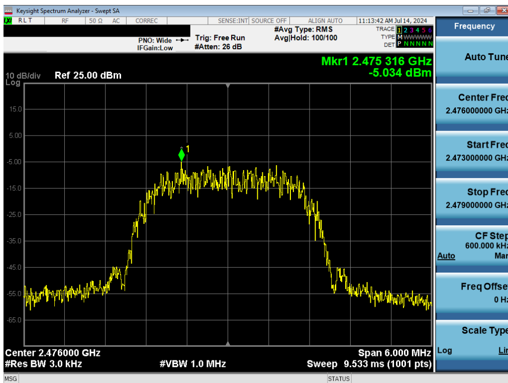
Plot 7-9. Power Spectral Density Plot (Bluetooth (HDR4), 4Mbps, ePA – Ch. 73)
