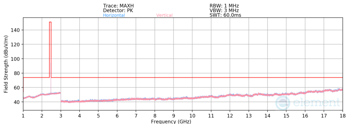
Plot 7-32. Radiated Spurious Emissions 1-18GHz (4Mbps, HDR4, ePA – Ch. 73)
