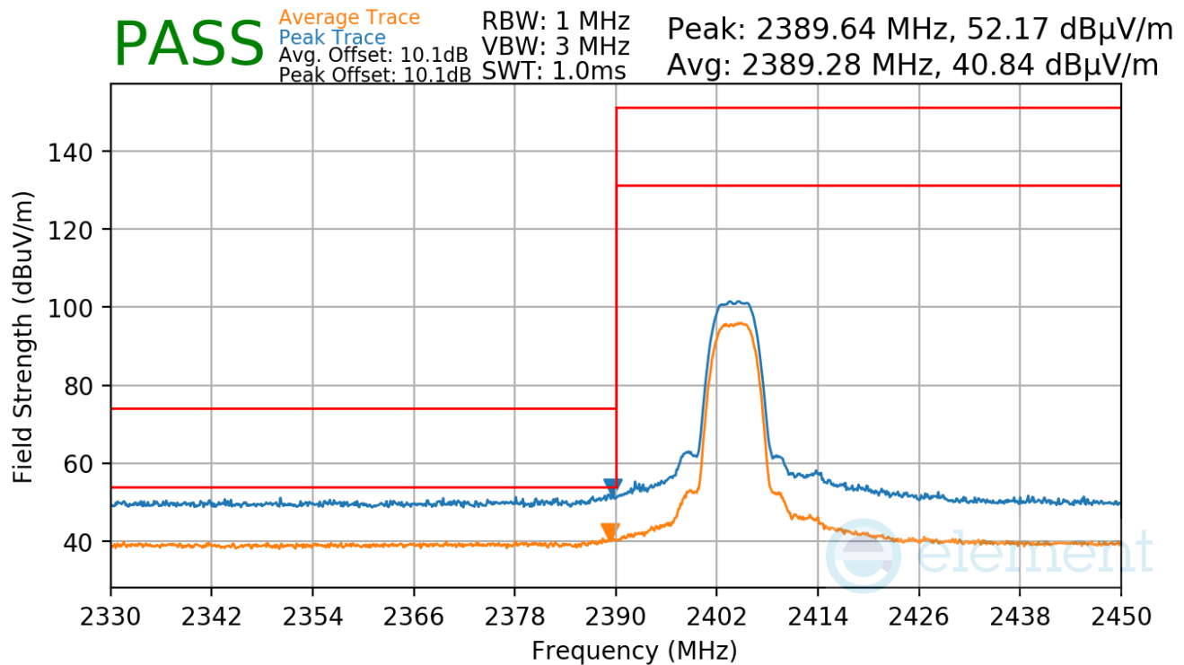
Plot 7-34. Radiated Restricted Lower Band Edge Measurement
