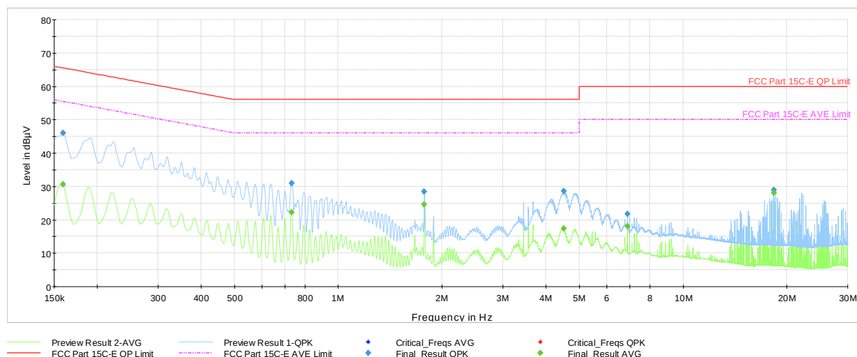
Plot 7-39. AC Line Conducted Plot with Bluetooth HDR (N, 4Mbps ePA - Ch.38 with AC/DC Adapter + Magnetic Charger)
