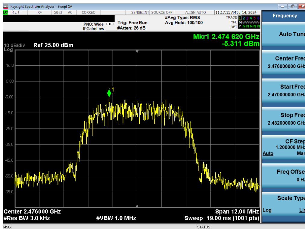
Plot 7-15. Power Spectral Density Plot (Bluetooth (HDR8), 8Mbps, ePA – Ch. 73)
