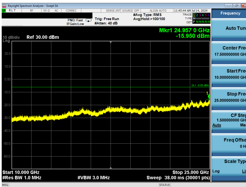
Plot 7-28. Conducted Spurious Plot (Bluetooth (HDR4), ePA – Ch. 73)
