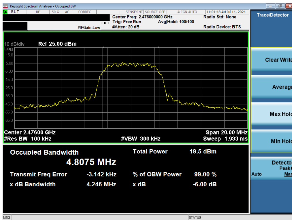
Plot 7-6. 6dB BW & 99% OBW Plot (Bluetooth (HDR8), 8Mbps, ePA – Ch. 73)
