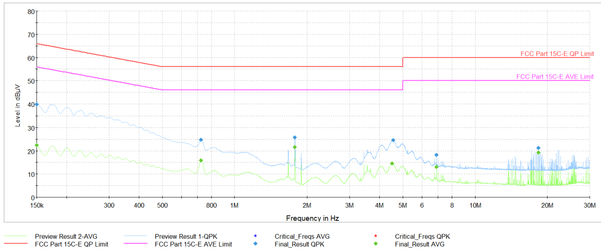
Plot 7-38. AC Line Conducted Plot with Bluetooth LE (L1, 1Mbps ePA – Ch.19 with AC/DC Adapter + Magnetic Charger)
