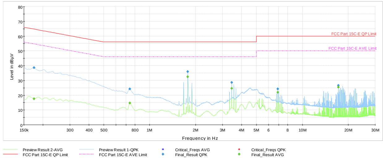
Plot 6-13. AC Line Conducted Plot (L1 - Mode 1, with Laptop via magnetic charger)
