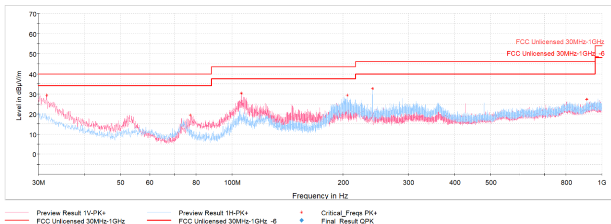
Plot 6-12. Radiated Spurious Emissions 30MHz – 1GHz (Mode 1, with Laptop via magnetic charger)
