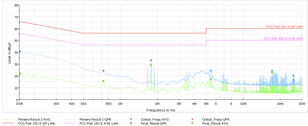
Plot 6-14. AC Line Conducted Plot (N - Mode 1, with Laptop via magnetic charger)
