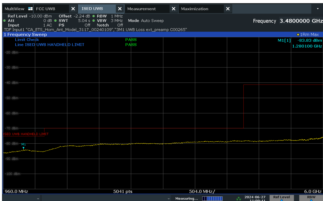
Plot 7-18. ISCED Radiated Spurious Emission 960-6000MHz (Ch. 5, Config 409, Payload 4093 Ant. Pol. V)
