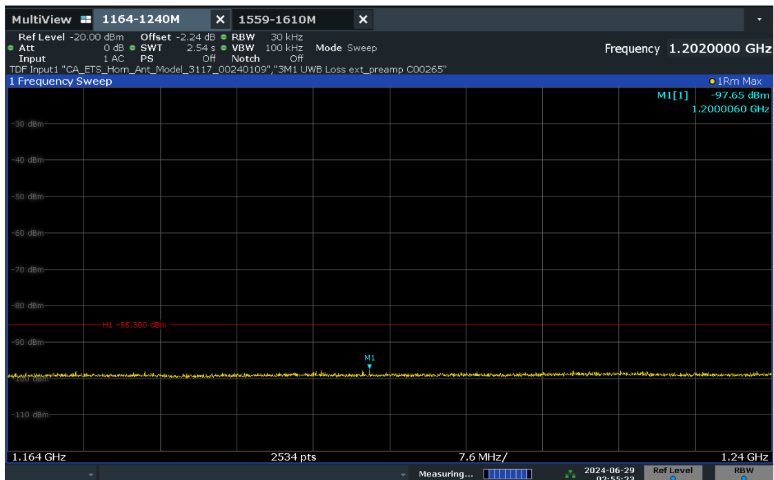
Plot 7-20. Radiated Spurious Emission 1164-1240MHz (Ch. 5, Config 409, Payload 4093 Ant. Pol. V)
