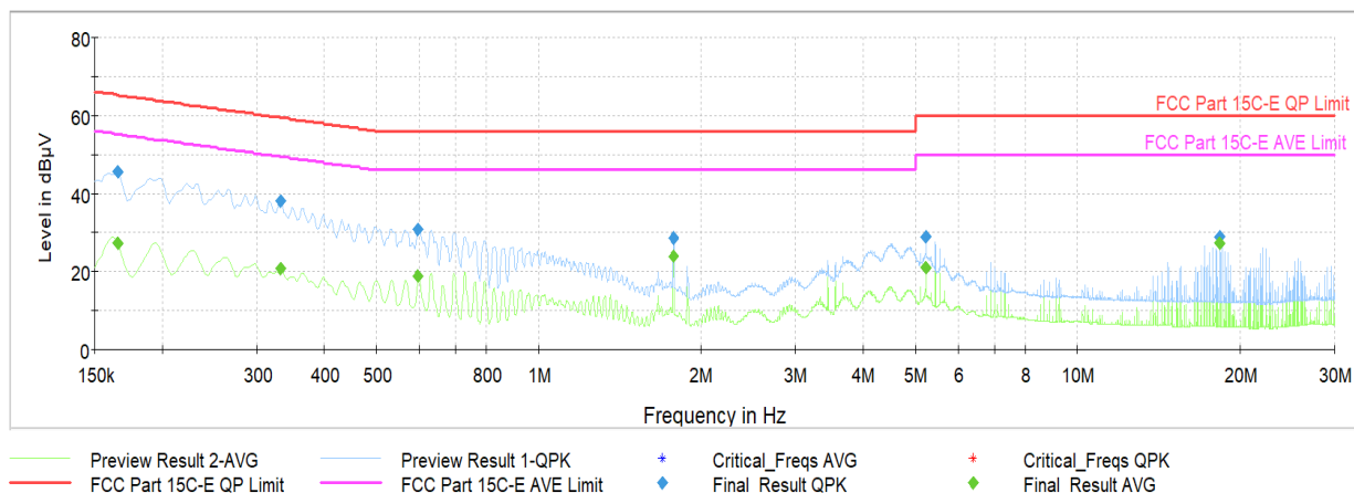
Plot 7-44. AC Line Conducted Plot (Ch. 9, Config 409, Payload 4093 N, with AC/DC Adapter + Magnetic Charger)
