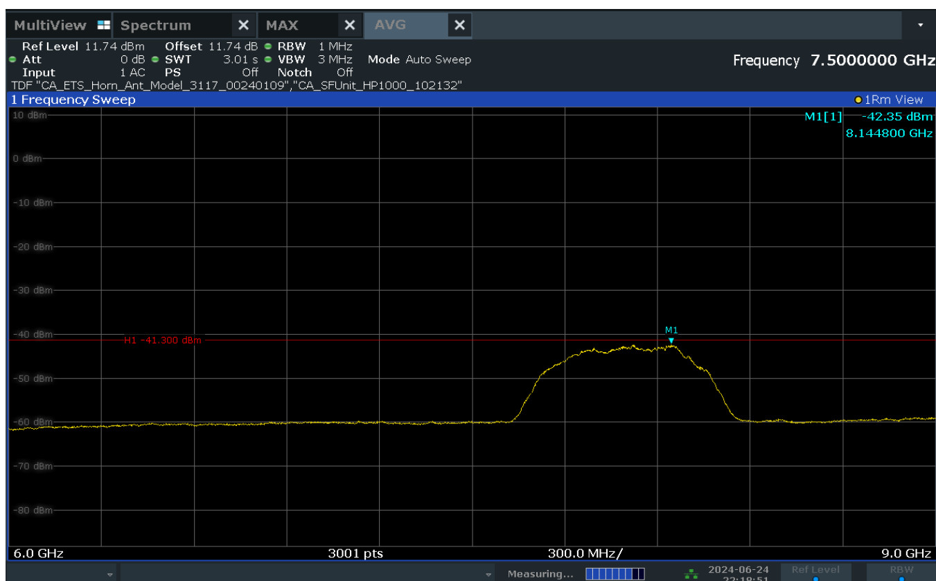
Plot 7-8. Average Radiated Power (Ch. 9, Config 409/Payload 4093)
