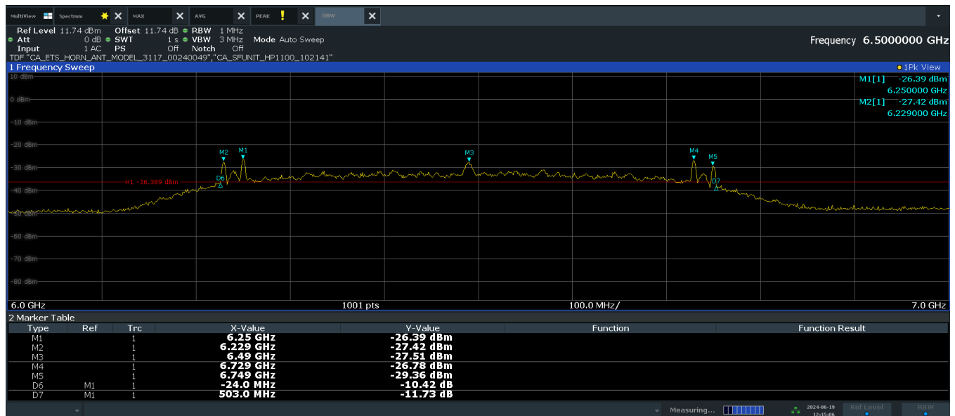
Plot 7-1. 10dBc Bandwidth (Ch. 5, Config 409/Payload 4093)
