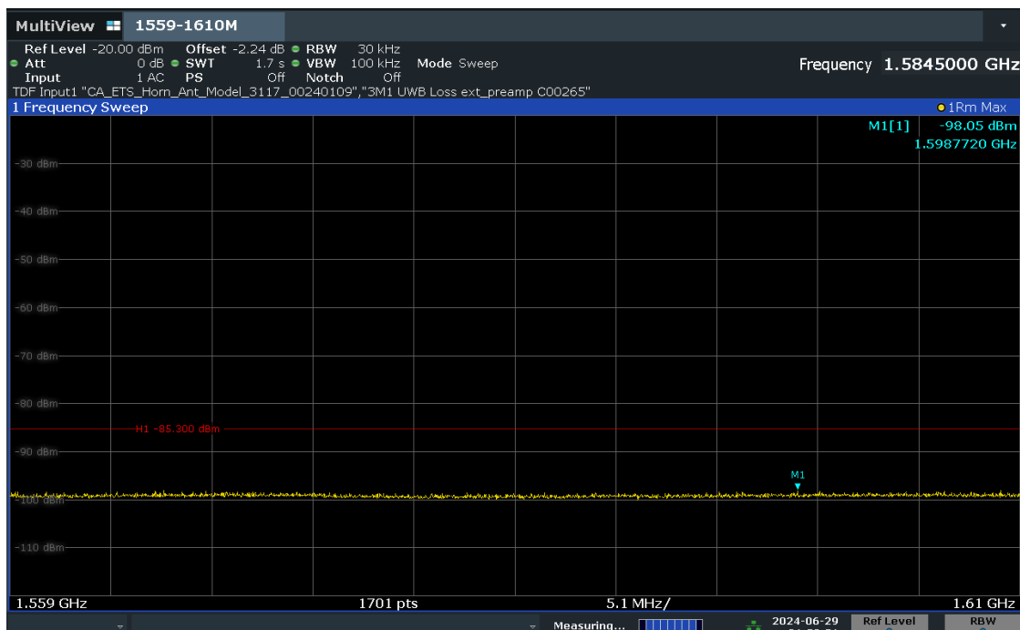
Plot 7-31. Radiated Spurious Emission 1559-1610MHz (Ch. 9, Config 409, Payload 4093 Ant. Pol. H)
