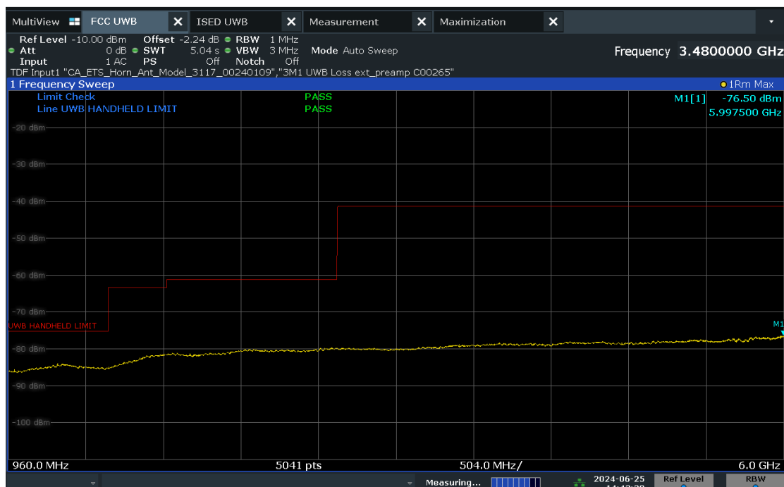
Plot 7-15. FCC Radiated Spurious Emission 960-6000MHz (Ch. 5, Config 409, Payload 4093 Ant. Pol. H)
