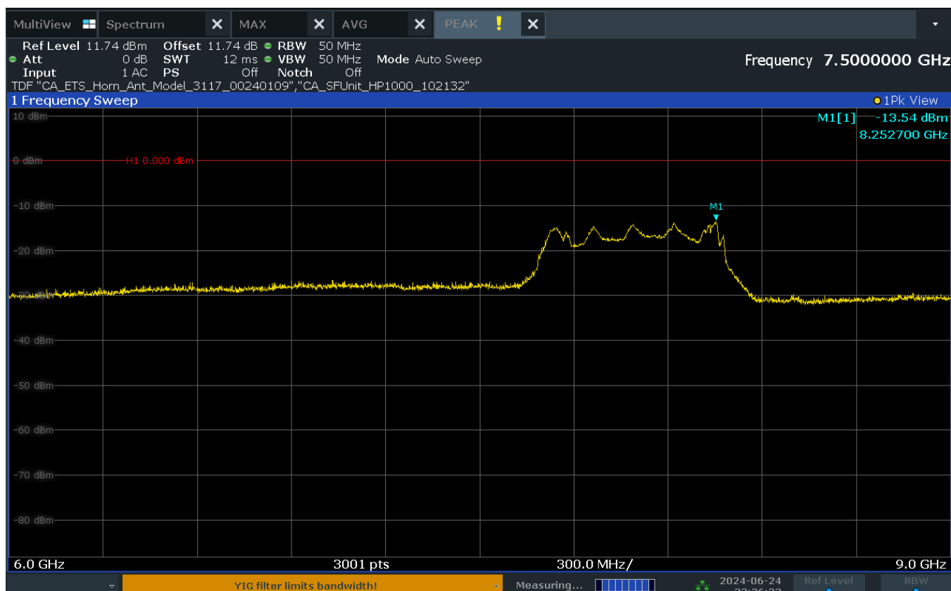
Plot 7-6. Peak Radiated Power (Ch. 9, Config 409/Payload 4093)
