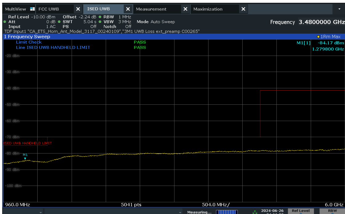
Plot 7-27. ISCED Radiated Spurious Emission 960-6000MHz (Ch. 9, Config 409, Payload 4093 Ant. Pol. H)
