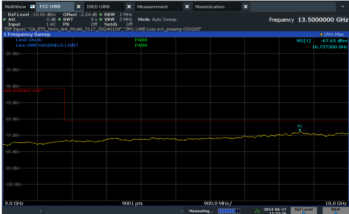
Plot 7-23. Radiated Spurious Emission 9-18GHz (Ch. 5, Config 409, Payload 4093 Ant. Pol. H)
