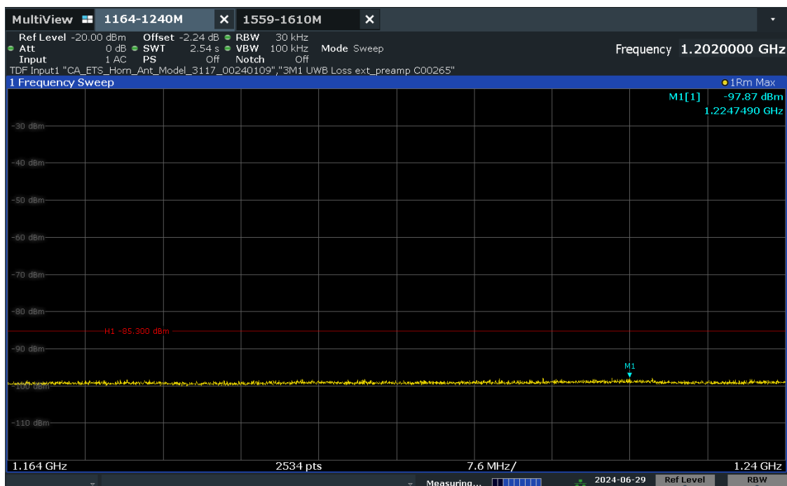
Plot 7-29. Radiated Spurious Emission 1164-1240MHz (Ch. 9, Config 409, Payload 4093 Ant. Pol. H)
