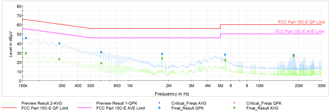
Plot 7-42. AC Line Conducted (Ch. 5, Config 409, Payload 4093 N, with AC/DC Adapter + Magnetic Charger)
