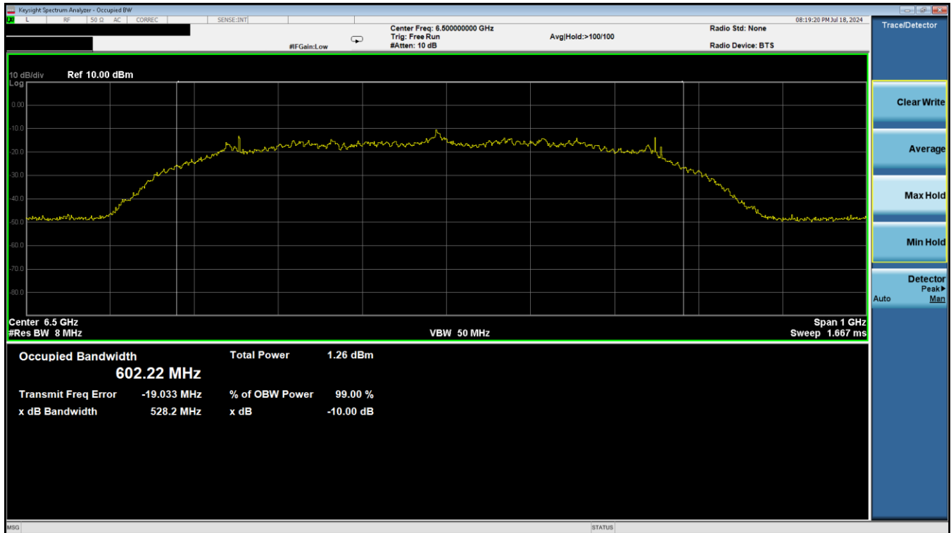
Plot 7-3. ISED 10dBc Occupied Bandwidth & 99% (Ch. 5, Config 409/Payload 4093)
