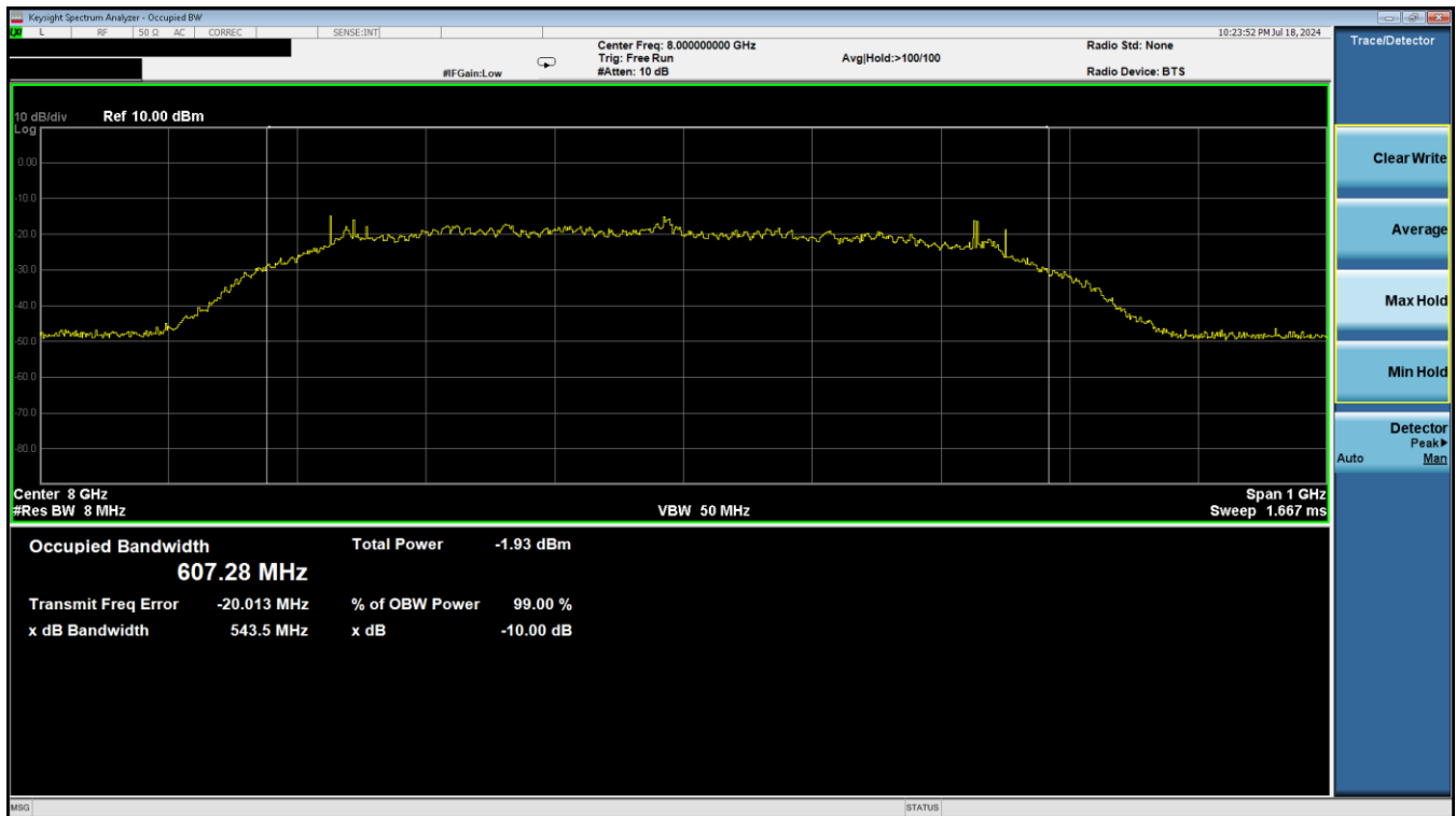
Plot 7-4. ISED 10dBc Occupied Bandwidth & 99 (Ch. 9, Config 409/Payload 4093)
