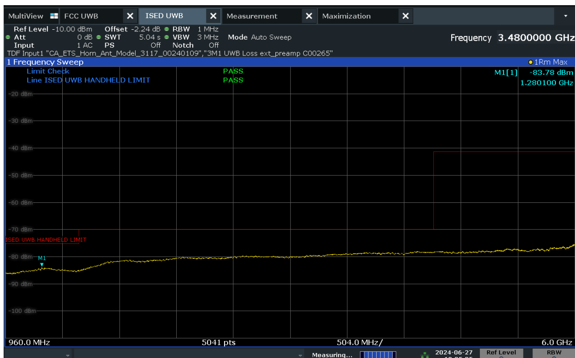
Plot 7-17. ISCED Radiated Spurious Emission 960-6000MHz (Ch. 5, Config 409, Payload 4093 Ant. Pol. H)
