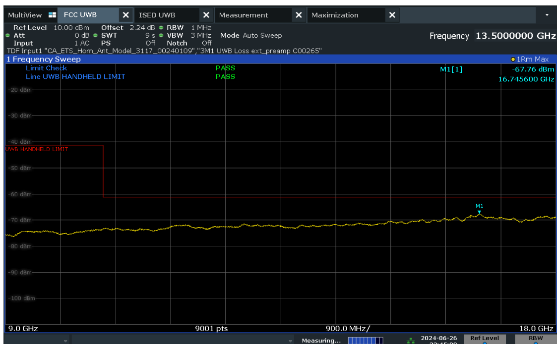
Plot 7-34. Radiated Spurious Emission 9-18GHz (Ch. 9, Config 409, Payload 4093 Ant. Pol. V)
