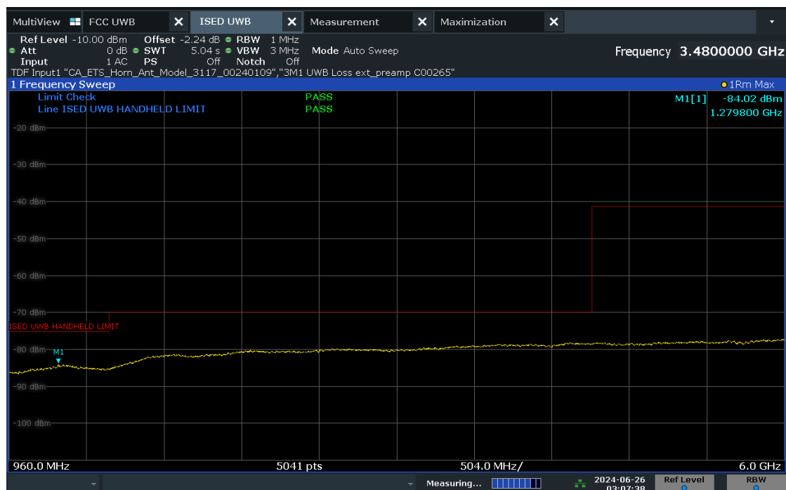
Plot 7-28. ISCED Radiated Spurious Emission 960-6000MHz (Ch.9, Config 409, Payload 4093 Ant. Pol. V)
