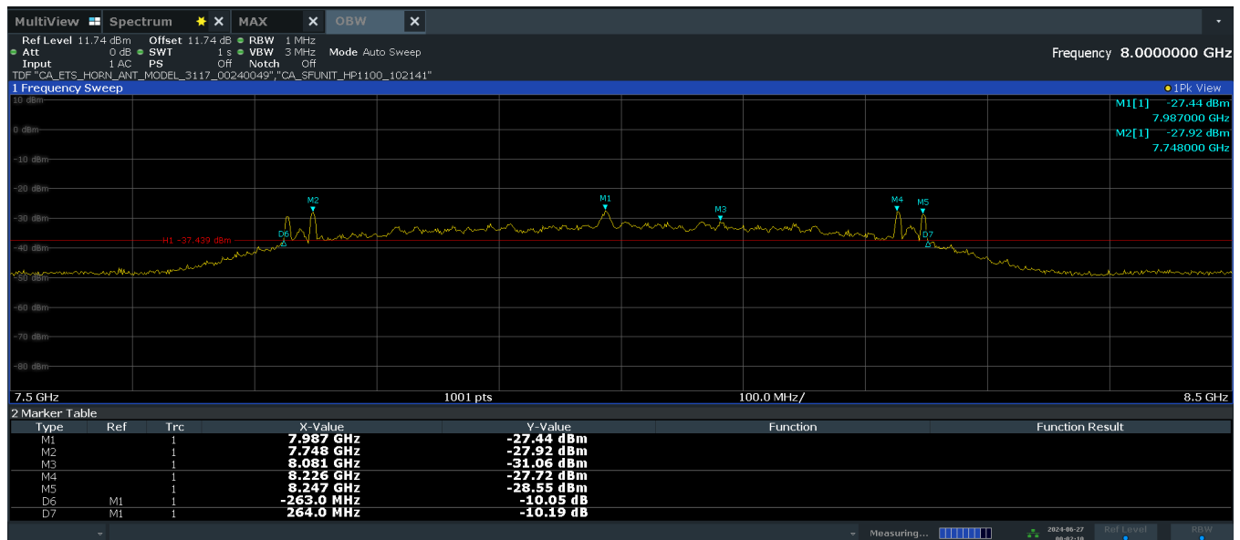
Plot 7-2. 10dBc Bandwidth (Ch. 9, Config 409/Payload 4093)
