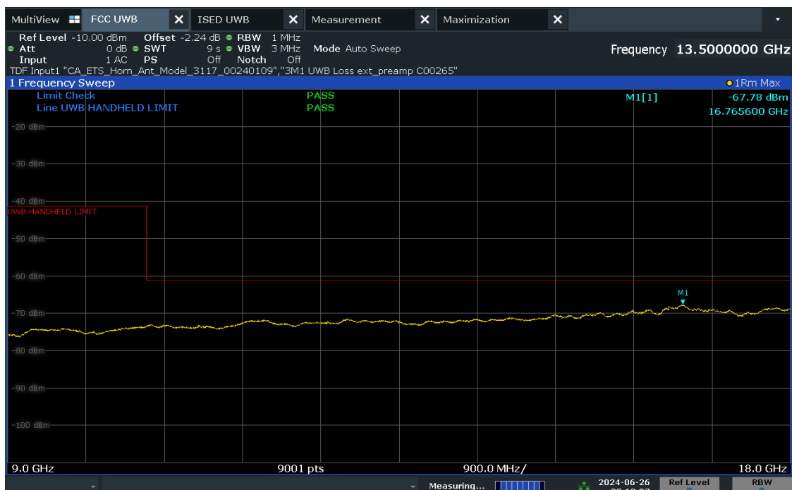
Plot 7-33. Radiated Spurious Emission 9-18GHz (Ch. 9, Config 409, Payload 4093 Ant. Pol. H)
