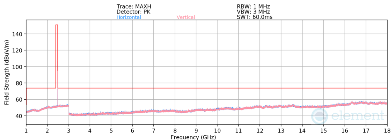
Plot 7-34. Radiated Spurious Emissions above 1GHz (BT GFSK ePA – Ch. 78)
