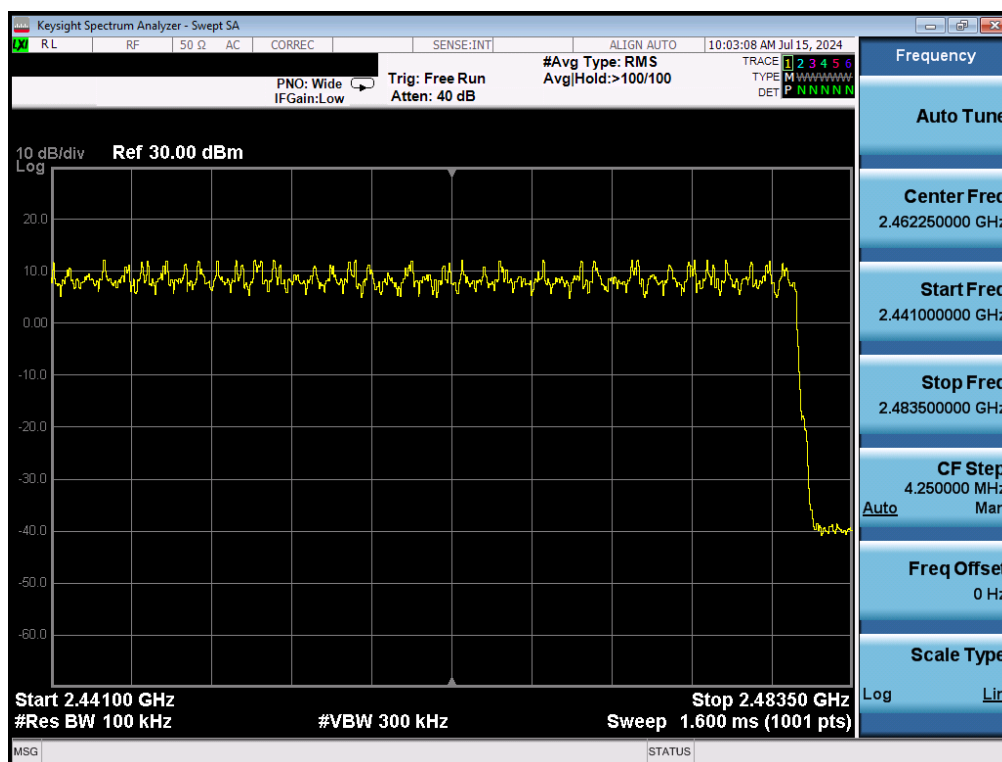
Plot 7-22. High End Spectrum Channel Hopping Plot (Bluetooth, 8DPSK, ePA)
