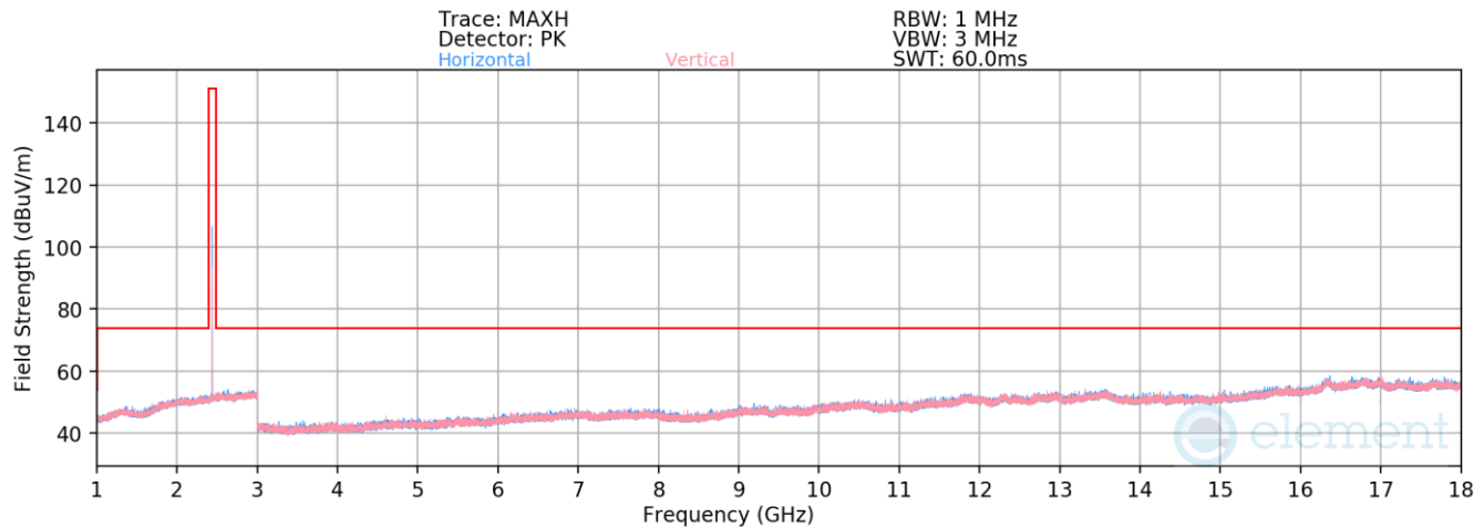
Plot 7-32. Radiated Spurious Emissions above 1GHz (BT GFSK ePA – Ch. 39)
