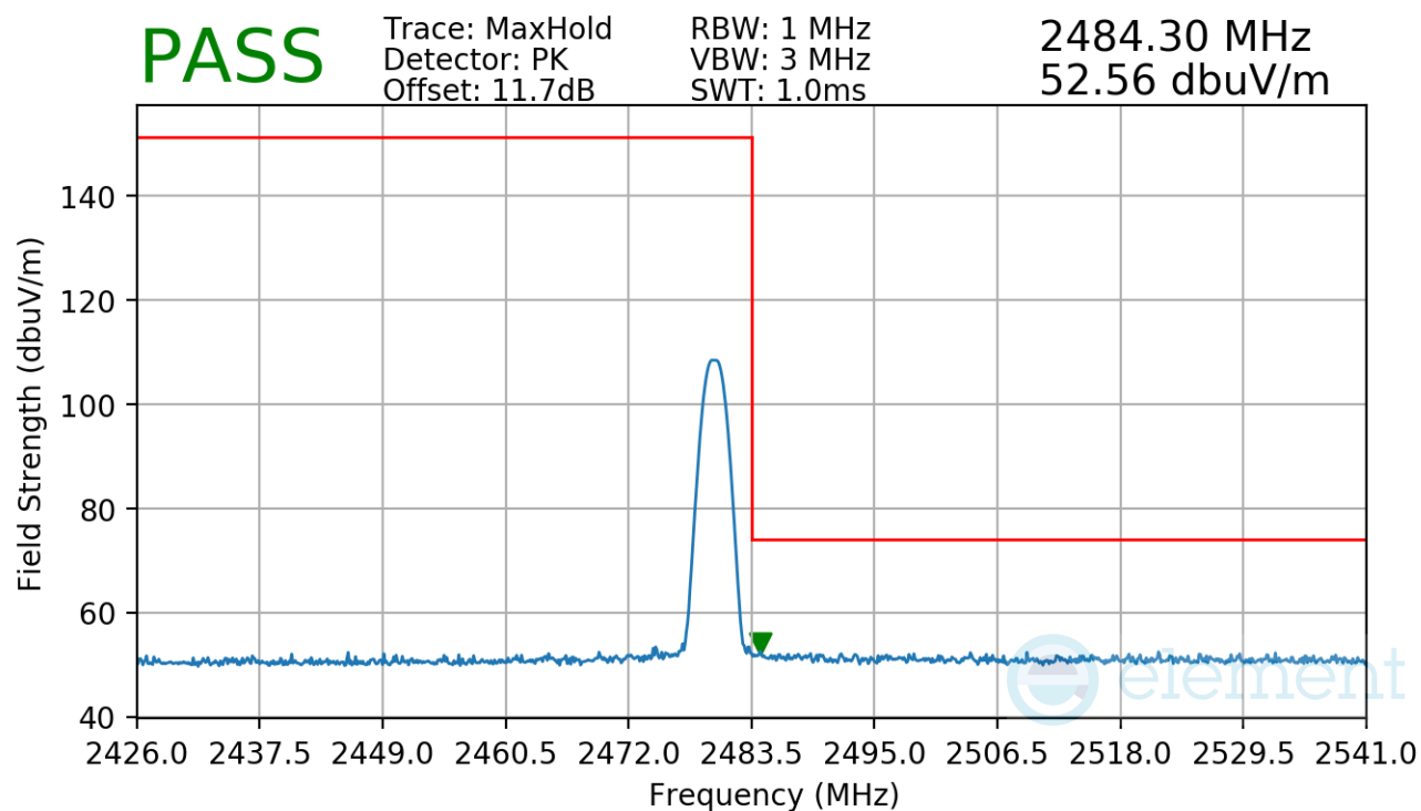
Plot 7-39. Radiated Restricted Upper Band Edge Measurement
