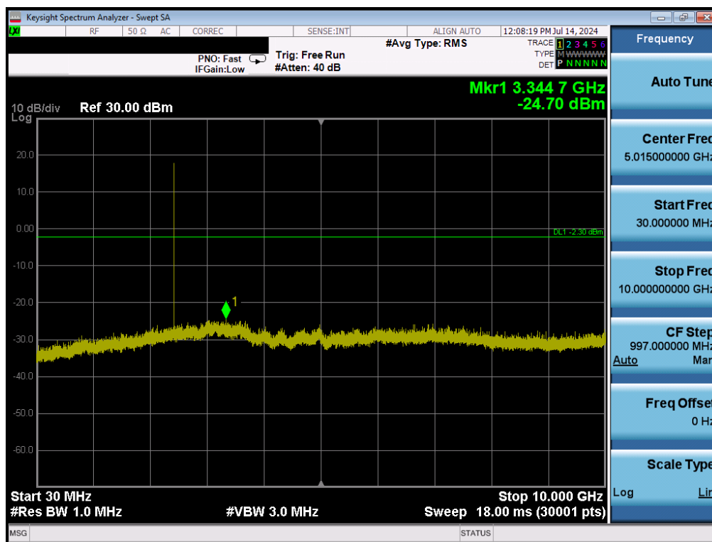
Plot 7-25. Conducted Spurious Plot (Bluetooth, GFSK, ePA – Ch. 39)
