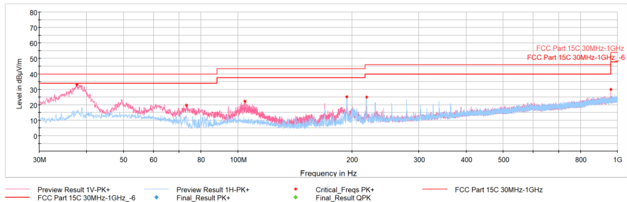
Plot 7-42. Radiated Spurious Emissions Below 1GHz – Simultaneous Transmission
