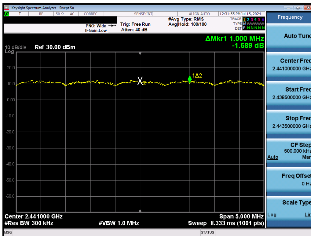
Plot 7-16. Channel Spacing Plot (Bluetooth, 8DPSK, ePA)
