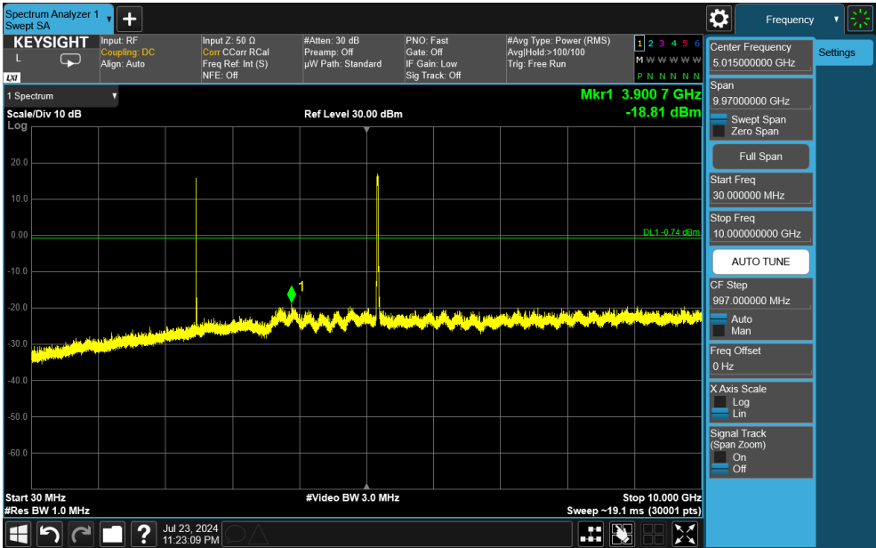
Plot 7-29. Conducted Simultaneous Tx Spurious Plot
