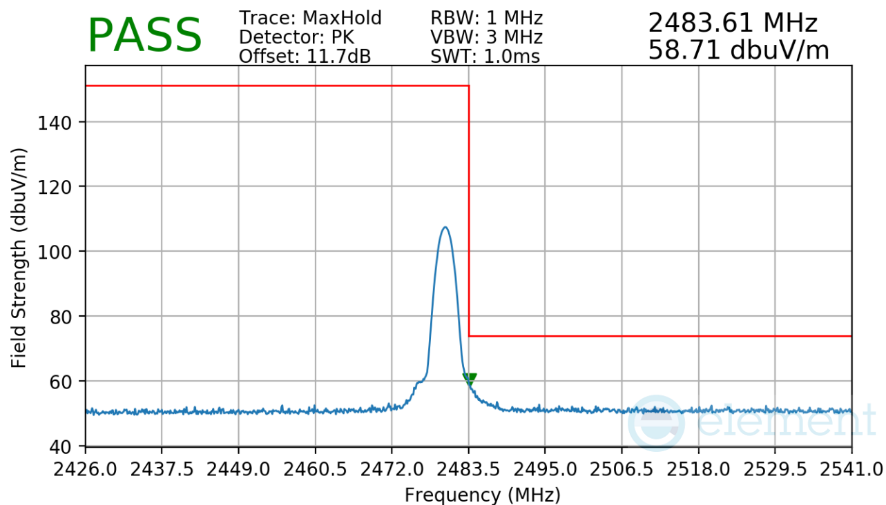
Plot 7-40. Radiated Restricted Upper Band Edge Measurement
