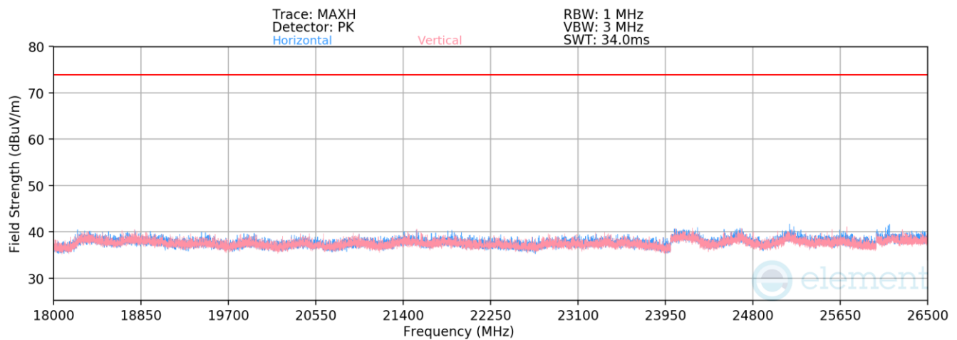
Plot 7-33. Radiated Spurious Emissions above 18GHz (GFSK ePA – Ch.39)
