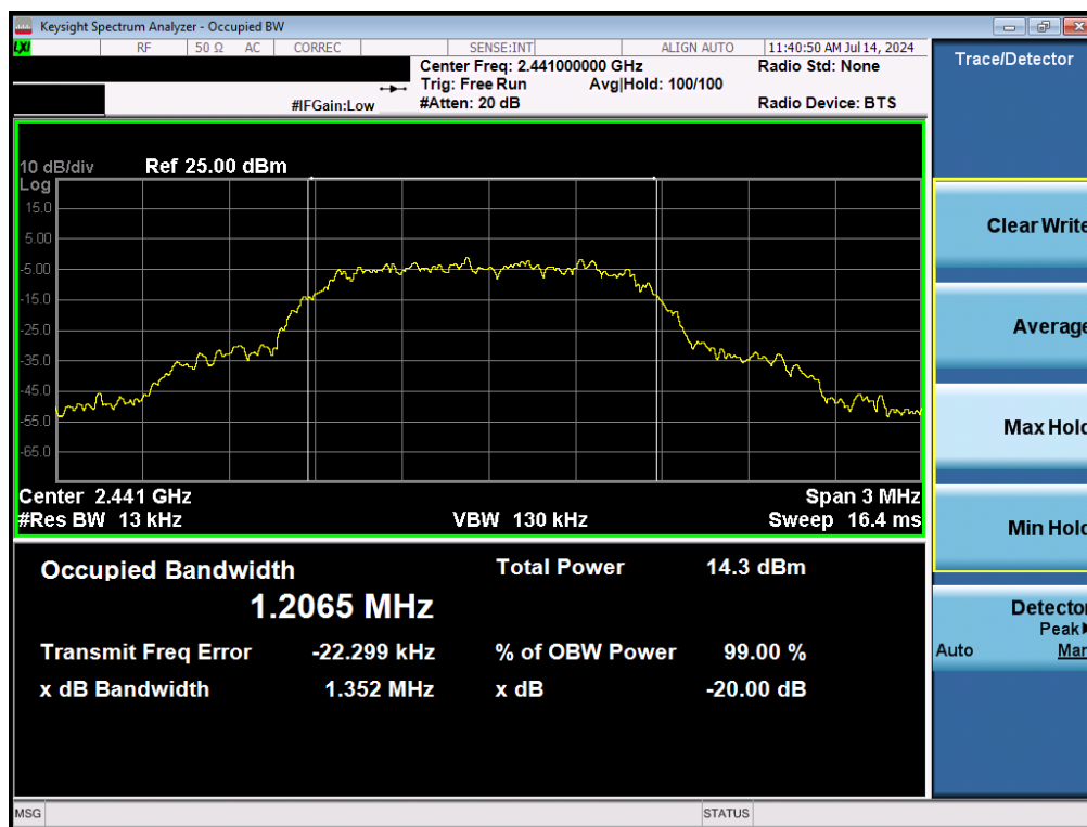
Plot 7-5. 20dB BW and 99% OBW Plot (Bluetooth, 8DPSK, ePA – Ch. 39)
