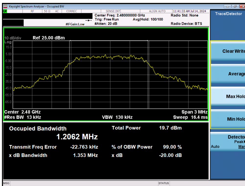
Plot 7-6. 20dB BW and 99% OBW Plot (Bluetooth, 8DPSK, ePA – Ch. 78)
