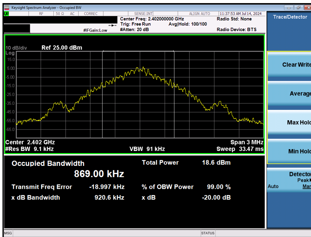
Plot 7-1. 20dB BW and 99% OBW Plot (Bluetooth, GFSK, ePA – Ch. 0)
