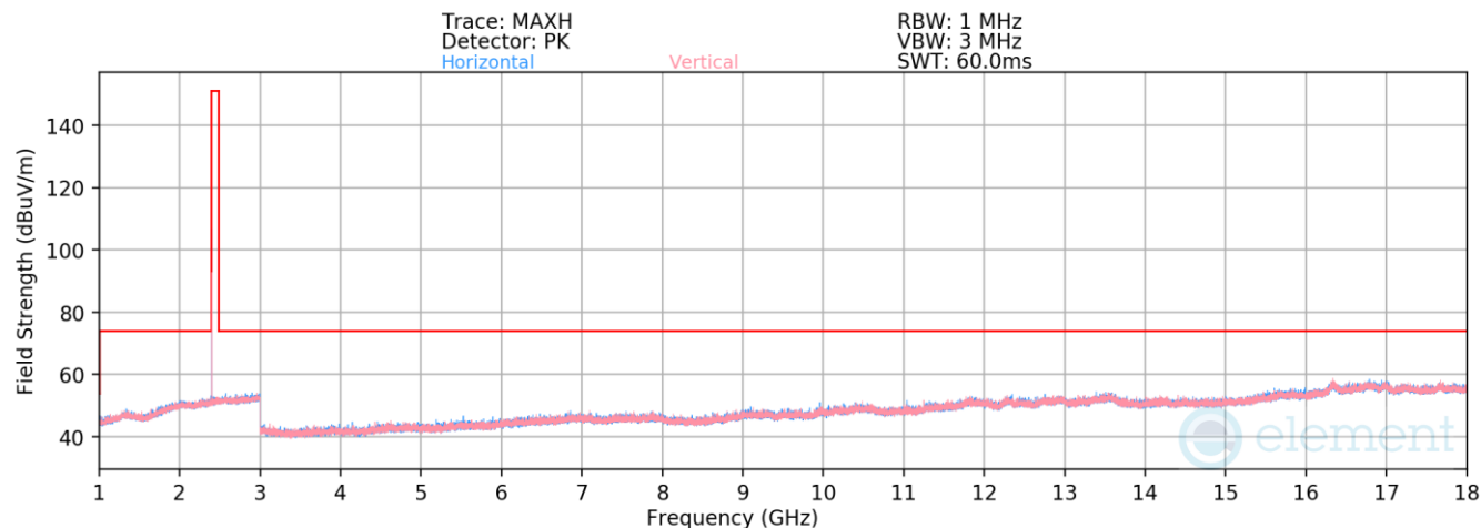
Plot 7-31. Radiated Spurious Emissions above 1GHz (BT GFSK ePA – Ch. 0)
