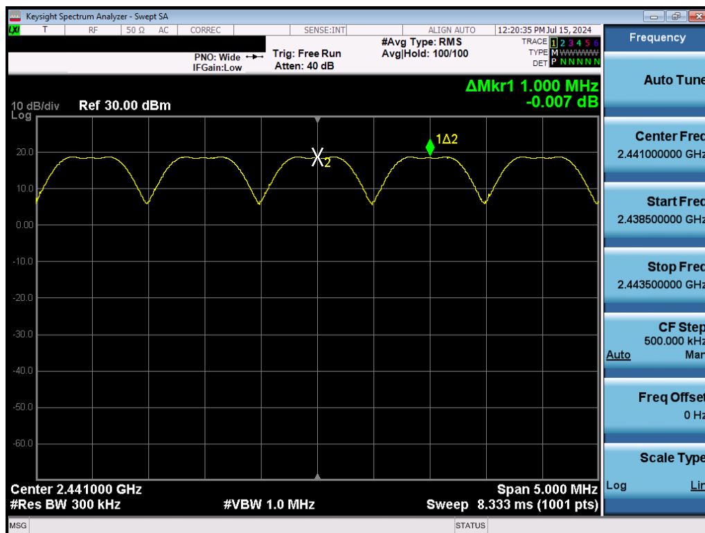
Plot 7-15. Channel Spacing Plot (Bluetooth, GFSK, ePA)
