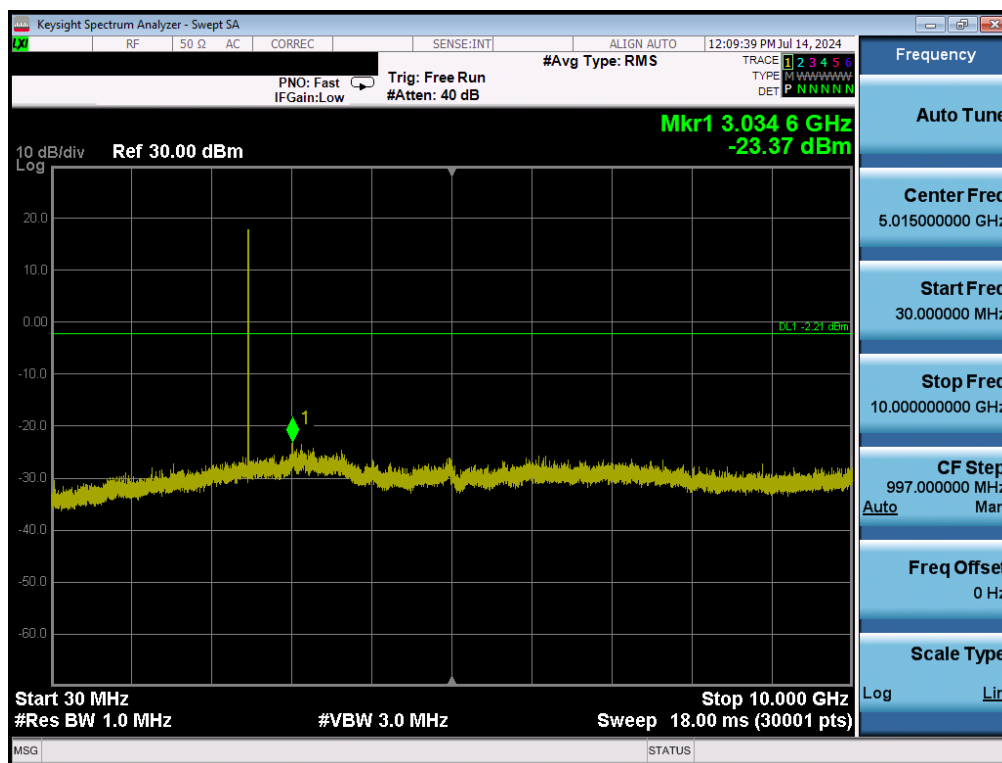
Plot 7-27. Conducted Spurious Plot (Bluetooth, GFSK, ePA – Ch. 78)
