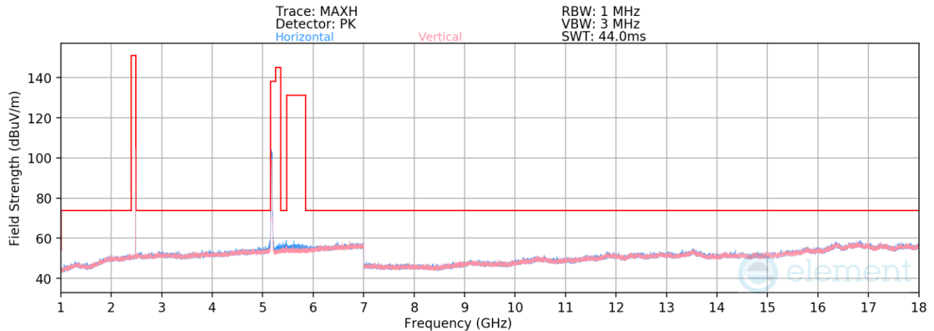
Plot 7-35. Radiated Spurious Emissions 1 - 18GHz – Simultaneous Transmission
