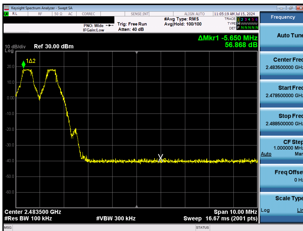
Plot 7-10. Band Edge Plot (Bluetooth with Hopping Enabled, GFSK, ePA)
