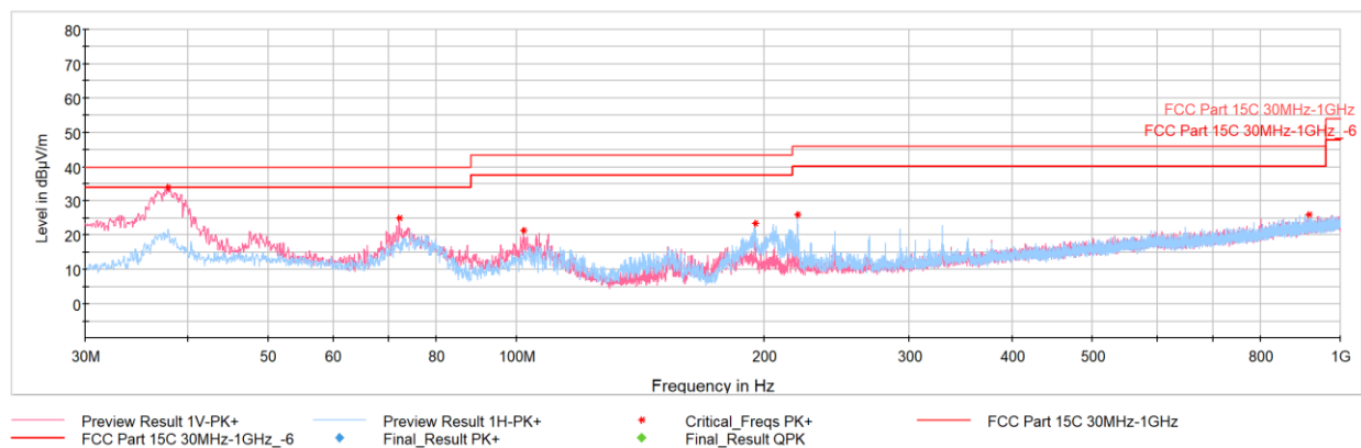
Plot 7-41. Radiated Spurious Emissions Below 1GHz (GFSK ePA – Ch.39, with AC/DC Adapter & Magnetic Charger)
