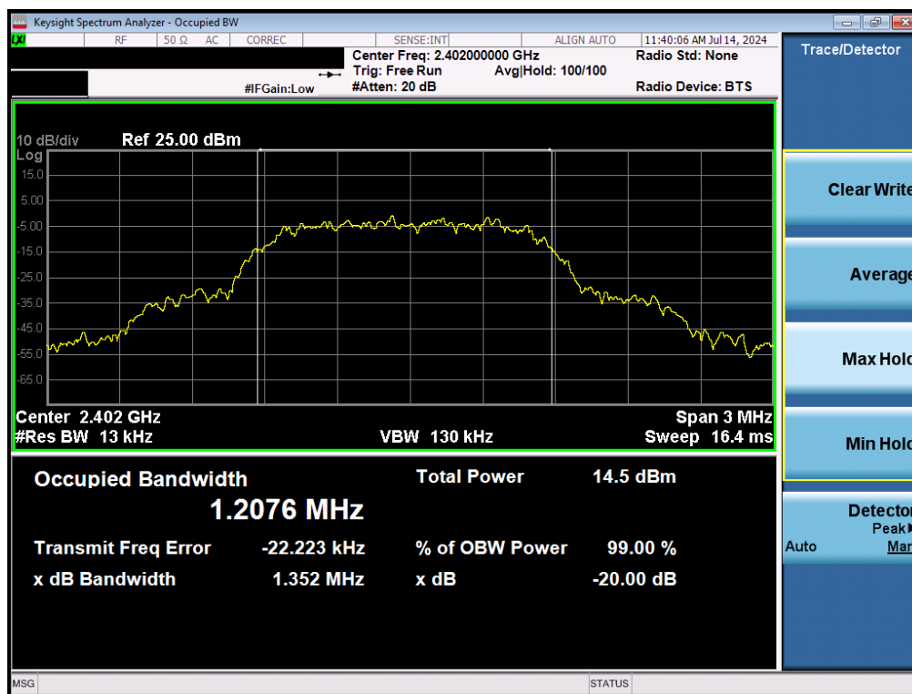
Plot 7-4. 20dB BW and 99% OBW Plot (Bluetooth, 8DPSK, ePA – Ch. 0)
