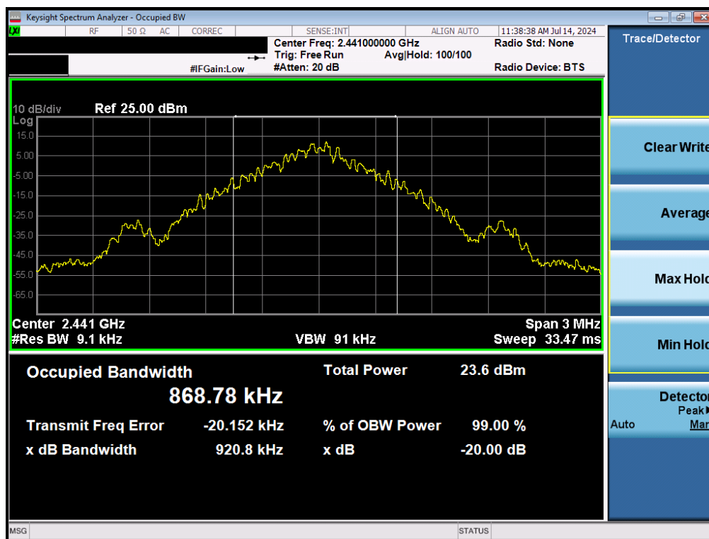
Plot 7-2. 20dB BW and 99% OBW Plot (Bluetooth, GFSK, ePA – Ch. 39)
