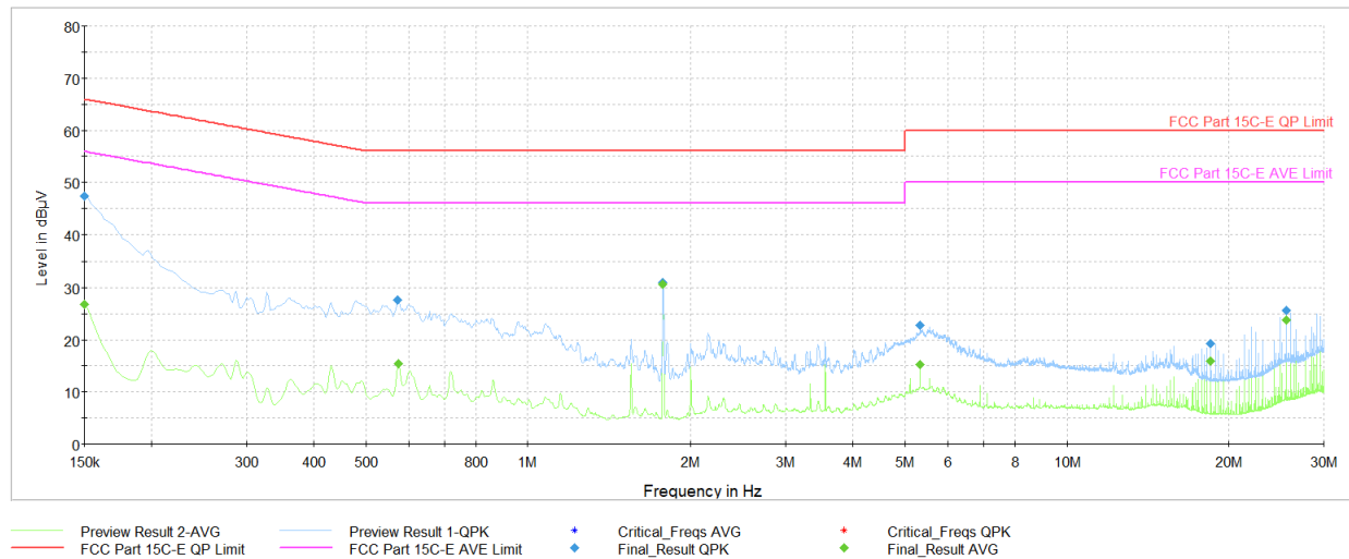
Plot 7-44. AC Line-Conducted Test Plot (N, GFSK ePA – Ch.39, with host PC and Magnetic Charger)
