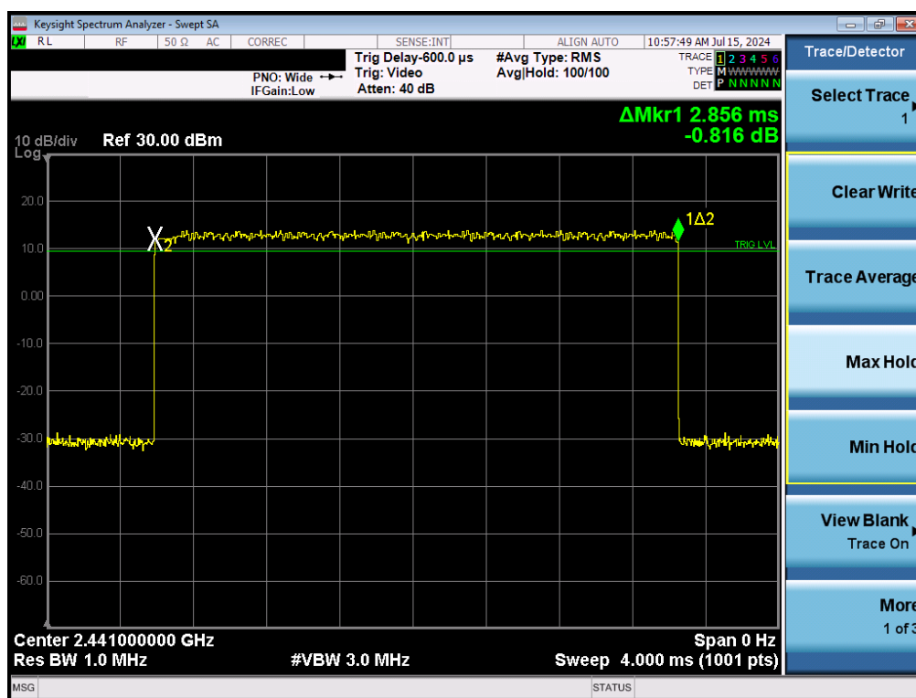
Plot 7-18. Time of Occupancy Plot (Bluetooth, 8DPSK, ePA)
