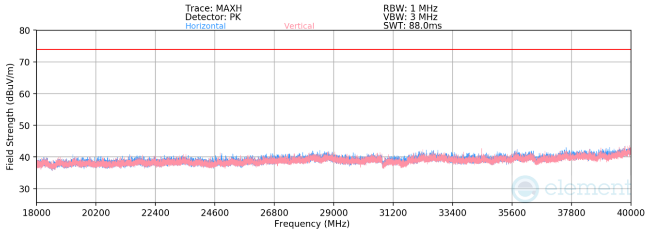
Plot 7-36. Radiated Spurious Emissions above 18GHz Simultaneous Transmission (Pol. H & V)
