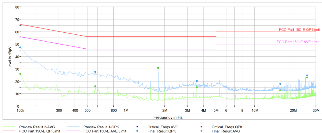
Plot 7-43. AC Line-Conducted Test Plot (L1, GFSK ePA – Ch.39, with host PC and Magnetic Charger)
