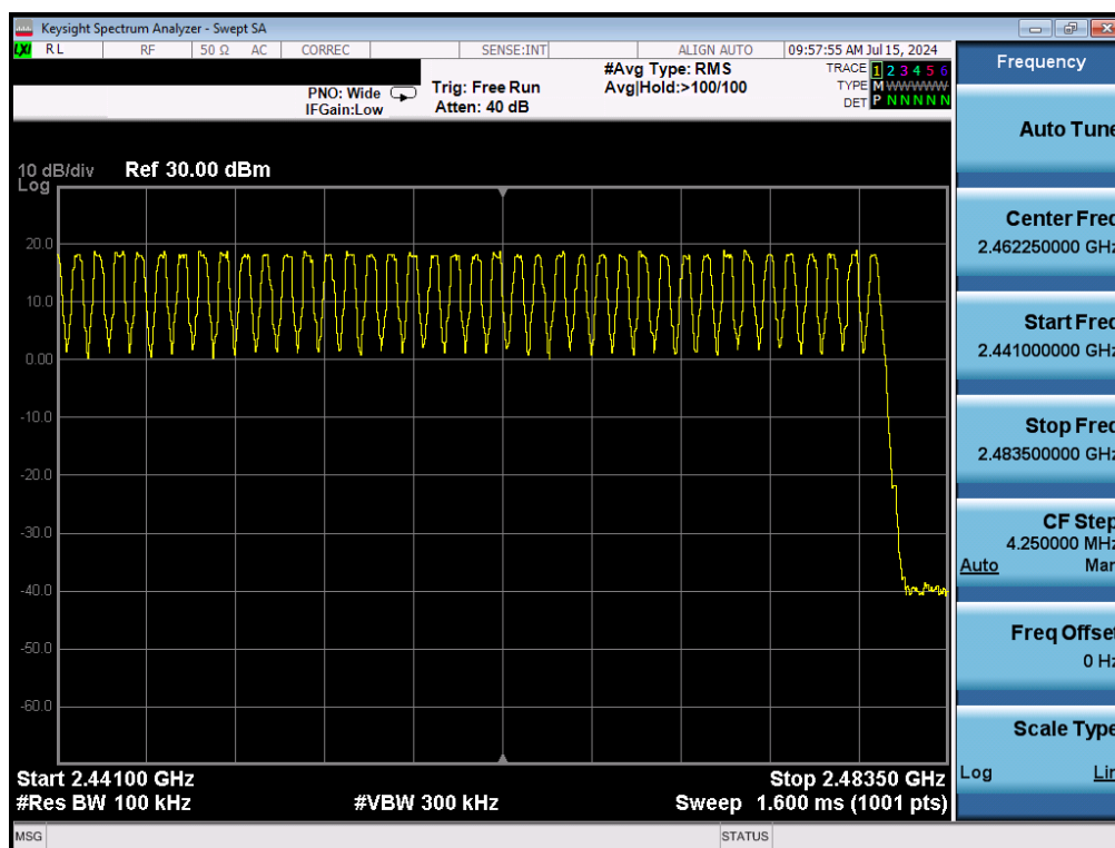
Plot 7-20. High End Spectrum Channel Hopping Plot (Bluetooth, GFSK, ePA)
