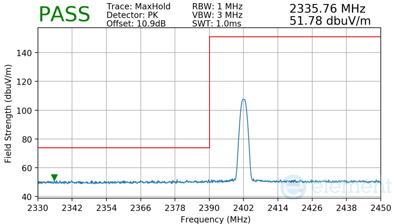
Plot 7-37. Radiated Restricted Lower Band Edge Measurement
