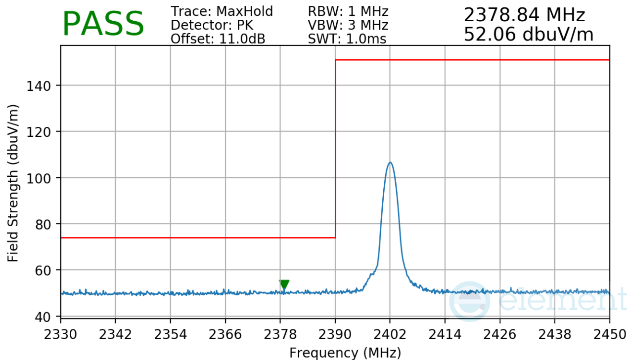
Plot 7-38. Radiated Restricted Lower Band Edge Measurement
