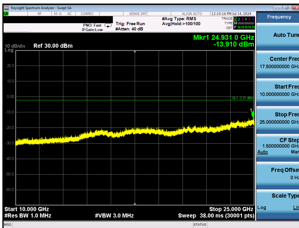
Plot 7-28. Conducted Spurious Plot (Bluetooth, GFSK, ePA – Ch. 78)
