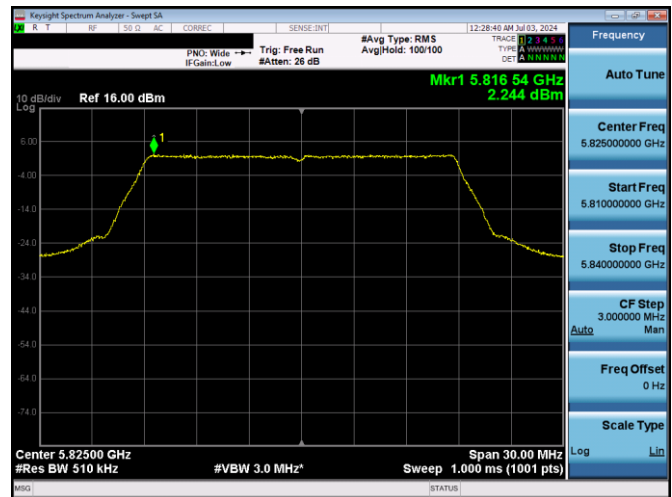
Plot 7-27. PSD (20MHz BW 802.11n – Ch. 165, MCS0)
