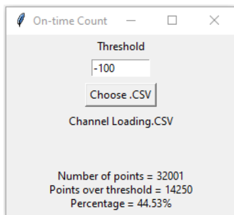
Figure 9-2. 5500MHz - Channel Loading Calculation - (20MHz)
