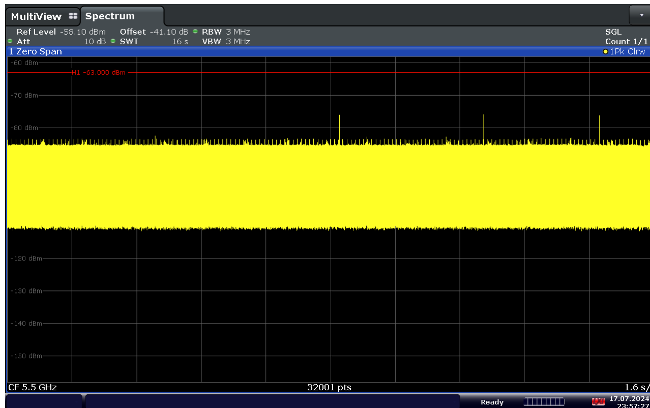
Figure 9-1. 5500MHz - Channel Loading - (20MHz)
