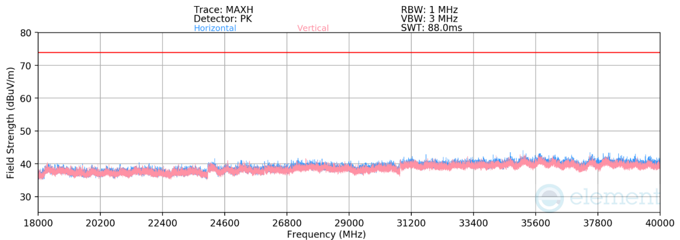
Plot 7-39. Radiated Emissions 18GHz-40GHz (802.11n – Ch. 157)
