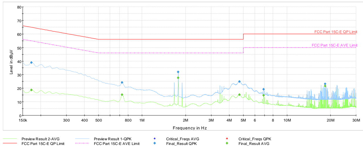
Plot 7-59. AC Line Conducted Plot with 802.11n Ch.157 (L1), with AC/DC adapter & magnetic charger
