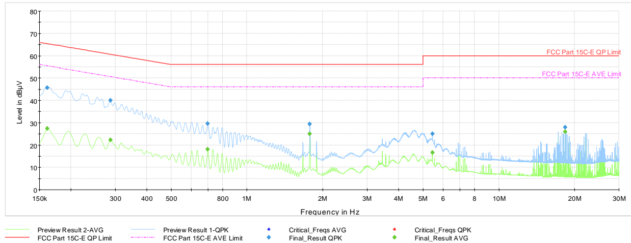
Plot 7-60. AC Line Conducted Plot with 802.11n Ch.157 (N), with AC/DC & magnetic charger
