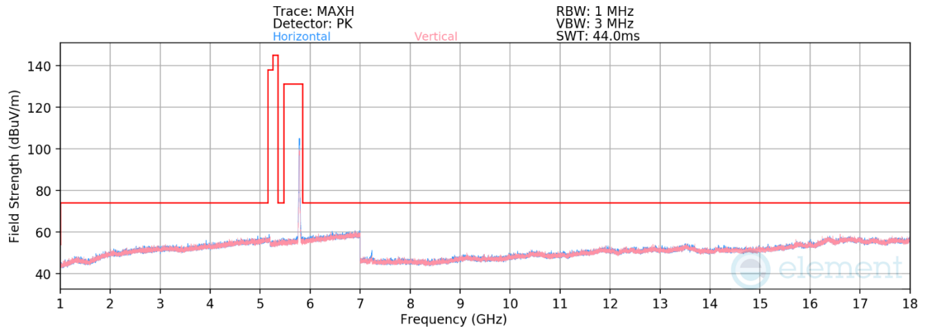
Plot 7-38. Radiated Spurious Emissions above 1GHz(802.11n – Ch. 157)
