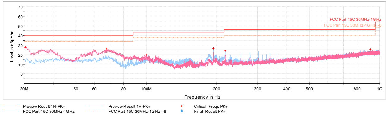
Plot 7-57. Radiated Spurious Emissions below 1GHz, 802.11n, Ch. 157 with AC/DC Adapter & magnetic charger
