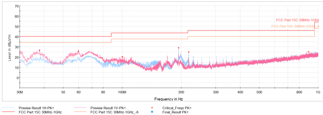
Plot 7-37. Radiated Spurious Emissions Below 1GHz (1Mbps, ePA – Ch.19, Pol. H & V, with AC/DC Adapter + Magnetic Charger)
