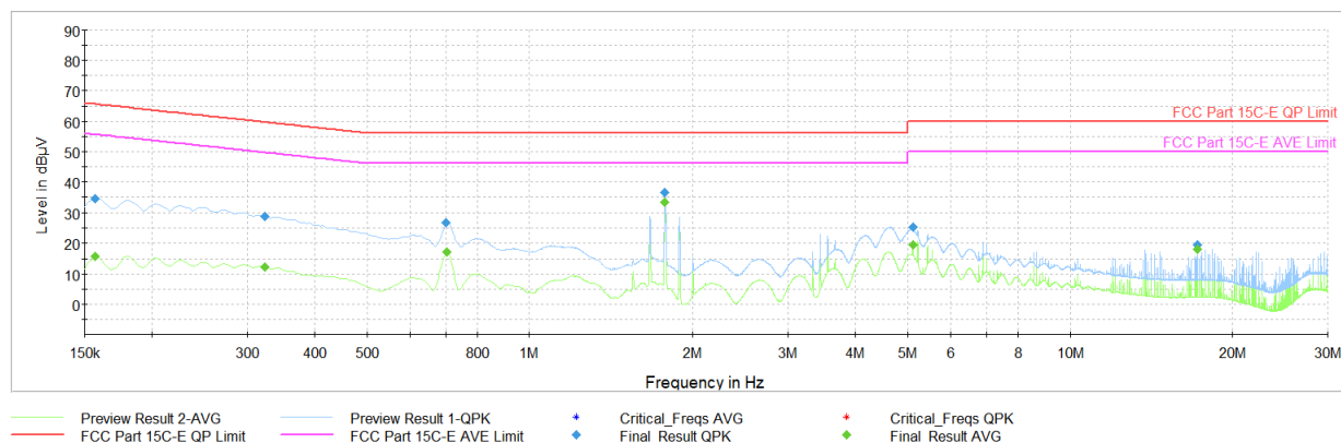
Plot 7-39. AC Line Conducted Plot with Bluetooth LE (N, 1Mbps ePA – Ch.19, with AC/DC Adapter + Magnetic Charger)
