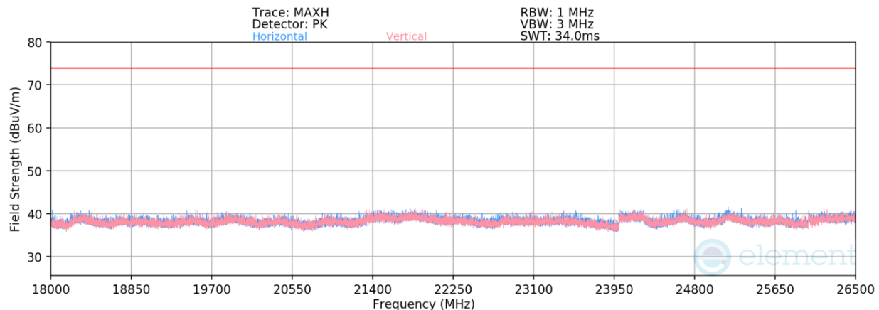
Plot 7-36. Radiated Spurious Emissions above 18GHz Simultaneous Transmission
