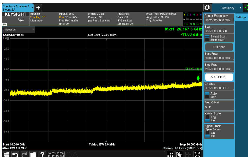
Plot 7-30. Conducted Simultaneous Tx Spurious Plot
