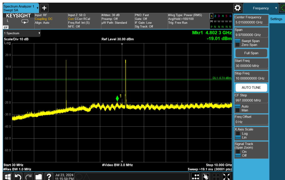
Plot 7-29. Conducted Simultaneous Tx Spurious Plot
