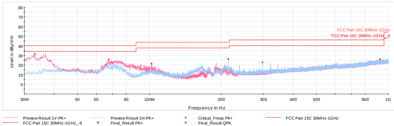
Plot 7-41. Radiated Spurious Emissions Below 1GHz (GFSK ePA – Ch.39, with AC/DC Adapter & Magnetic Charger)
