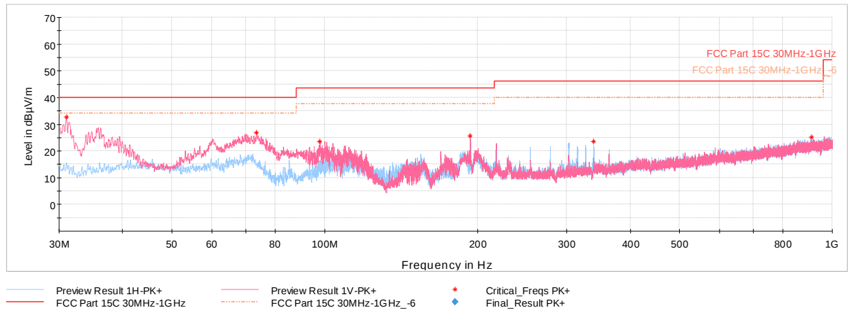
Plot 7-42. Radiated Spurious Emissions Below 1GHz – Simultaneous Transmission
