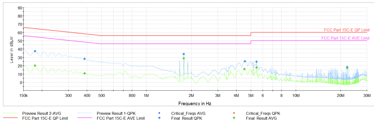
Plot 7-43. AC Line-Conducted Test Plot (L1, GFSK ePA – Ch.39, with AC/DC Adapter + Magnetic Charger)
