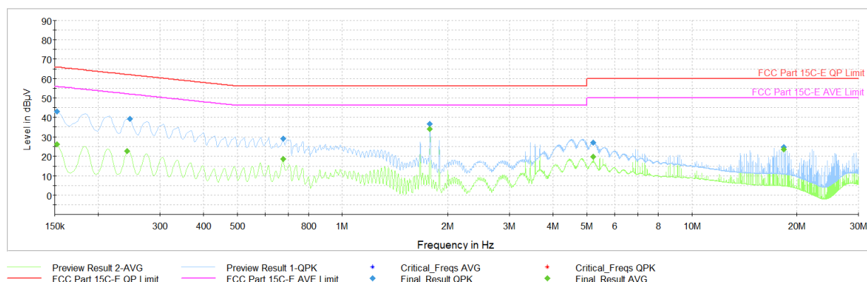
Plot 7-44. AC Line-Conducted Test Plot (N, GFSK ePA – Ch.39, with AC/DC Adapter + Magnetic Charger)
