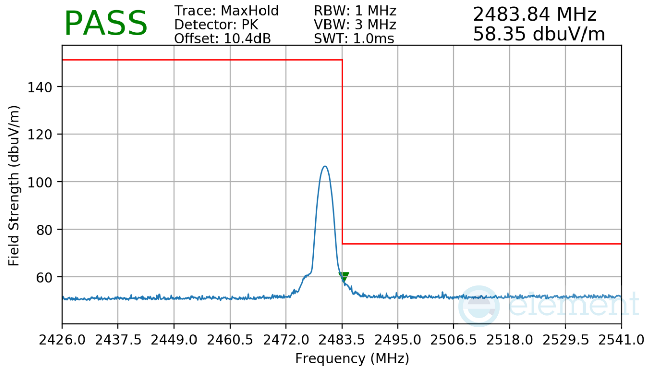
Plot 7-40. Radiated Restricted Upper Band Edge Measurement
