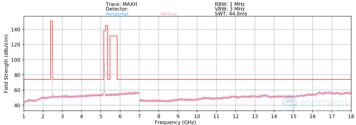
Plot 7-35. Radiated Spurious Emissions 1 - 18GHz – Simultaneous Transmission
