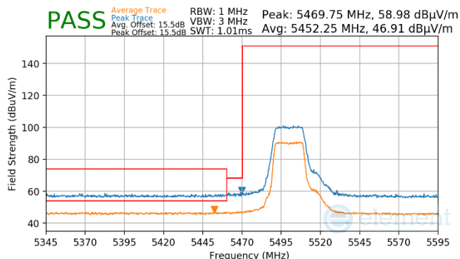
Plot 7-49. (Pk & Avg, Ch.100, 802.11n, MCS0)
