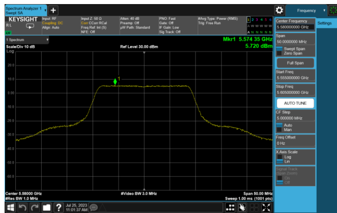
Plot 7-20. PSD (20MHz BW 802.11n - Ch. 116, MCS0)
