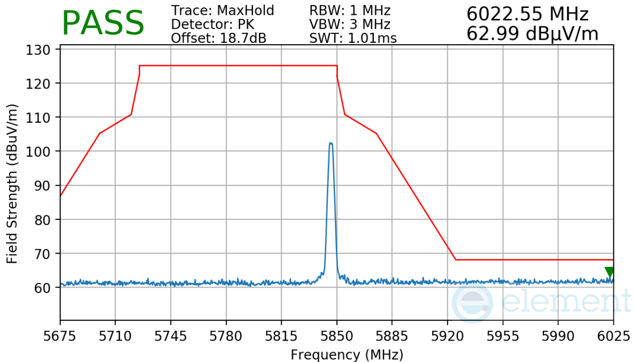
Plot 7-25. Radiated Upper Band Edge Measurement (Pk, Ch. 48, QPSK, 250Kbps)
