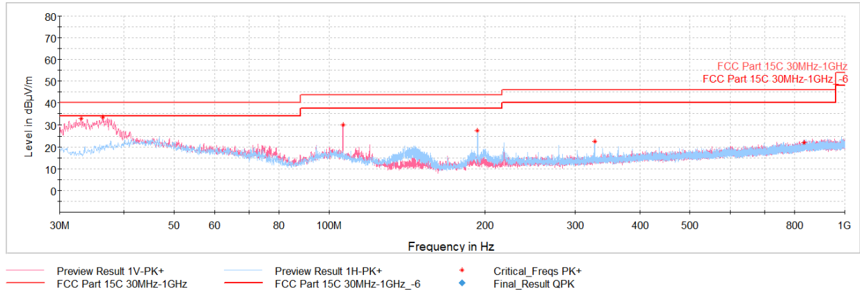
Plot 7-30. RSE 30MHz - 1GHz (OQPSK - Ch. 24), with Laptop & Magnetic charger
