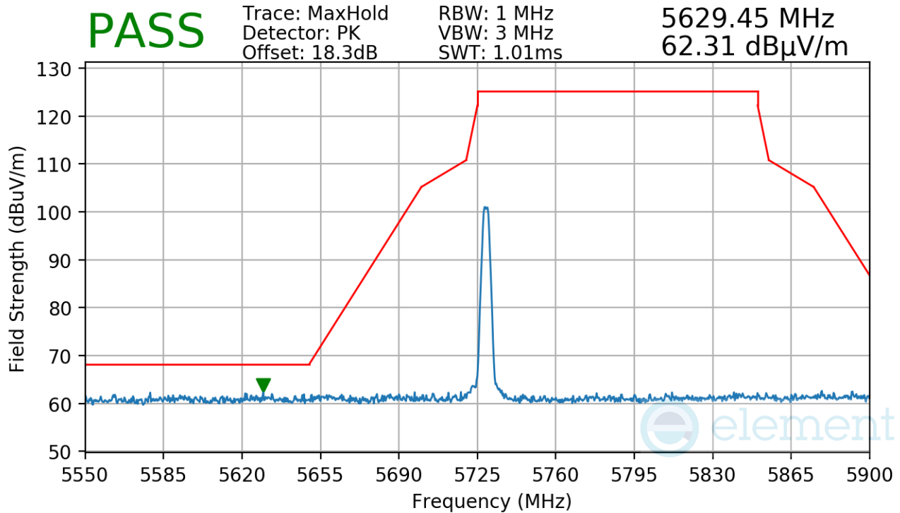
Plot 7-24. Radiated Lower Band Edge Measurement (Pk, Ch. 1, QPSK, 250Kbps)
