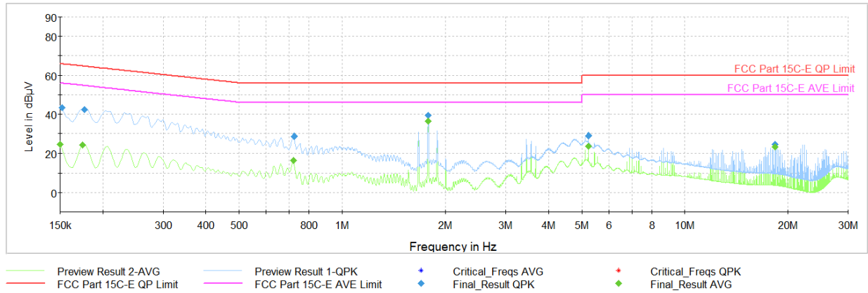
Plot 7-32. AC Line Conducted Plot (OQPSK – Ch. 24) (N) with AC/DC Adapter & Magnetic charger
