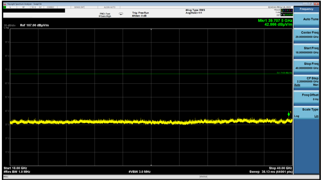
Plot 7-22. Radiated Spurious Emissions Above 18GHz (OQPSK – 5786.25MHz Pol H)
