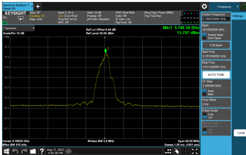
Plot 7-17. PSD (QPSK, 5786.25MHz, 1000kbps)
