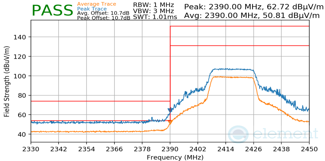
Plot 7-69. Radiated Restricted Lower Band Edge Measurement
