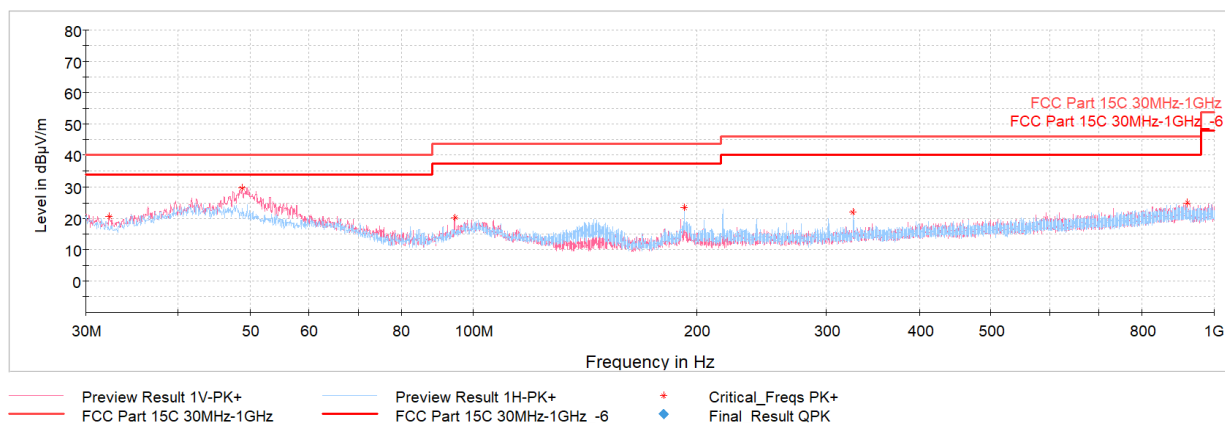
Plot 7-38. Radiated Spurious Emissions Below 1GHz (1Mbps, ePA – Ch.39, Pol. H & V, with AC/DC Adapter + Magnetic Charger)
