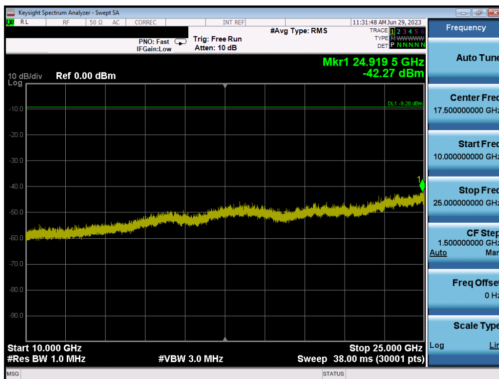
Plot 7-24. Conducted Spurious Plot (Bluetooth (HDR4), 4 Mbps, ePA – Ch. 1)
