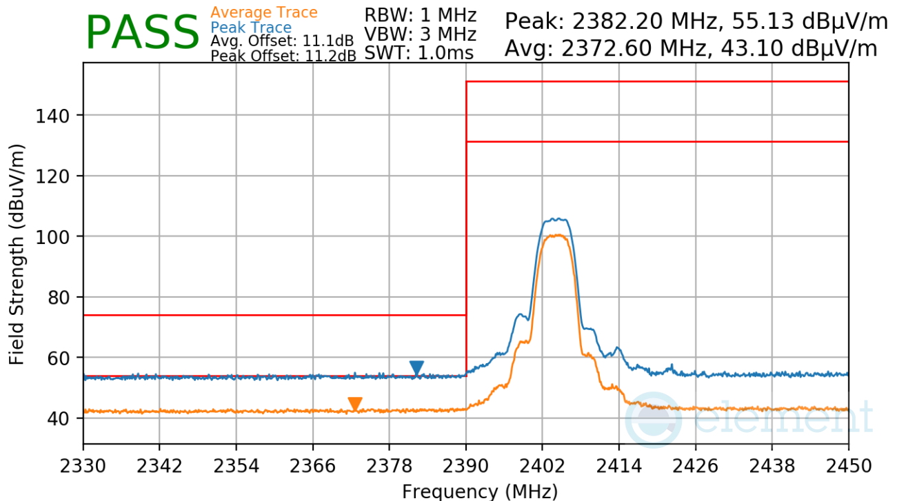
Plot 7-35. Radiated Restricted Lower Band Edge Measurement
