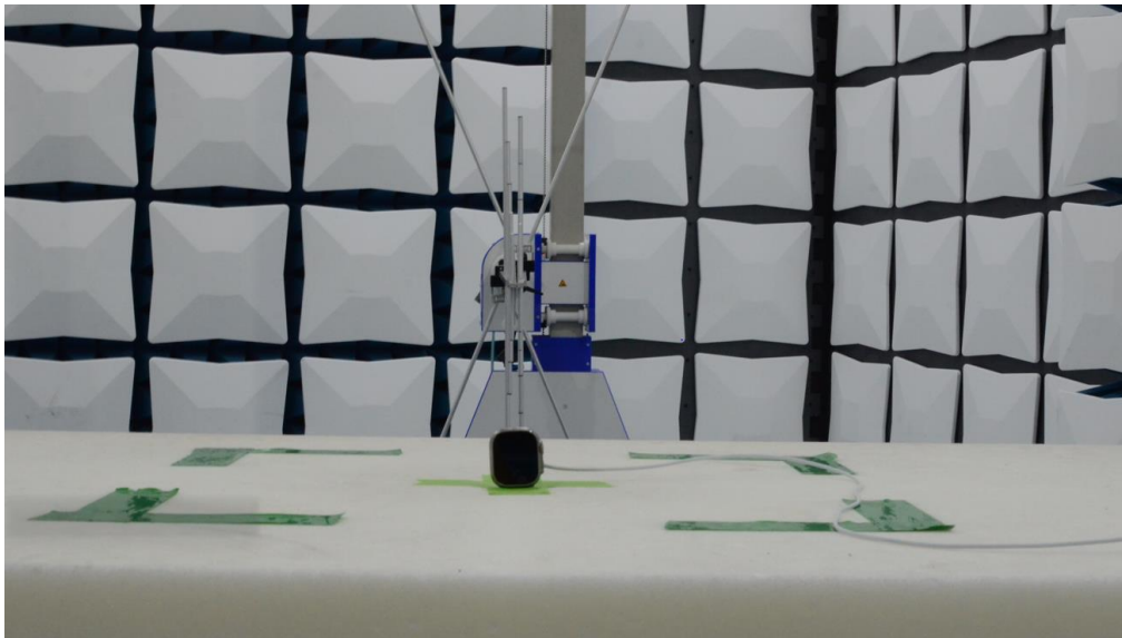
Figure 16: 30MHz-1GHz Test Setup (Rear View)
