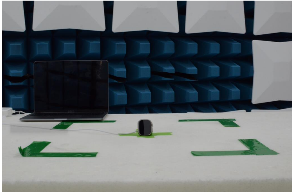
Figure 21: 30MHz-1GHz Test Setup (Front View)
