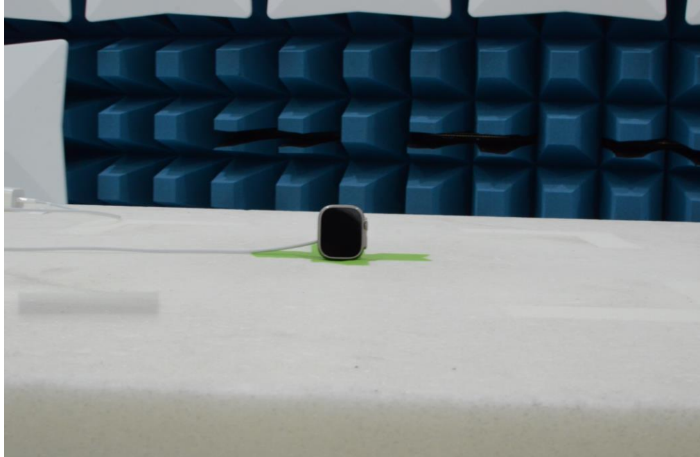
Figure 9: 1-18GHz Test Setup (Front View)
