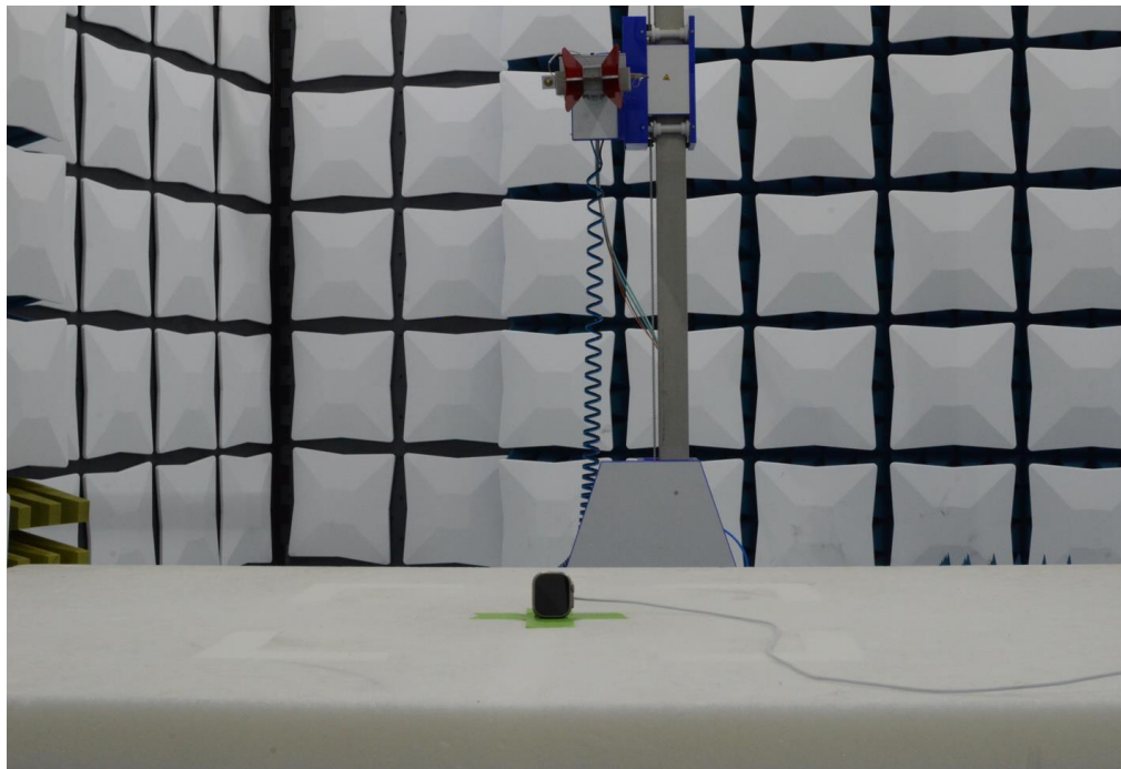
Figure 10: 1-18GHz Test Setup (Rear View)
