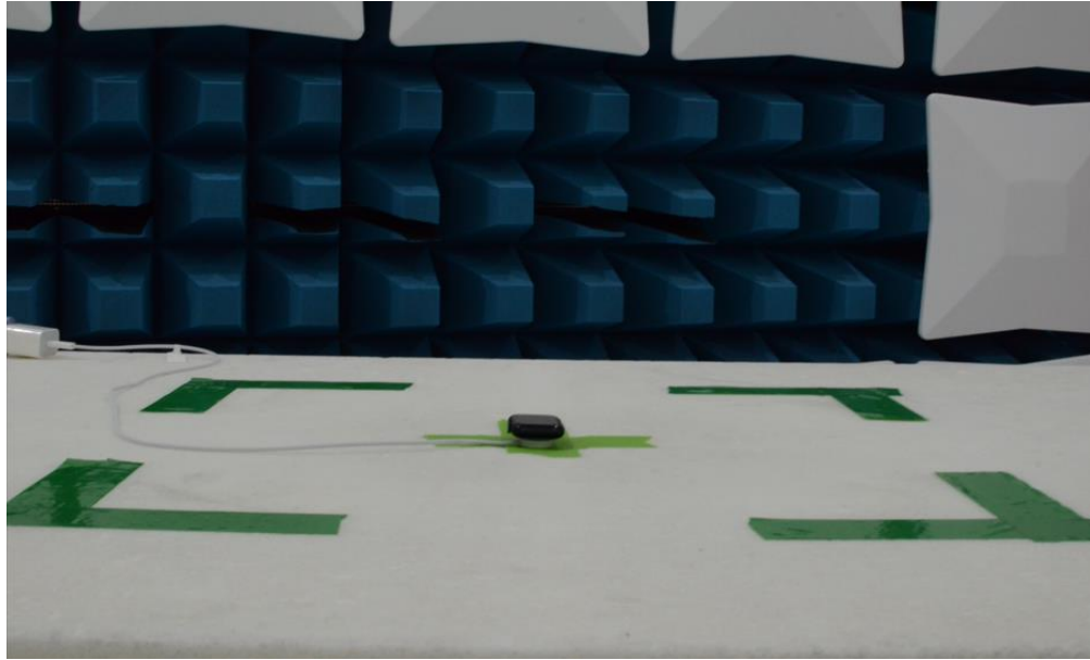
Figure 11: 30MHz-1GHz Test Setup (Front View)
