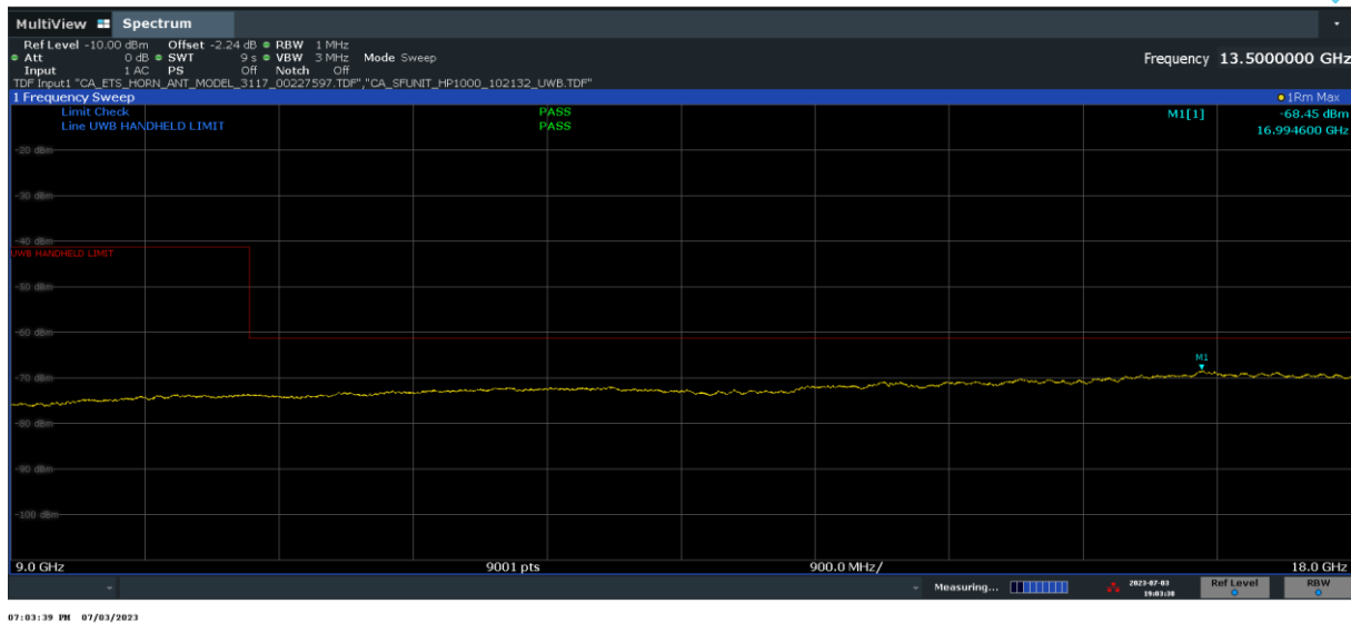
Plot 7-33. Radiated Spurious Emission 9-18GHz (Ch. 9, Config 409, Payload 4093 Ant. Pol. H)
