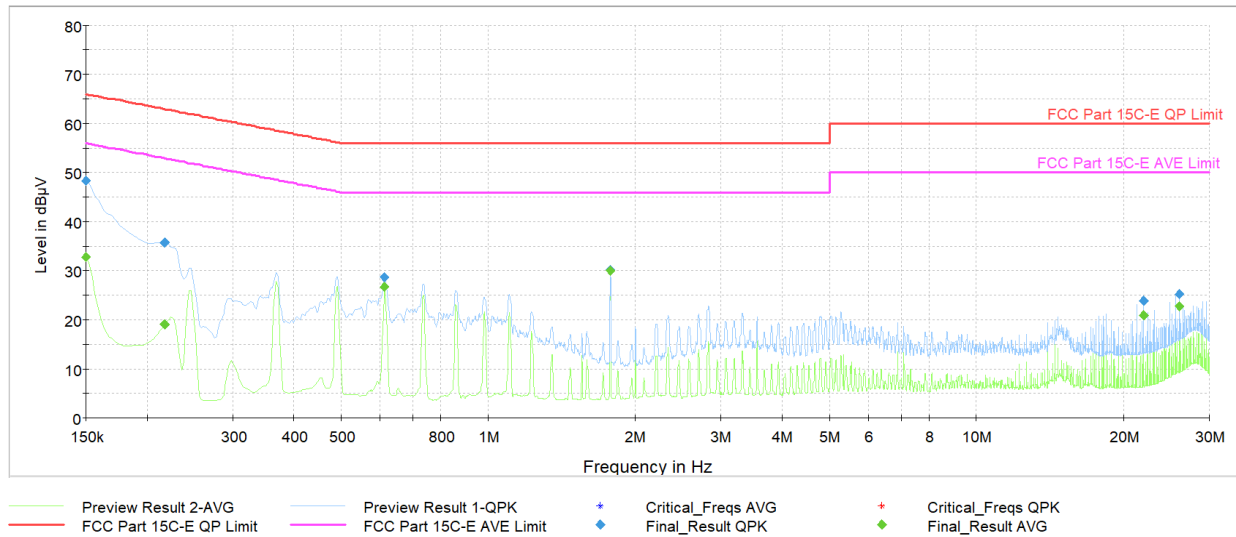
Plot 7-41. AC Line Conducted (Ch. 5, Config 409, Payload 4093 L1, with PC via USB-C cable with magnetic charger)
