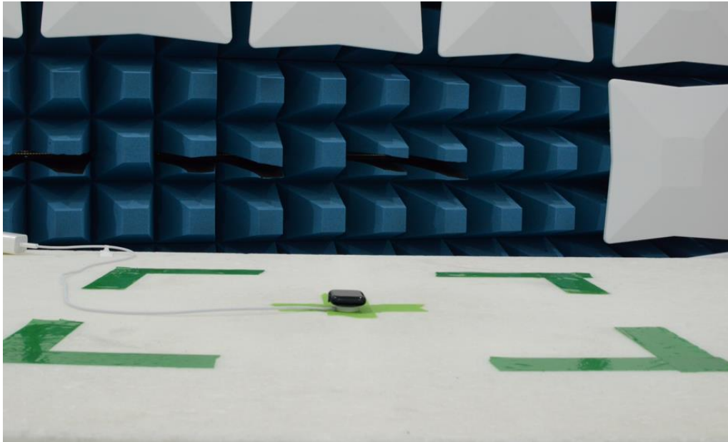
Figure 1: 1-18GHz Test Setup (Front View)
