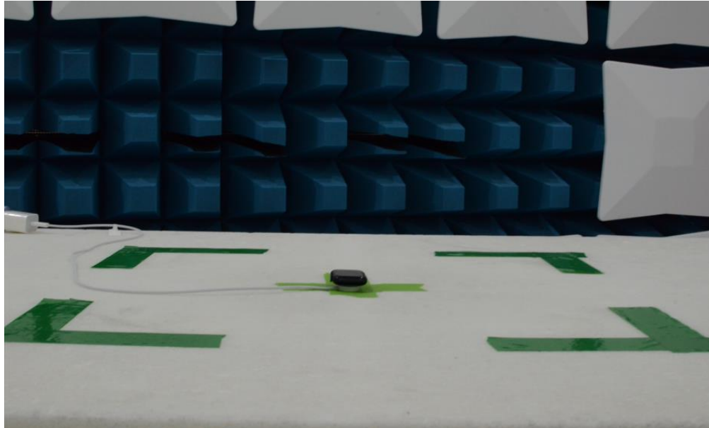
Figure 7: 30MHz-1GHz Test Setup (Front View)
