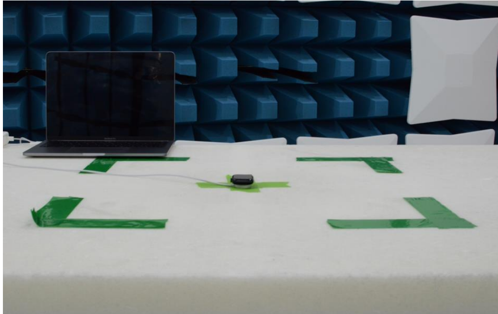
Figure 13: 30MHz-1GHz Test Setup (Front View)
