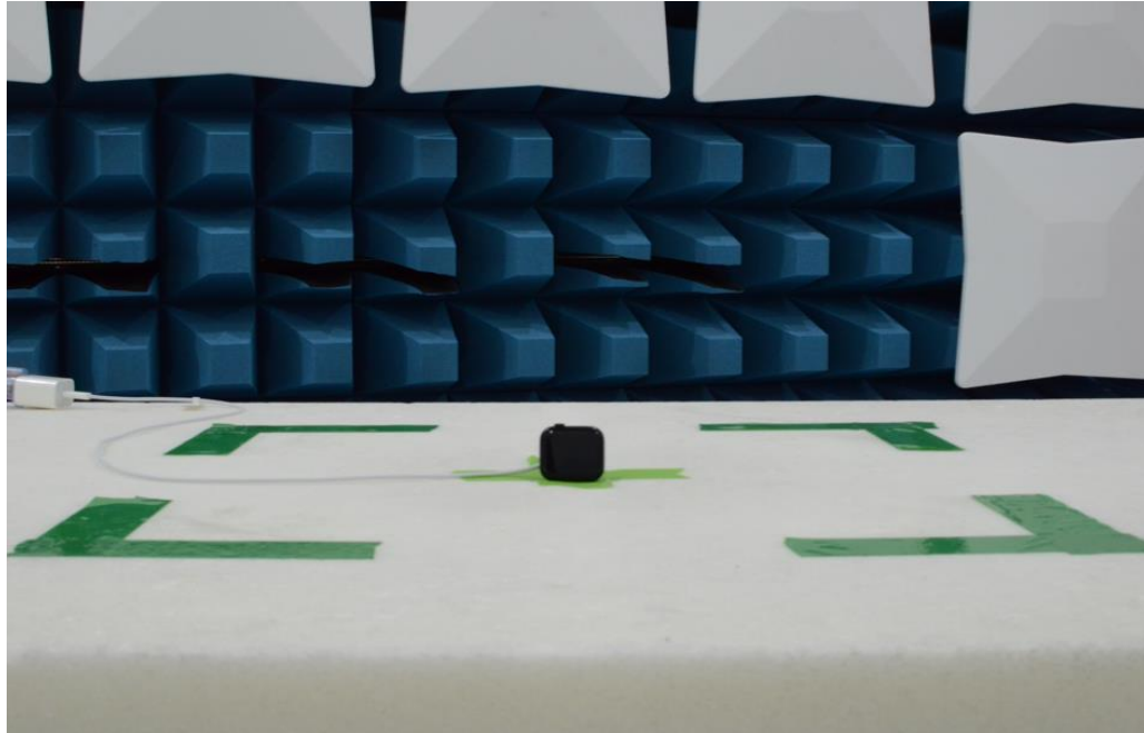
Figure 3: 1-18GHz Test Setup (Front View)
