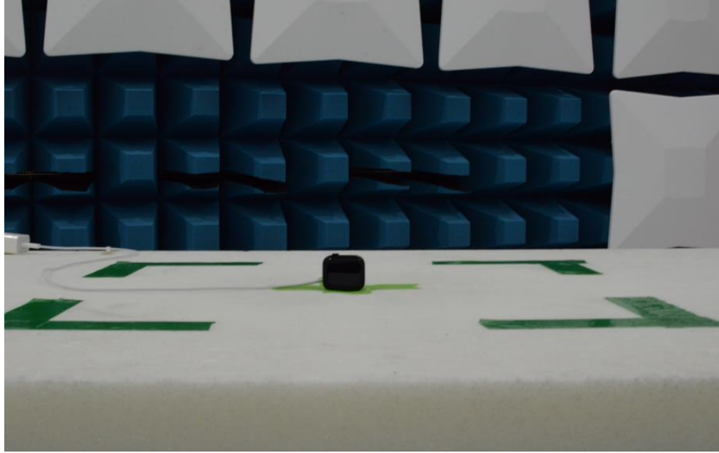
Figure 9: 30MHz-1GHz Test Setup (Front View)
