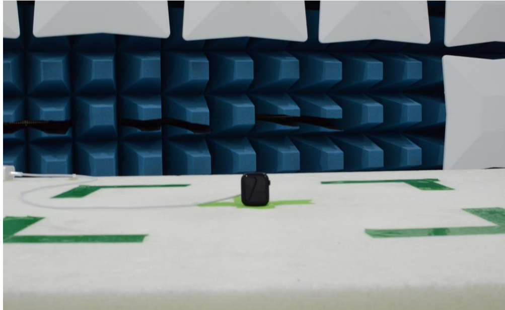
Figure 5: 1-18GHz Test Setup (Front View)
