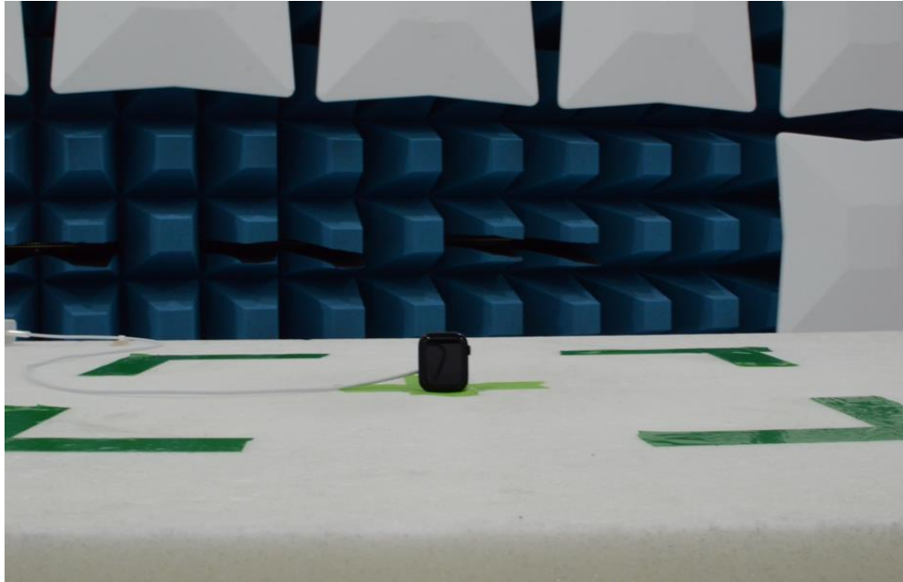
Figure 11: 30MHz-1GHz Test Setup (Front View)
