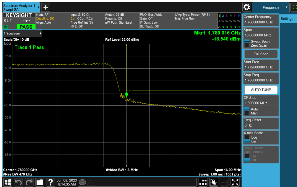
Plot 7-78. Upper Band Edge Plot (LTE Band 66 - 20MHz QPSK – Full RB)
