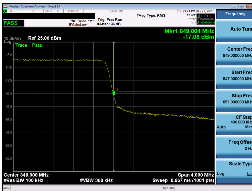
Plot 7-39. Upper BE Plot (LTE Band 5 - 3MHz QPSK – Full RB Configuration)
