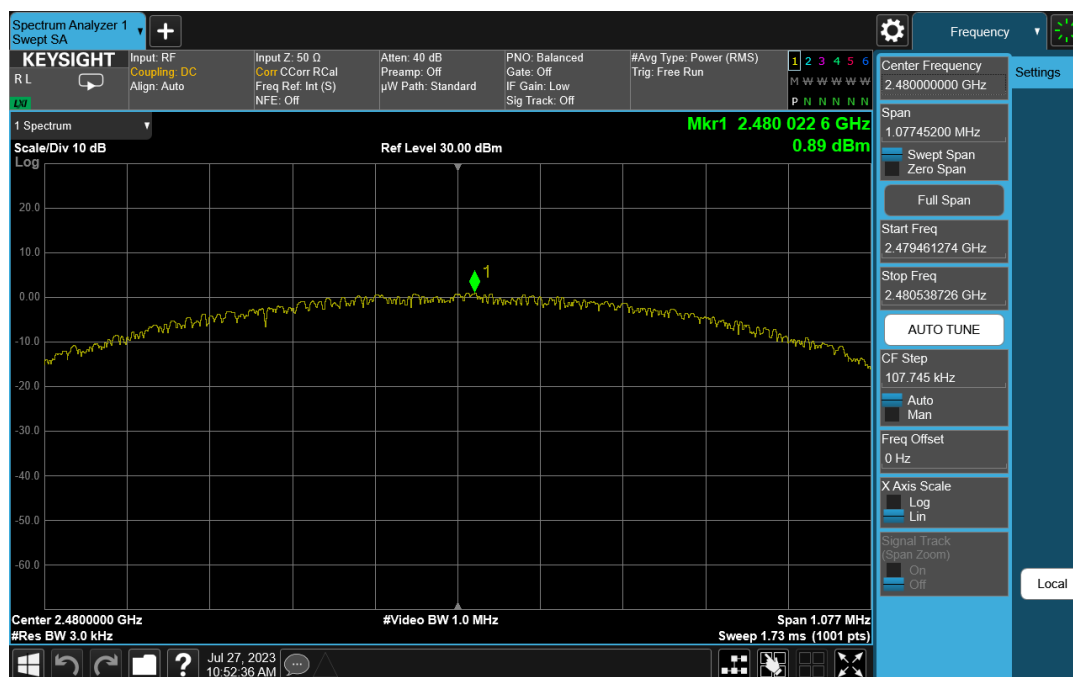
Plot 7-9. Power Spectral Density Plot (Bluetooth (LE), 1Mbps, ePA – Ch. 39)
