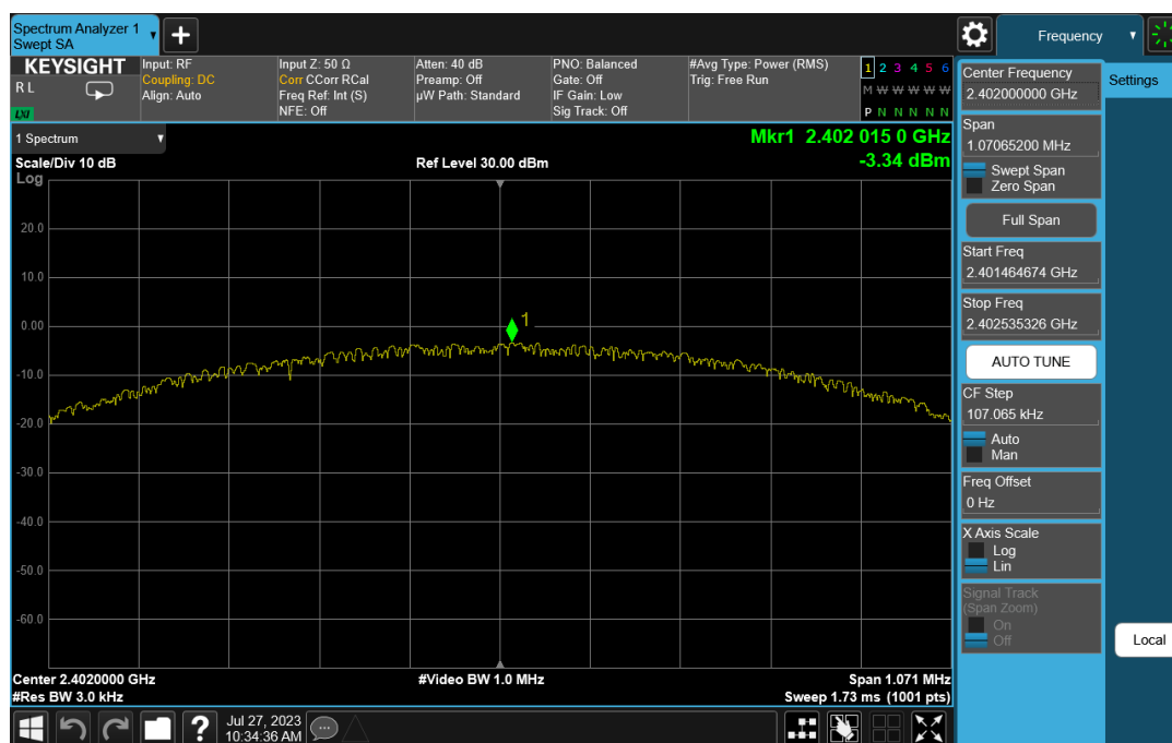
Plot 7-10. Power Spectral Density Plot (Bluetooth (LE), 1Mbps, iPA – Ch. 0)
