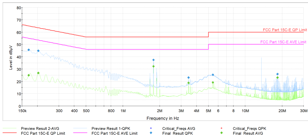
Plot 7-12. AC Line-Conducted Plot (L1, CE B 848kbps, with AC/DC Adapter and Magnetic Charger)
