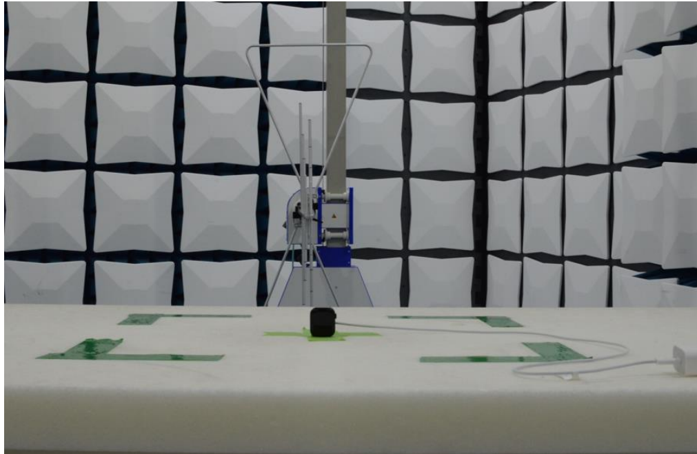
Figure 13: 30MHz-1GHz Test Setup (Rear View)
