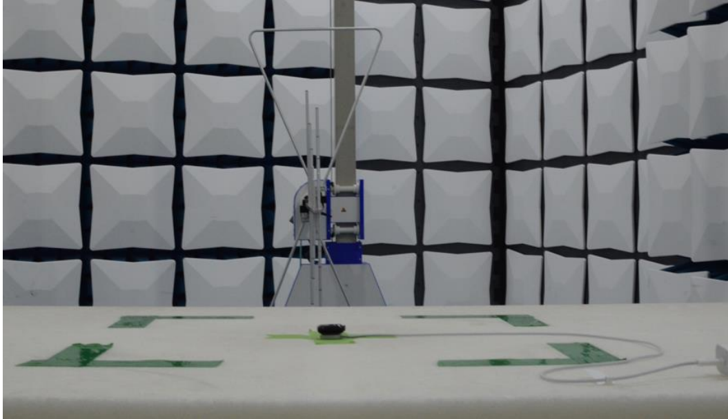
Figure 9: 30MHz-1GHz Test Setup (Rear View)
