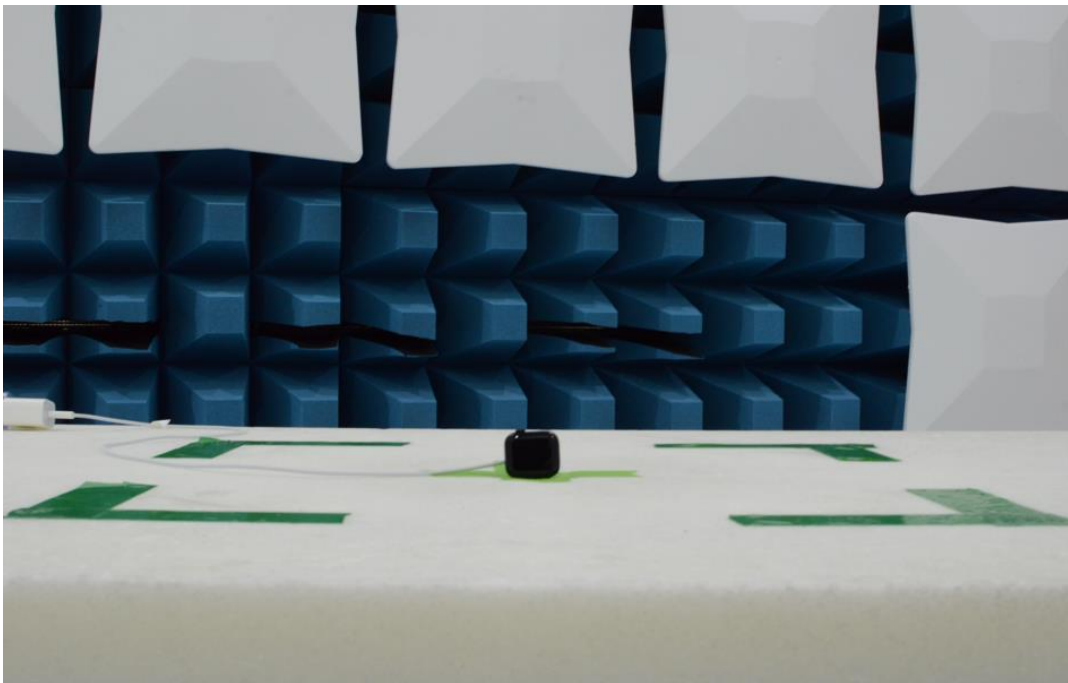
Figure 10: 30MHz-1GHz Test Setup (Front View)
