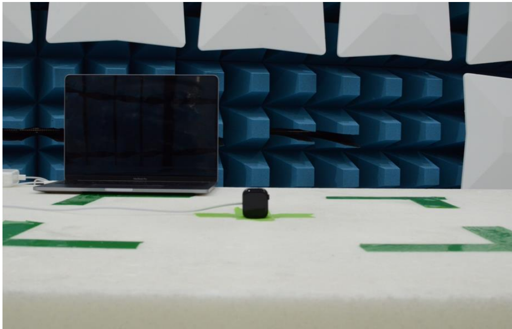
Figure 18: 30MHz-1GHz Test Setup (Front View)
