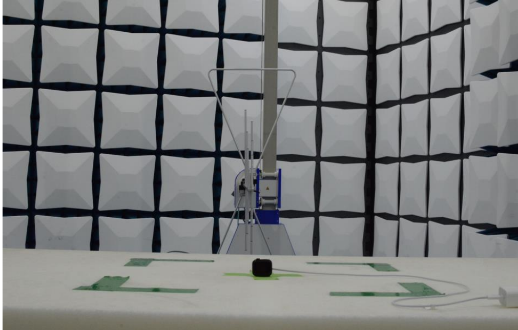
Figure 11: 30MHz-1GHz Test Setup (Rear View)
