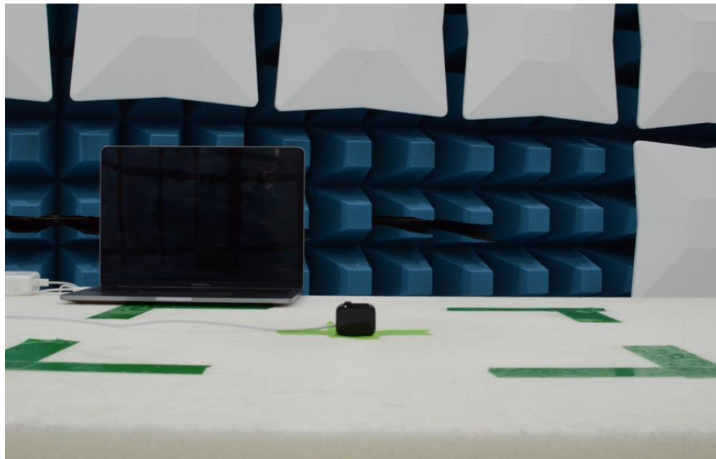
Figure 16: 30MHz-1GHz Test Setup (Front View)
