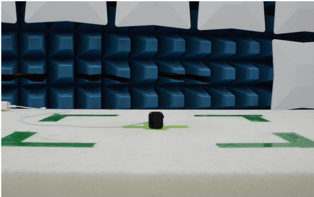
Figure 12: 30MHz-1GHz Test Setup (Front View)
