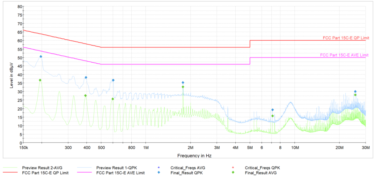
Plot 7-44. AC Line Conducted Plot (Ch. 9, Config 409, Payload 4093 N, with Laptop + Magnetic Charger)
