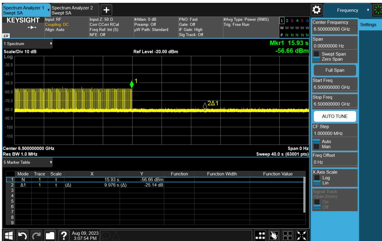
Plot 7-11. Cessation Time – Mode2 (Ch. 5, 6.5 GHz)
