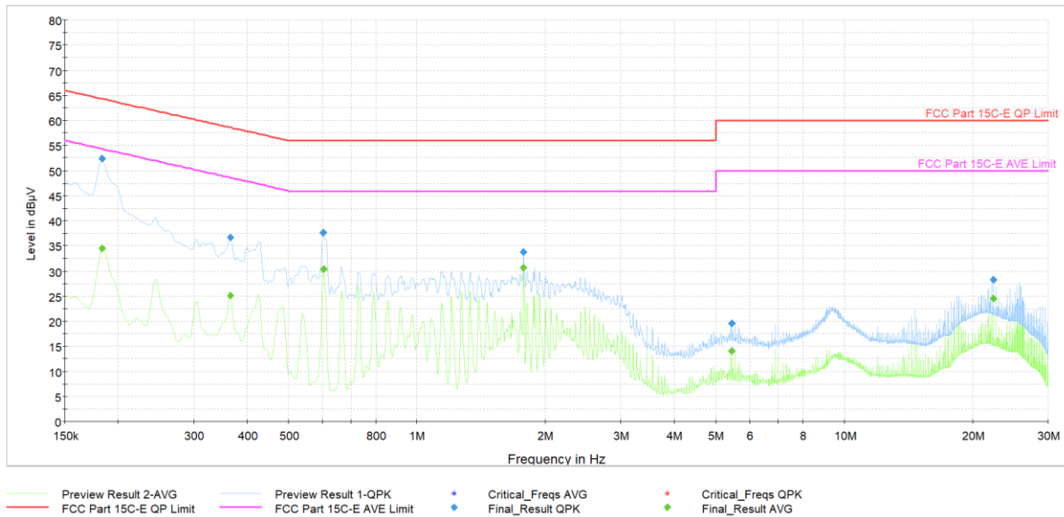
Plot 7-41. AC Line Conducted (Ch. 5, Config 409, Payload 4093 L1, with Laptop + Magnetic Charger)
