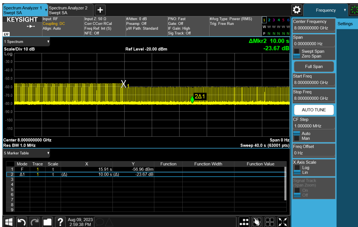
Plot 7-14. Cessation Time – Mode2 (Ch. 9, 8 GHz)
