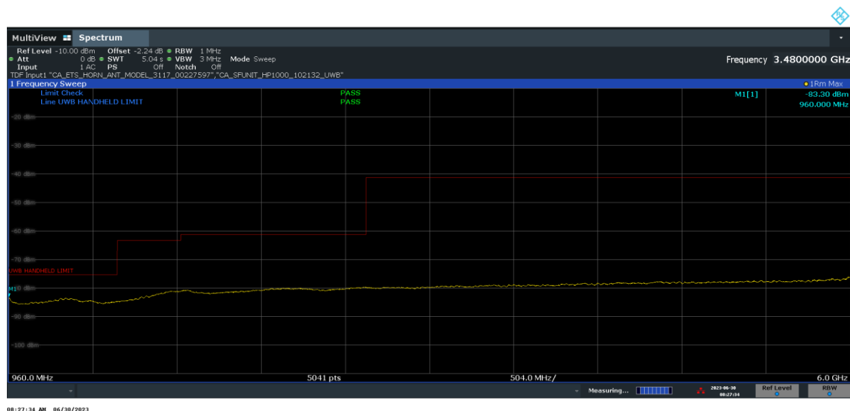
Plot 7-15. FCC Radiated Spurious Emission 960-6000MHz (Ch. 5, Config 409, Payload 4093 Ant. Pol. H)
