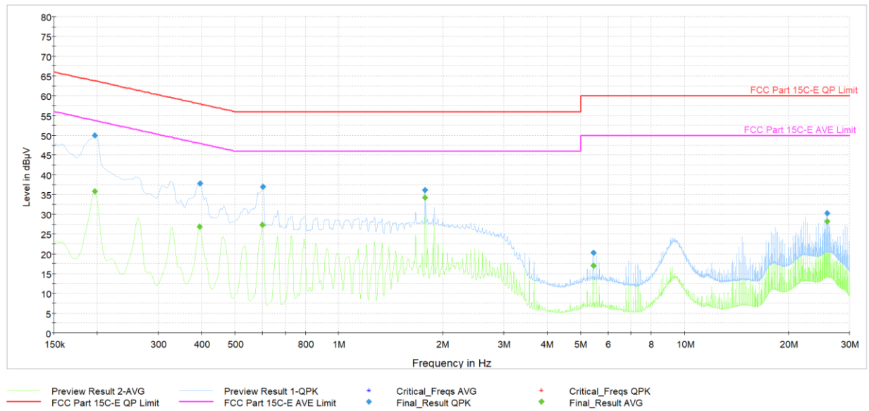
Plot 7-42. AC Line Conducted (Ch. 5, Config 409, Payload 4093 N, with Laptop + Magnetic Charger)
