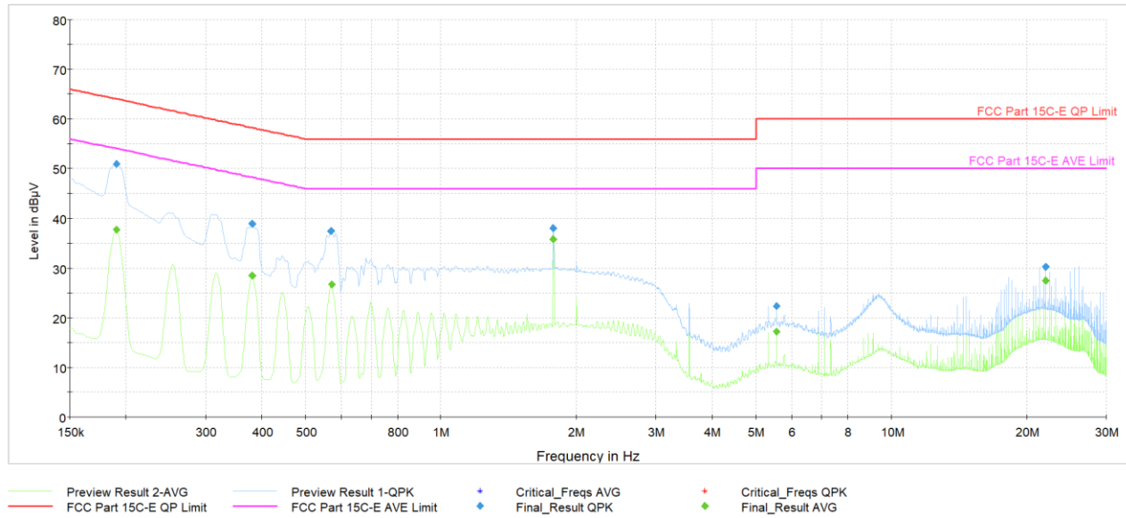
Plot 7-43. AC Line Conducted (Ch. 9, Config 409, Payload 4093 L1, with Laptop + Magnetic Charger)
