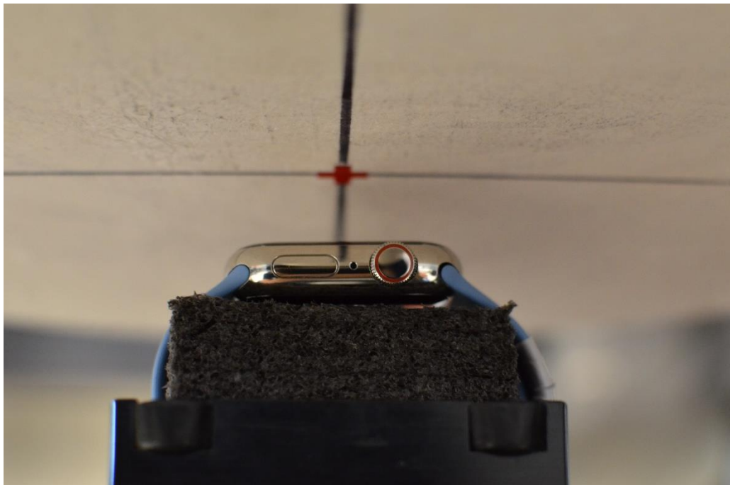
SAR Test Setup Photo 7: Stainless Steel with Sport Wristband, Head, Front Side at 10mm
