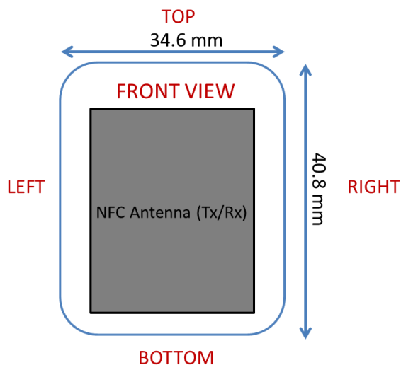
Figure H-2 NFC Antenna Locations
