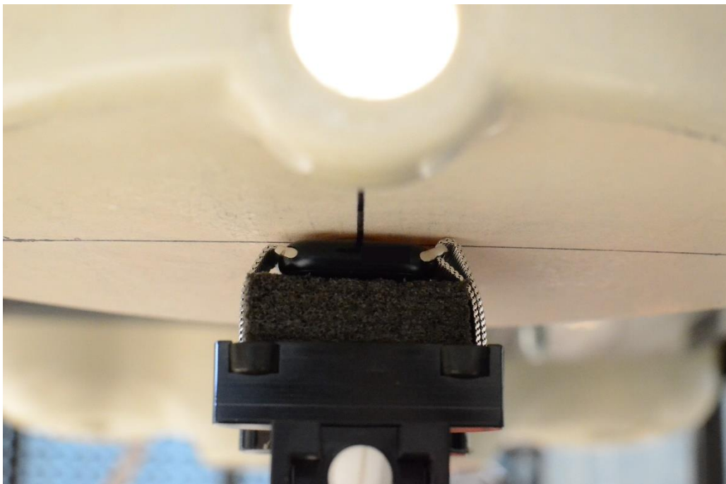
SAR Test Setup Photo 6: Aluminum with Metal Loops Wristband, Extremity, Back Side at 0mm
