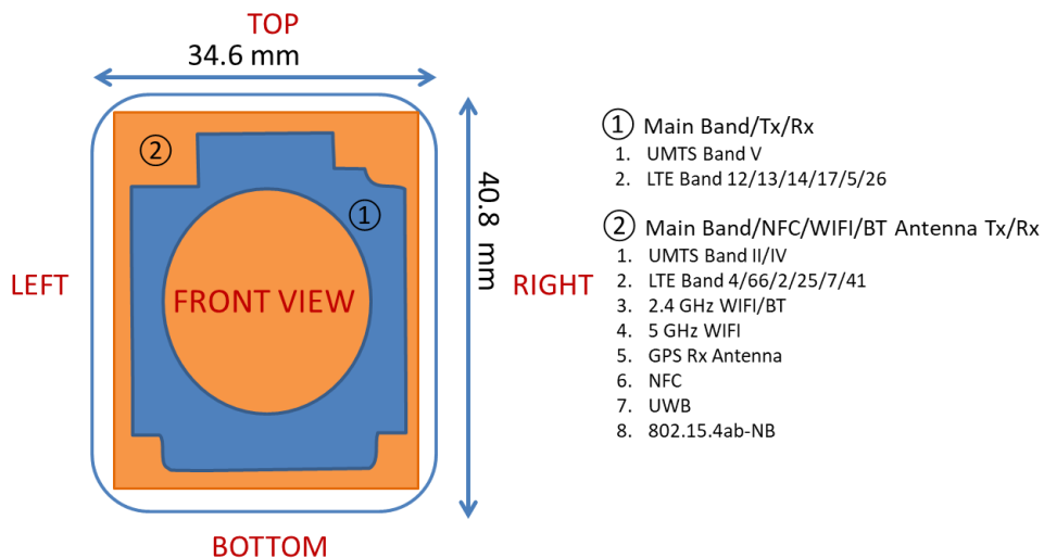
Figure H-1 DUT Antenna Locations
