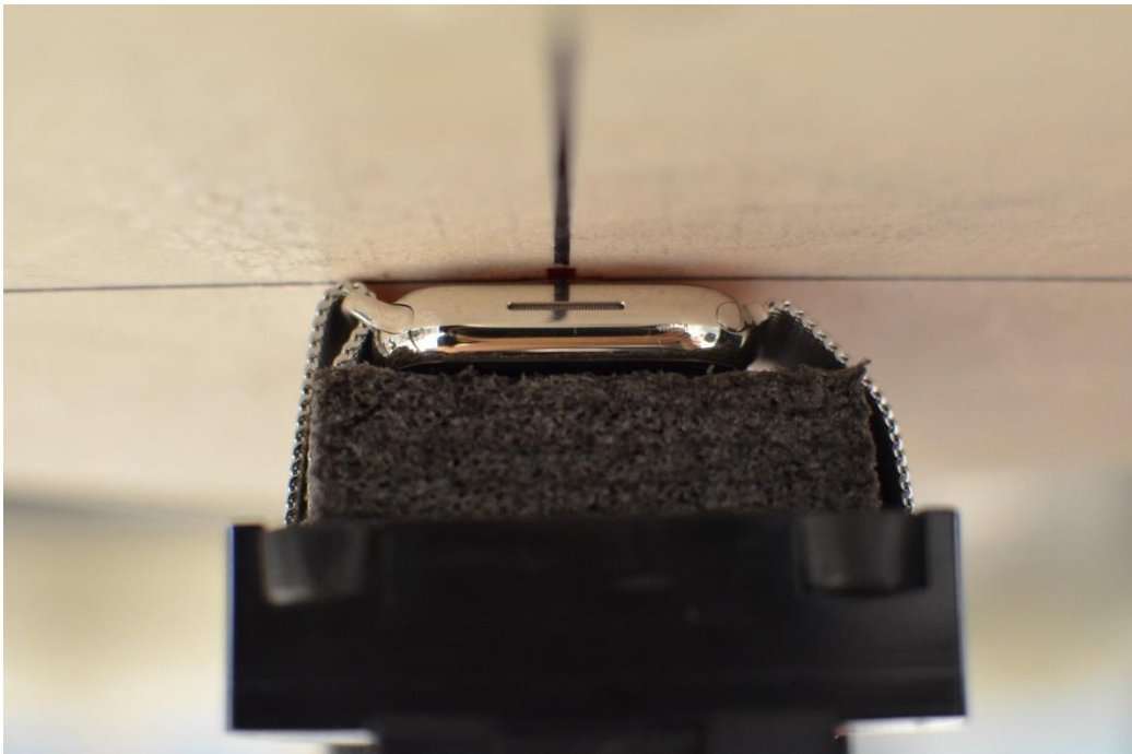
SAR Test Setup Photo 12: Stainless Steel with Metal Loops Wristband, Extremity, Back Side at 0mm
