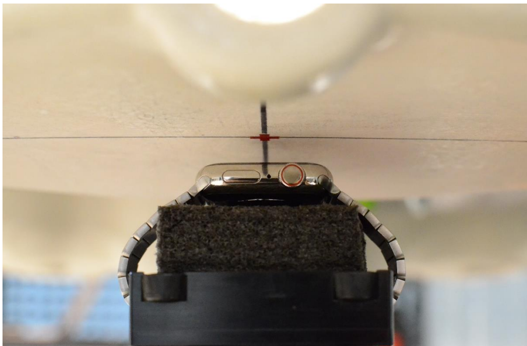
SAR Test Setup Photo 8: Stainless Steel with Metal Links Wristband, Head, Front Side at 10mm
