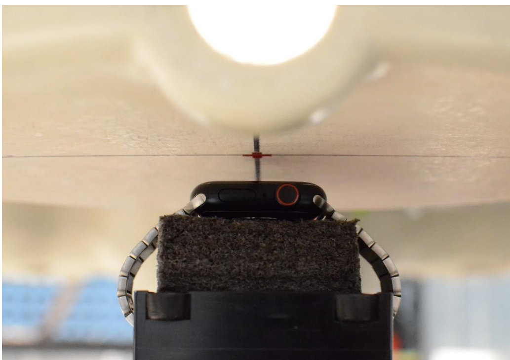
SAR Test Setup Photo 2: Aluminum with Metal Links Wristband, Head, Front Side at 10mm
