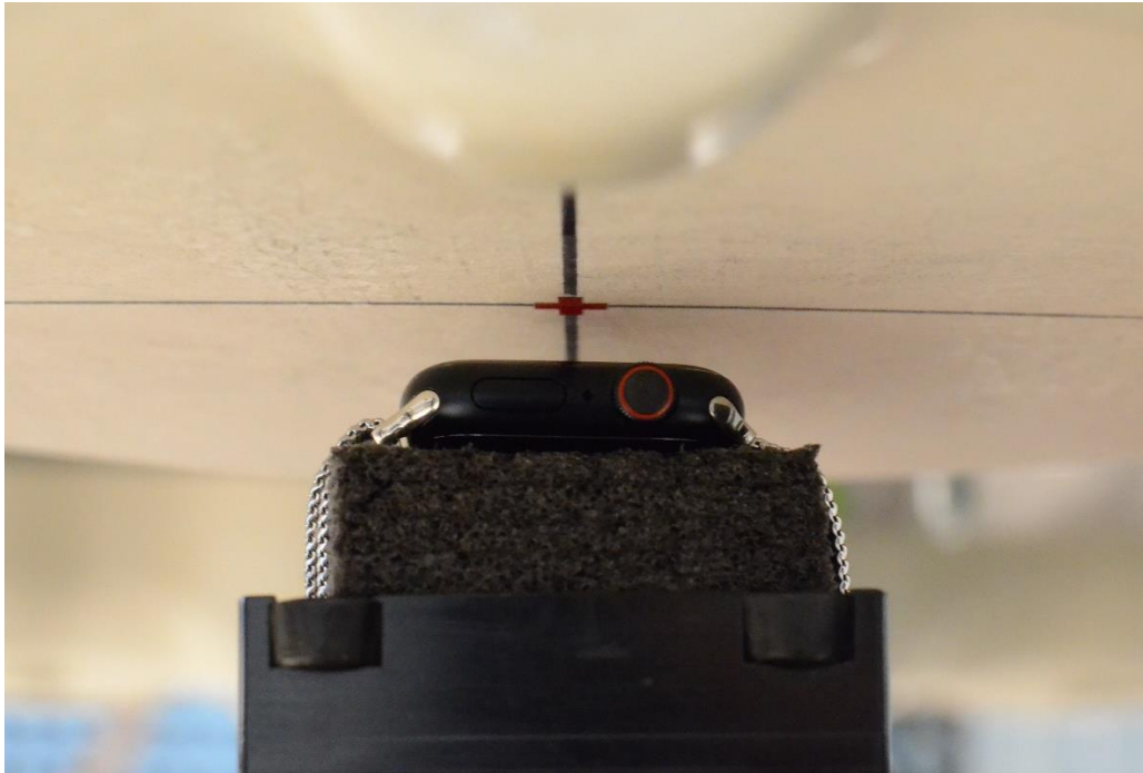
SAR Test Setup Photo 3: Aluminum with Metal Loops Wristband, Head, Front Side at 10mm
