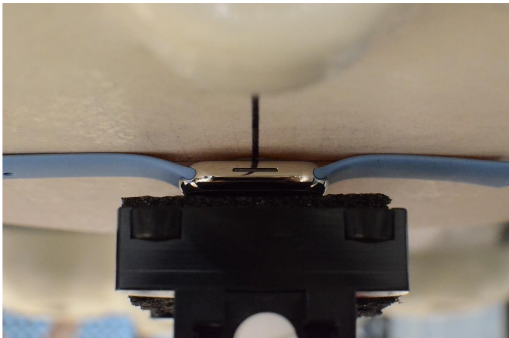
SAR Test Setup Photo 10: Stainless Steel with Sport Wristband, Extremity, Back Side at 0mm
