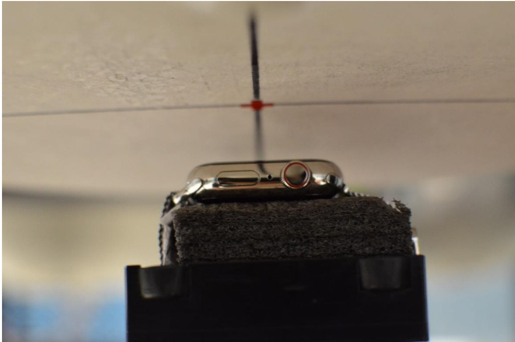
SAR Test Setup Photo 9: Stainless Steel with Metal Loops Wristband, Head, Front Side at 10mm
