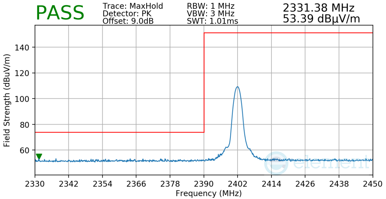
Plot 7-38. Radiated Restricted Lower Band Edge Measurement
