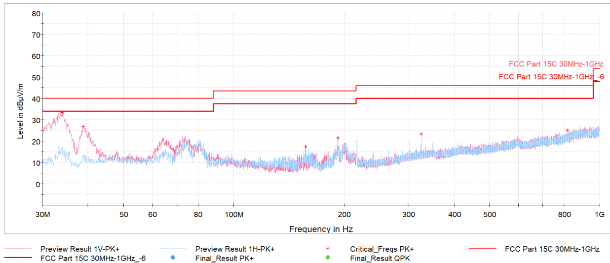
Plot 7-41. Radiated Spurious Emissions Below 1GHz (GFSK ePA – Ch.78, with AC/DC Adapter & Magnetic Charger)
