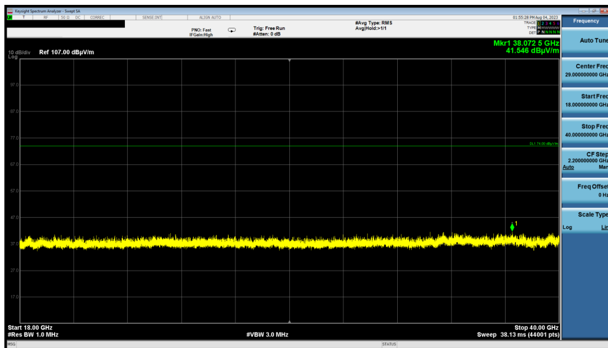
Plot 7-36. Radiated Spurious Emissions above 18GHz Simultaneous Transmission (Pol. V)
