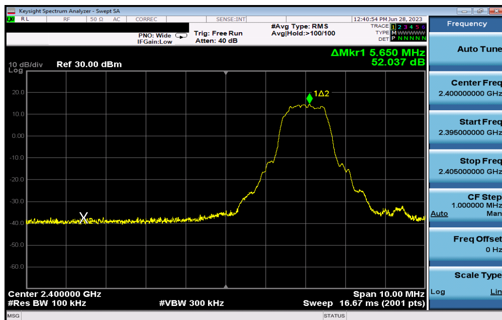
Plot 7-11. Band Edge Plot (Bluetooth with Hopping Disabled, 8DPSK, ePA – Ch. 0)
