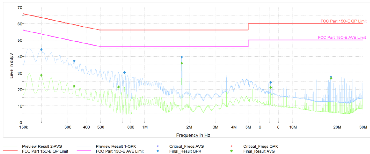
Plot 7-43. AC Line-Conducted Test Plot (L1, GFSK ePA – Ch.78, with AC/DC Adapter & Magnetic Charger)
