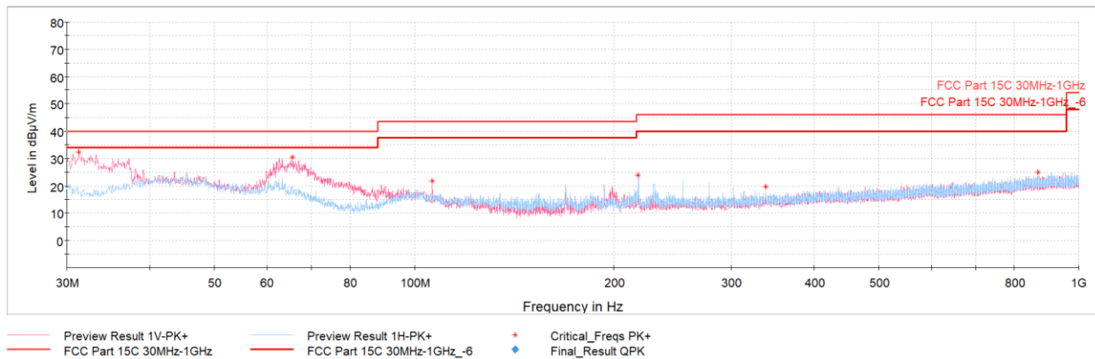
Plot 7-42. Radiated Spurious Emissions – Simultaneous Transmission 30MHz – 1GHz, with AC/DC Adapter & Magnetic Charger
