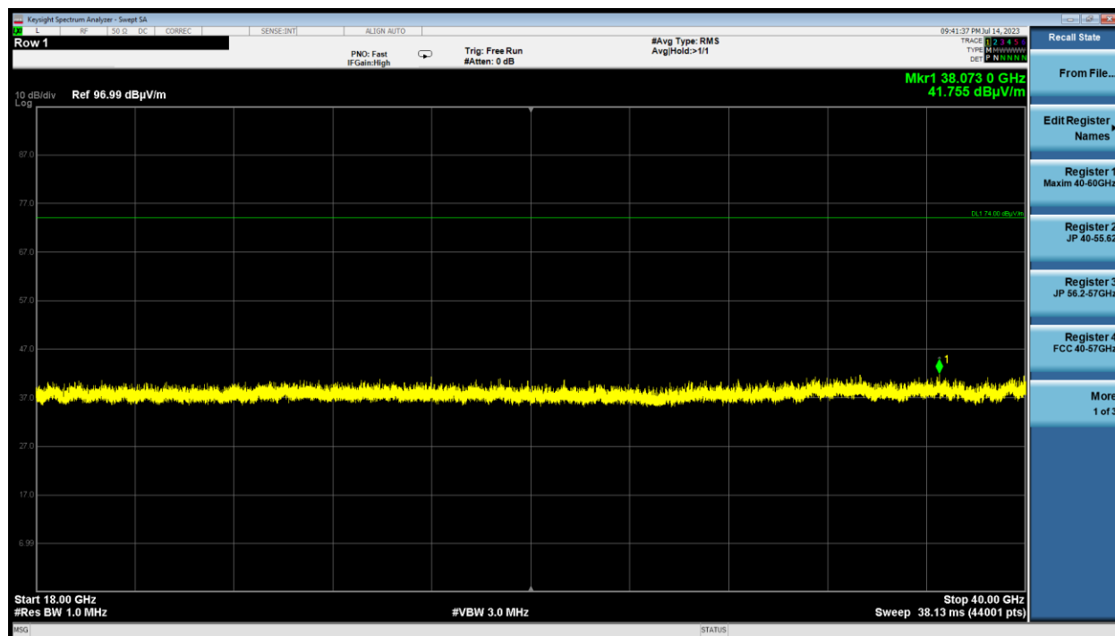
Plot 7-32. Radiated Spurious Emissions above 18GHz (GFSK ePA – Ch.78, Pol. H)
