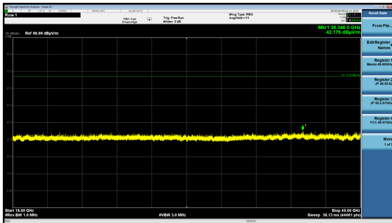
Plot 7-33. Radiated Spurious Emissions above 18GHz (GFSK ePA – Ch.78, Pol. V)
