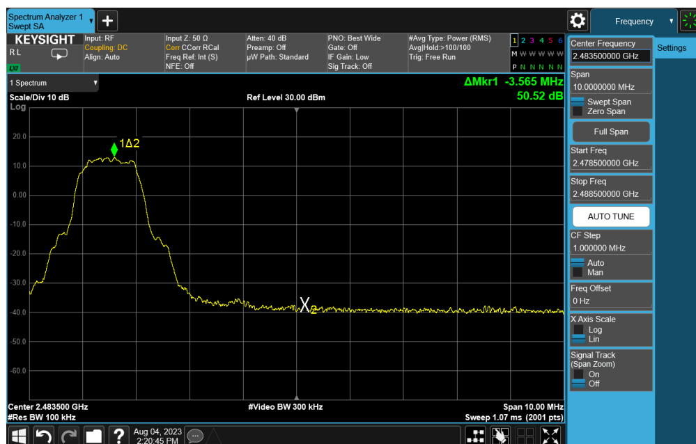
Plot 7-12. Band Edge Plot (Bluetooth with Hopping Disabled, 8DPSK, ePA – Ch. 78)
