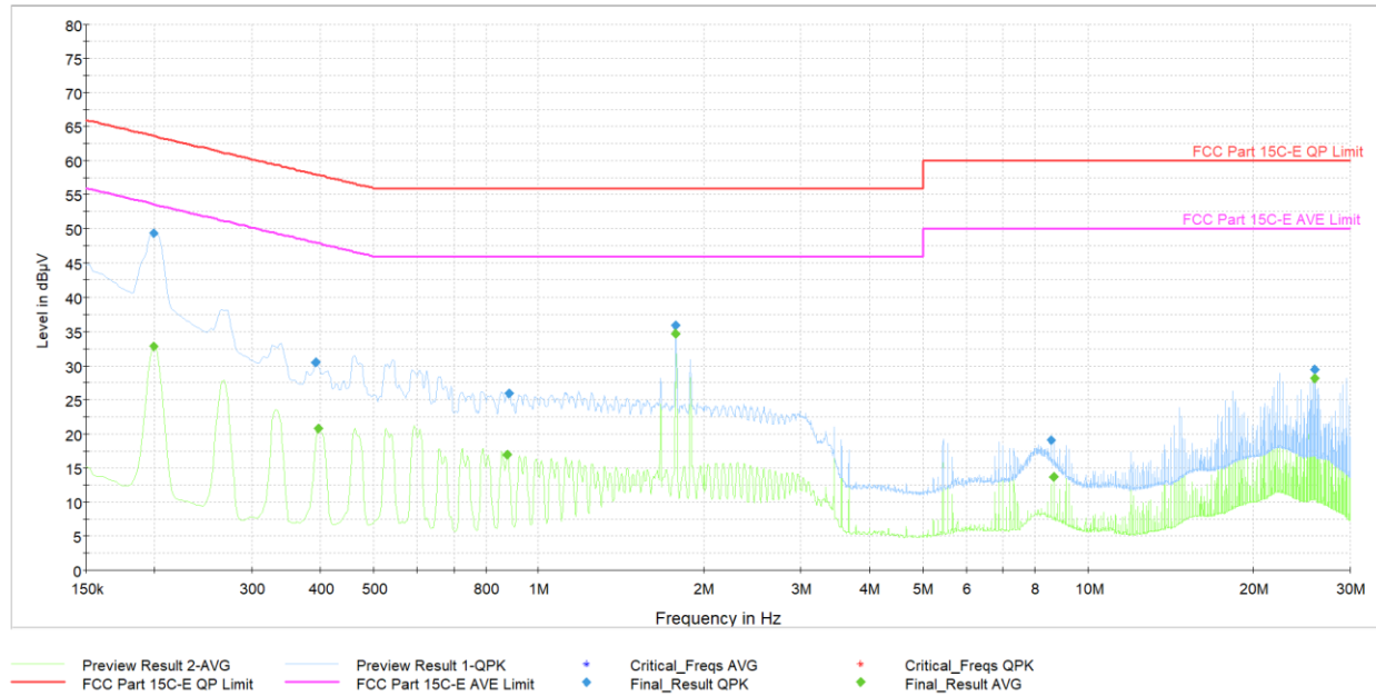
Plot 7-44. AC Line-Conducted Test Plot (N, GFSK ePA – Ch.78, with Laptop & Magnetic Charger)
