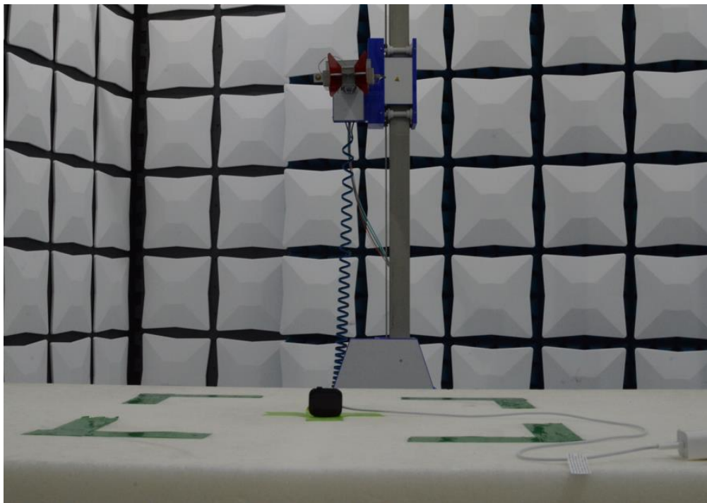
Figure 4: 1-18GHz Test Setup (Rear View)
