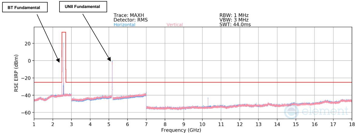
Plot 7-66. Antenna FCM Radiated Spurious Emissions -Simultaneous Transmission 1GHz – 18GHz
