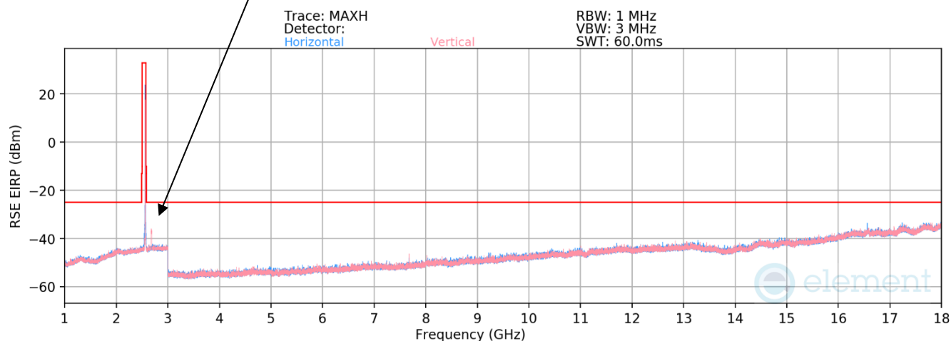
Plot 7-59. Antenna FCM Radiated Spurious Plot above 1GHz (LTE Band 7)
