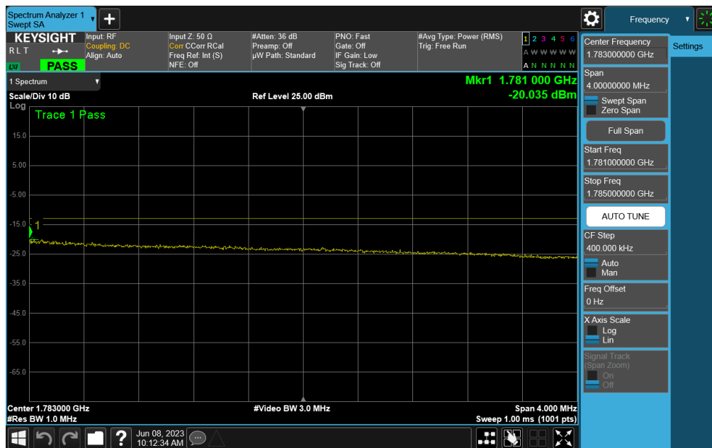
Plot 7-79. Upper Extended Band Edge Plot (LTE Band 66 - 20MHz QPSK – Full RB)
