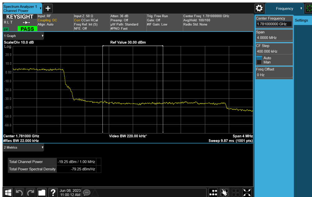
Plot 7-63. Upper Extended Band Edge Plot (LTE Band 66 - 3MHz QPSK – Full RB)
