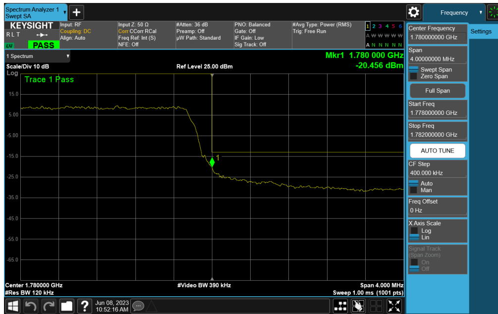
Plot 7-66. Upper Band Edge Plot (LTE Band 66 - 5MHz QPSK – Full RB)
