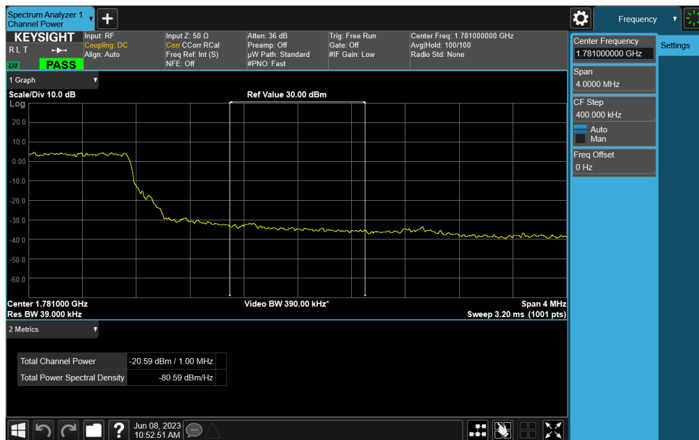
Plot 7-67. Upper Extended Band Edge Plot (LTE Band 66 - 5MHz QPSK – Full RB)
