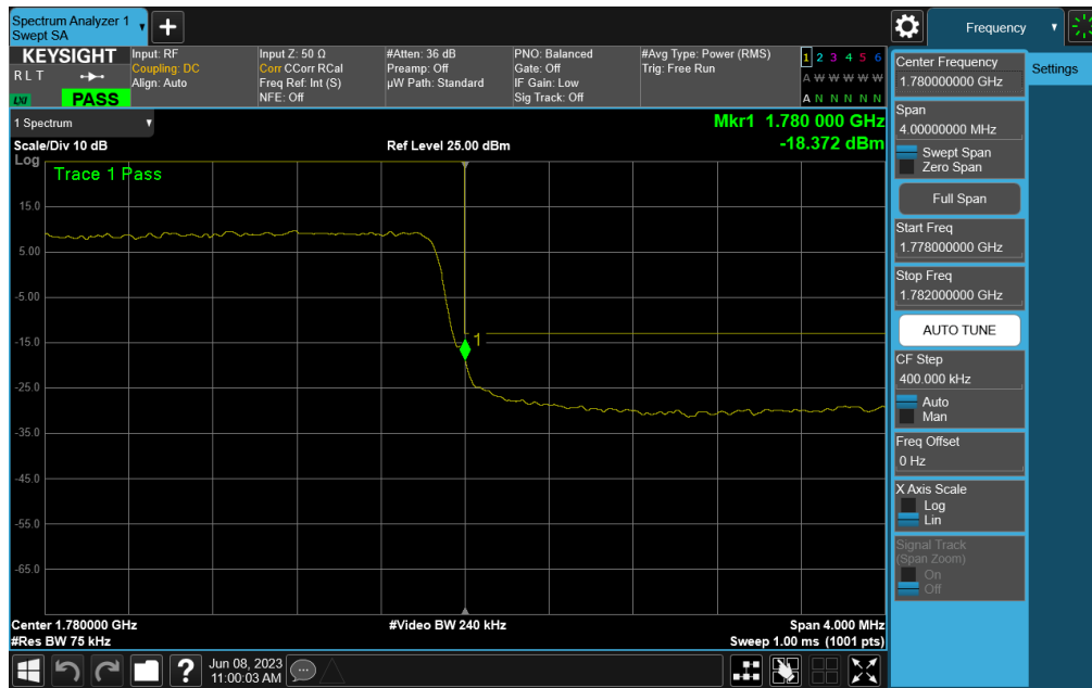
Plot 7-62. Upper Band Edge Plot (LTE Band 66 - 3MHz QPSK – Full RB)
