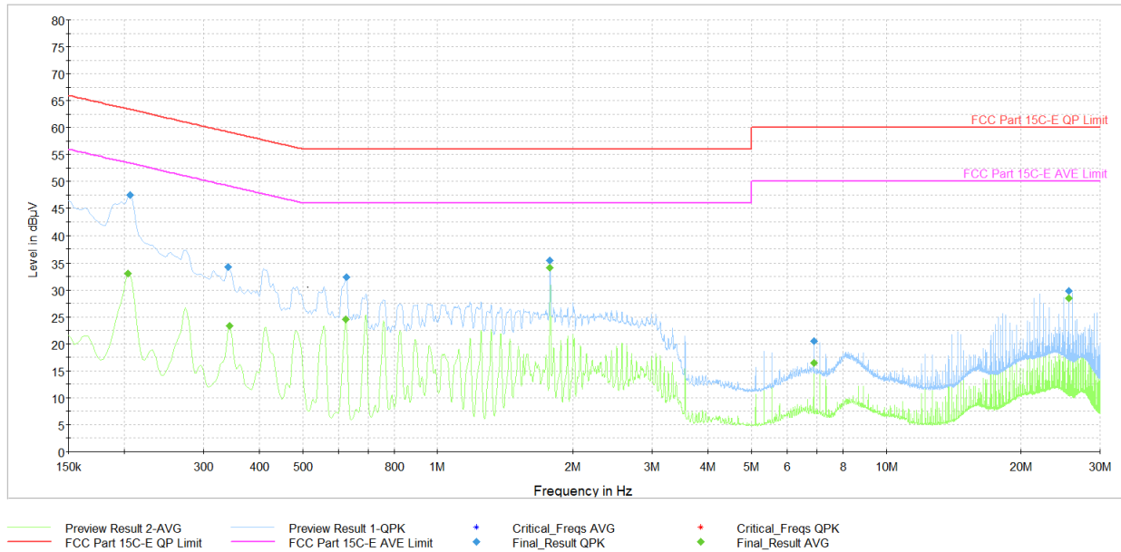
Plot 7-40. AC Line Conducted Plot with Bluetooth HDR (N, 4Mbps ePA - Ch.38 with Laptop + Magnetic Charger)
