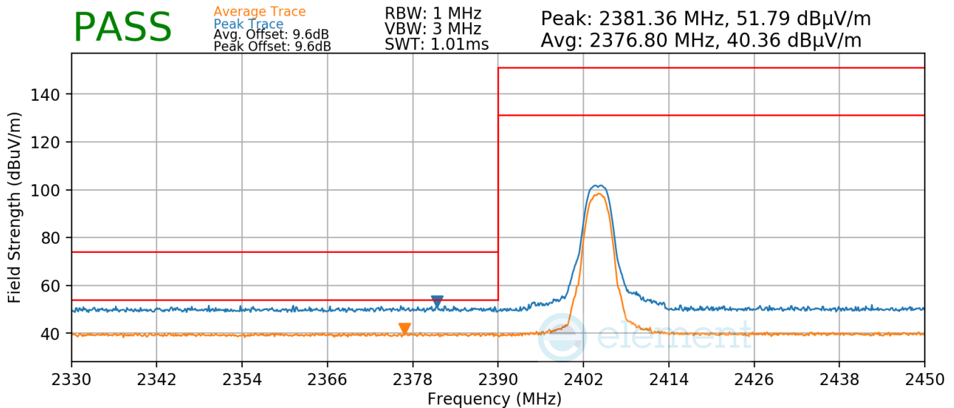
Plot 7-34. Radiated Restricted Lower Band Edge Measurement
