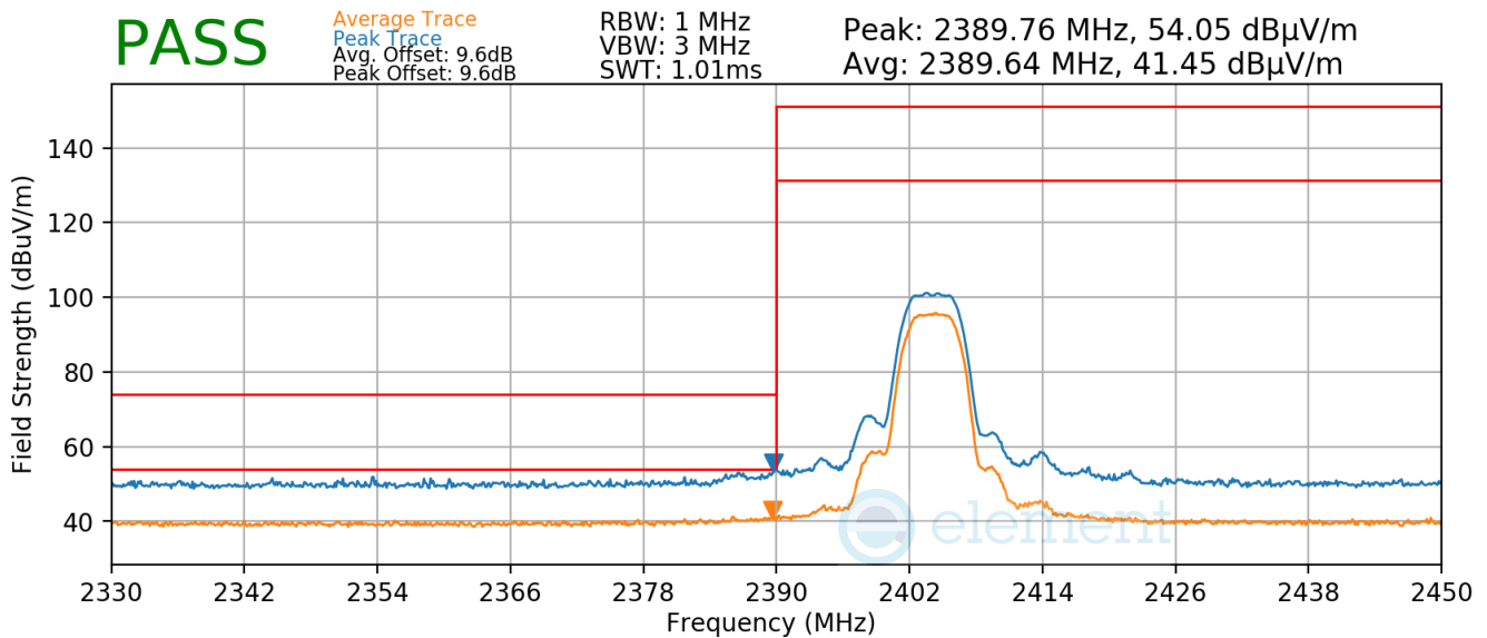
Plot 7-35. Radiated Restricted Lower Band Edge Measurement
