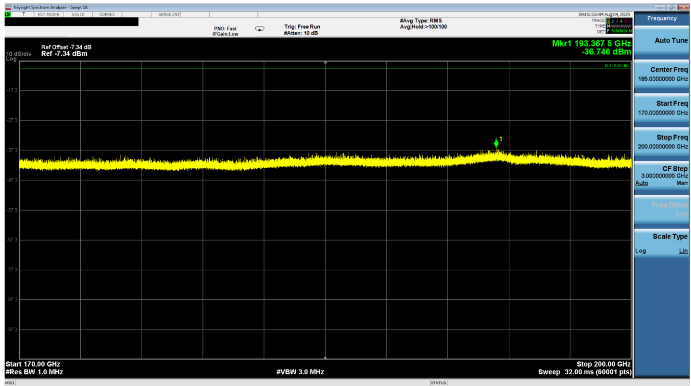
Plot 6-9. Radiated Spurious Emissions 170GHz – 200GHz (Mode 1)
