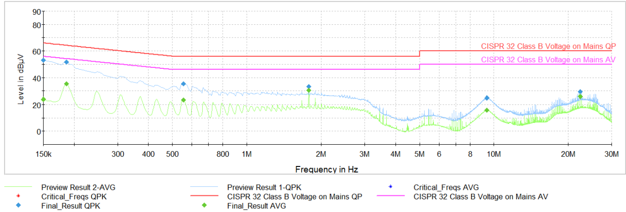
Plot 6-14. AC Line Conducted Plot (N - Mode 1, with Magnetic Charger & Laptop)
