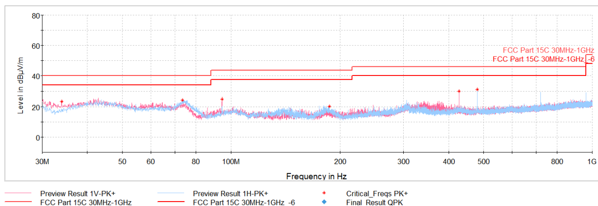
Plot 6-12. Radiated Spurious Emissions 30MHz – 1GHz (Mode 1, with Magnetic Charger & Laptop)
