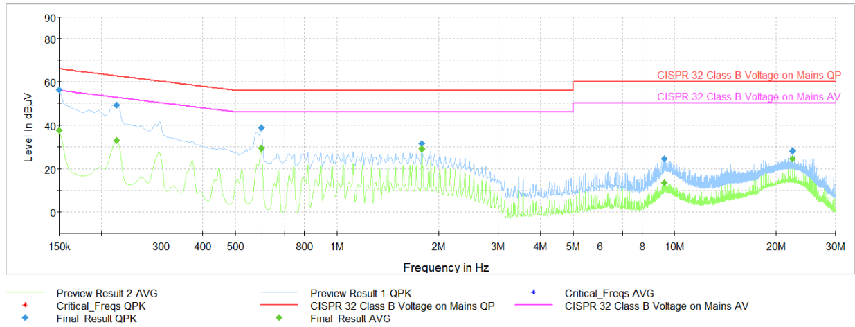
Plot 6-13. AC Line Conducted Plot (L1 - Mode 1, with Magnetic Charger & Laptop)
