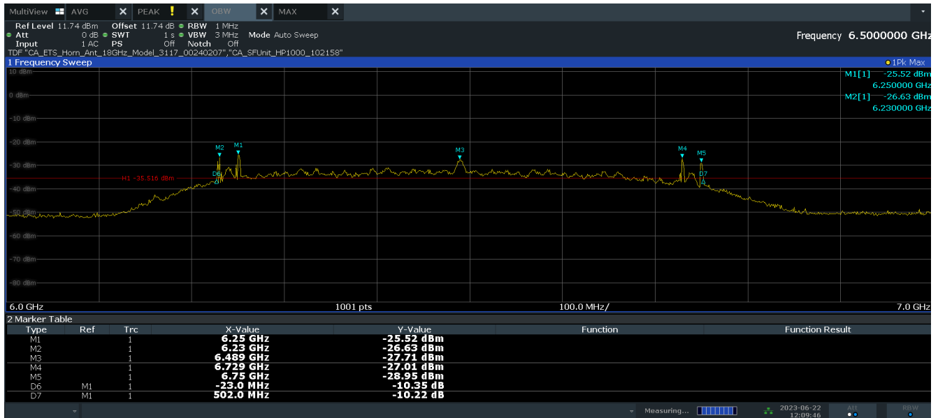
Plot 7-1. 10dBc Bandwidth (Ch. 5, Config 409/Payload 4093)
