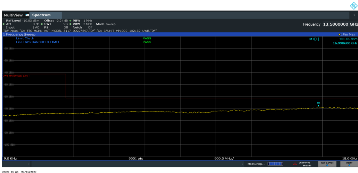
Plot 7-34. Radiated Spurious Emission 9-18GHz (Ch. 9, Config 409, Payload 4093 Ant. Pol. V)
