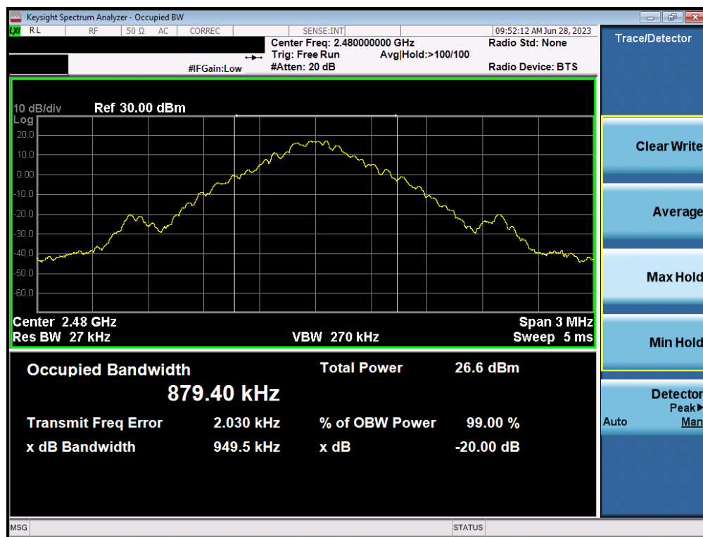
Plot 7-3. 20dB BW and 99% OBW Plot (Bluetooth, GFSK, ePA – Ch. 78)
