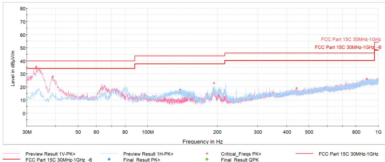
Plot 7-41. Radiated Spurious Emissions Below 1GHz (GFSK ePA – Ch.39, with AC/DC Adapter & Magnetic Charger)
