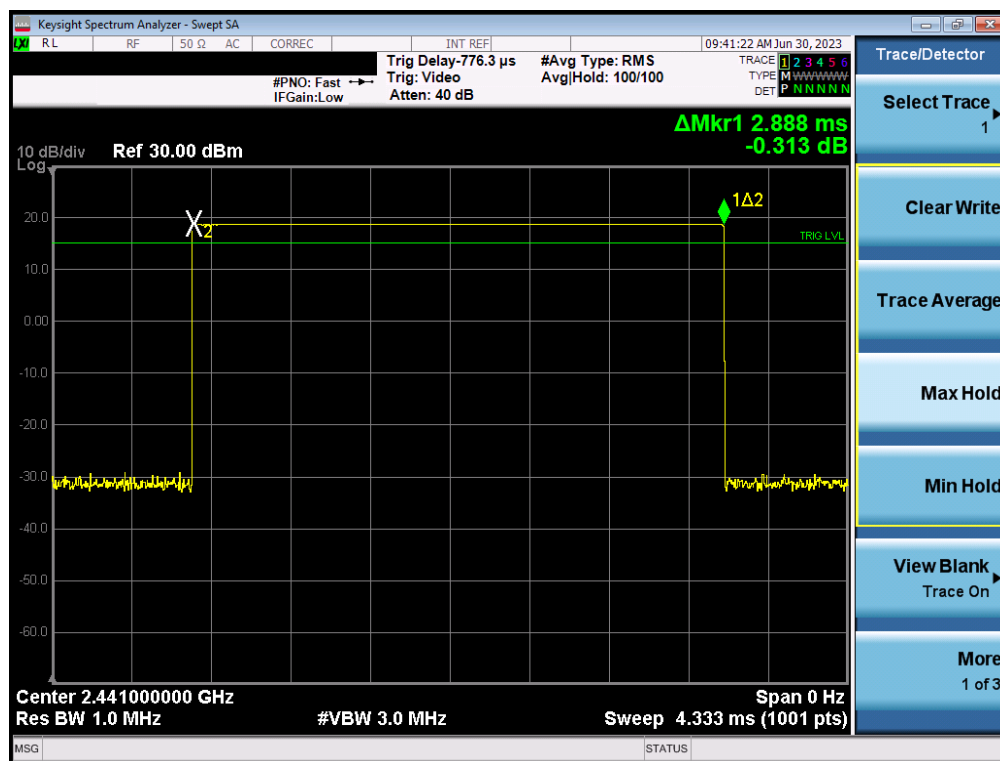
Plot 7-17. Time of Occupancy Plot (Bluetooth, GFSK, ePA)
