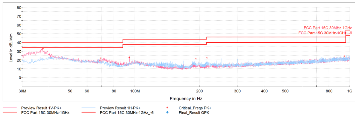
Plot 7-42. Radiated Spurious Emissions Below 1GHz – Simultaneous Transmission
