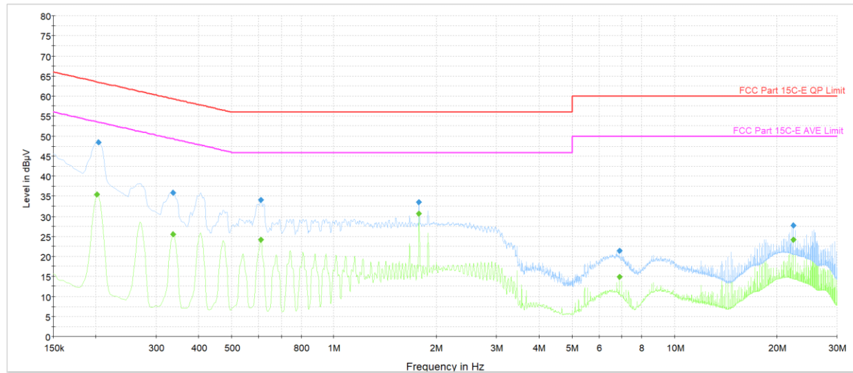
Plot 7-43. AC Line-Conducted Test Plot (L1, GFSK ePA – Ch.39, with Laptop + Magnetic Charger)
