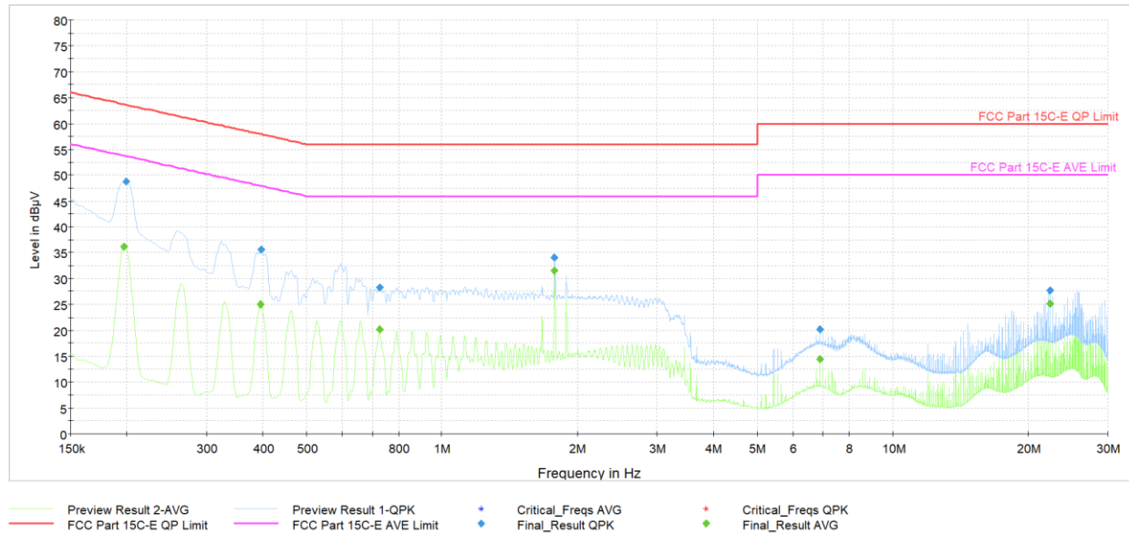
Plot 7-44. AC Line-Conducted Test Plot (N, GFSK ePA – Ch.39, with Laptop + Magnetic Charger)
