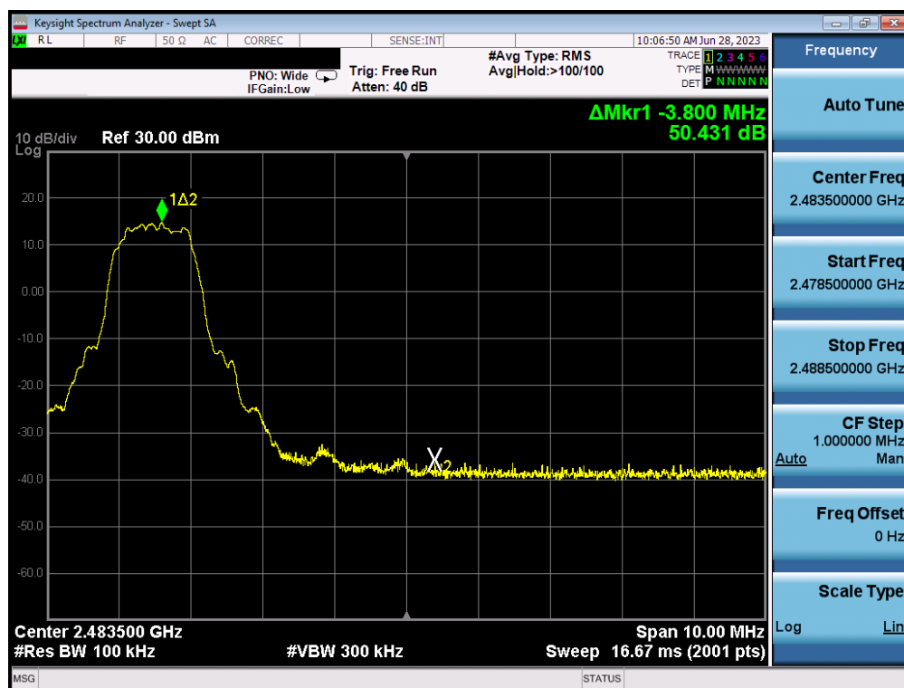
Plot 7-12. Band Edge Plot (Bluetooth with Hopping Disabled, 8DPSK, ePA – Ch. 78)
