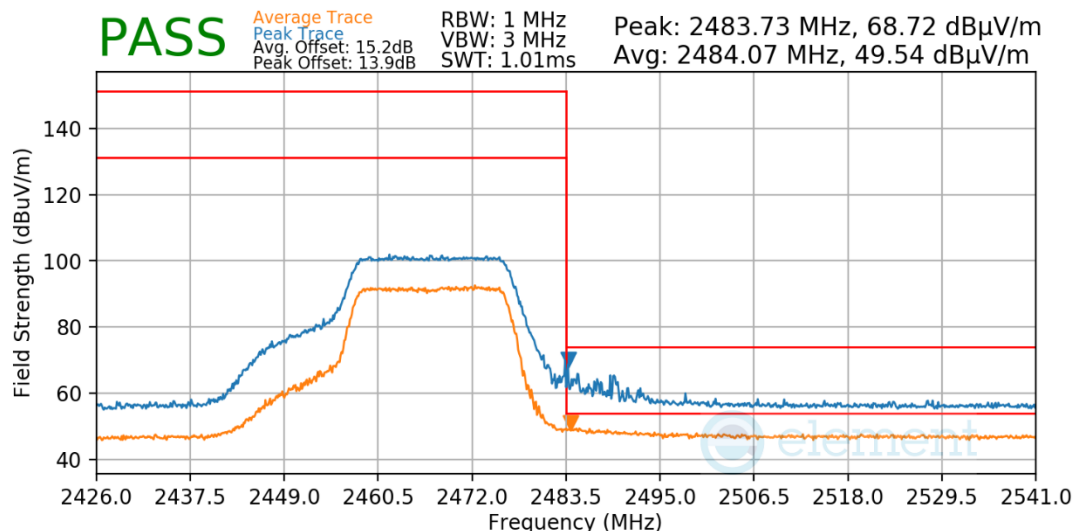
Plot 7-70. Radiated Restricted Upper Band Edge Measurement
