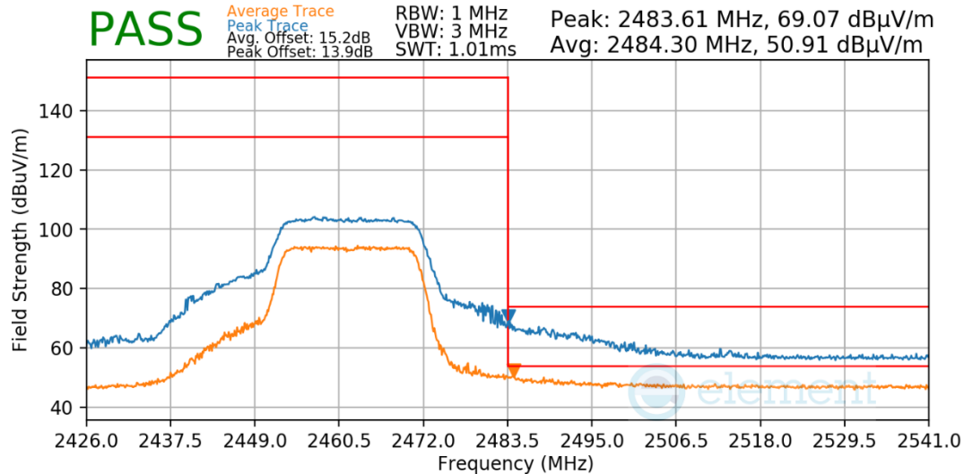
Plot 7-69. Radiated Restricted Upper Band Edge Measurement
