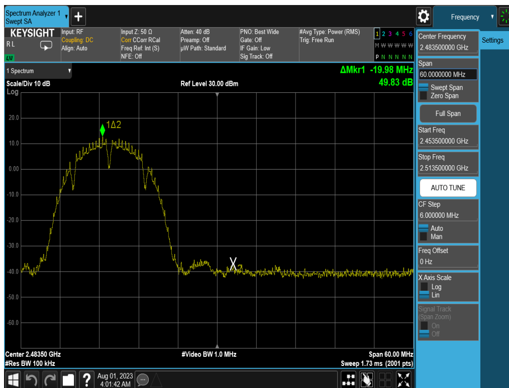
Plot 7-26. Band Edge Plot (802.11b – Ch. 12) – 1Mbps
