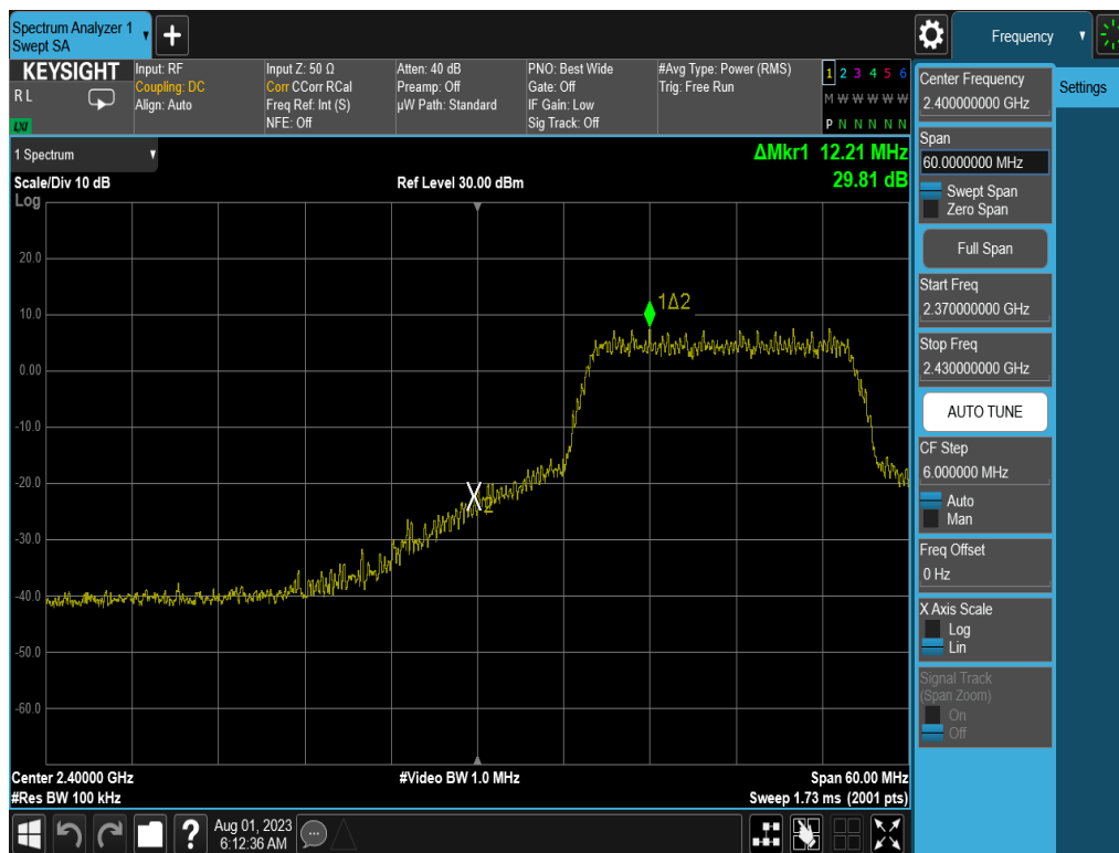
Plot 7-41. Band Edge Plot (802.11n (2.4GHz) – Ch. 2) – MCS7
