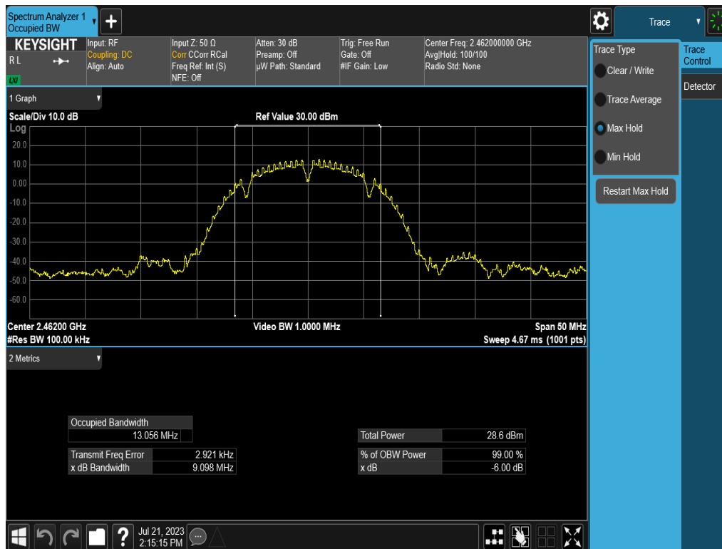
Plot 7-3. 6dB Bandwidth & 99% OBW Plot (802.11b – Ch. 11) – 1Mbps
