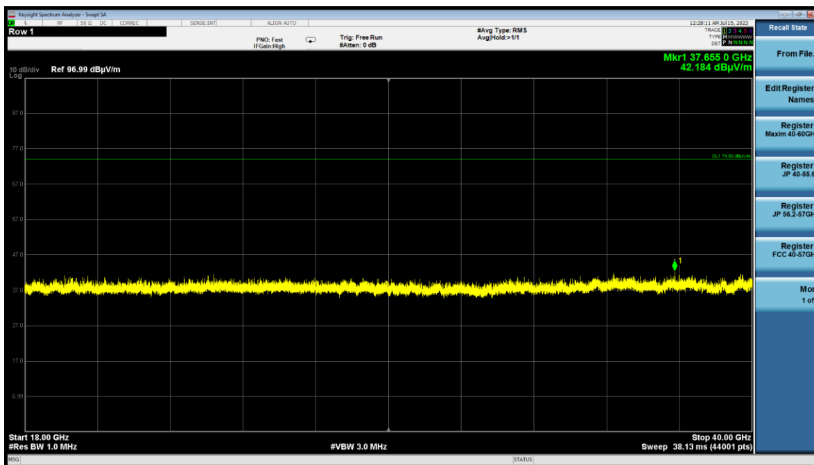
Plot 7-32. Radiated Spurious Emissions above 18GHz (BT GFSK ePA – Ch.39, Pol.H)
