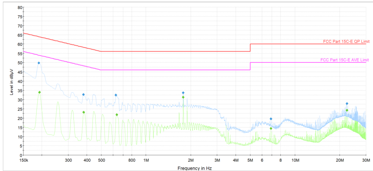
Plot 7-39. AC Line Conducted Plot with Bluetooth LE (L1, 1Mbps ePA – Ch.19 with AC/DC Adapter + Laptop Charger)
