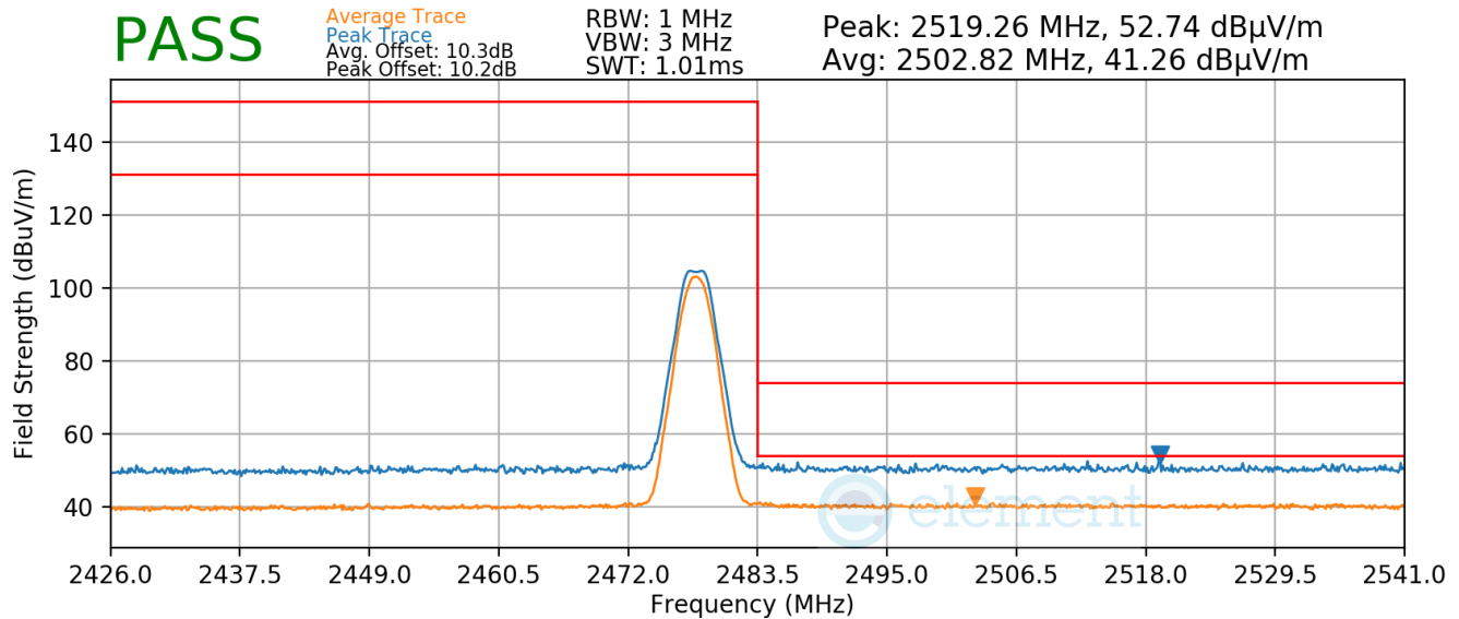
Plot 7-37. Radiated Restricted Upper Band Edge Measurement
