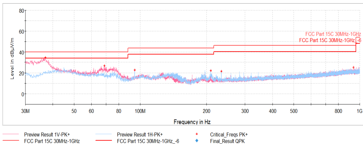
Plot 7-38. Radiated Spurious Emissions Below 1GHz (1Mbps, ePA – Ch.19, Pol. H & V, with AC/DC Adapter + Magnetic Charger)
