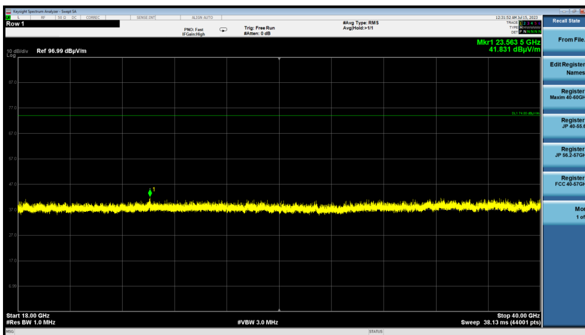
Plot 7-33. Radiated Spurious Emissions above 18GHz (BT GFSK ePA – Ch.39, Pol V)
