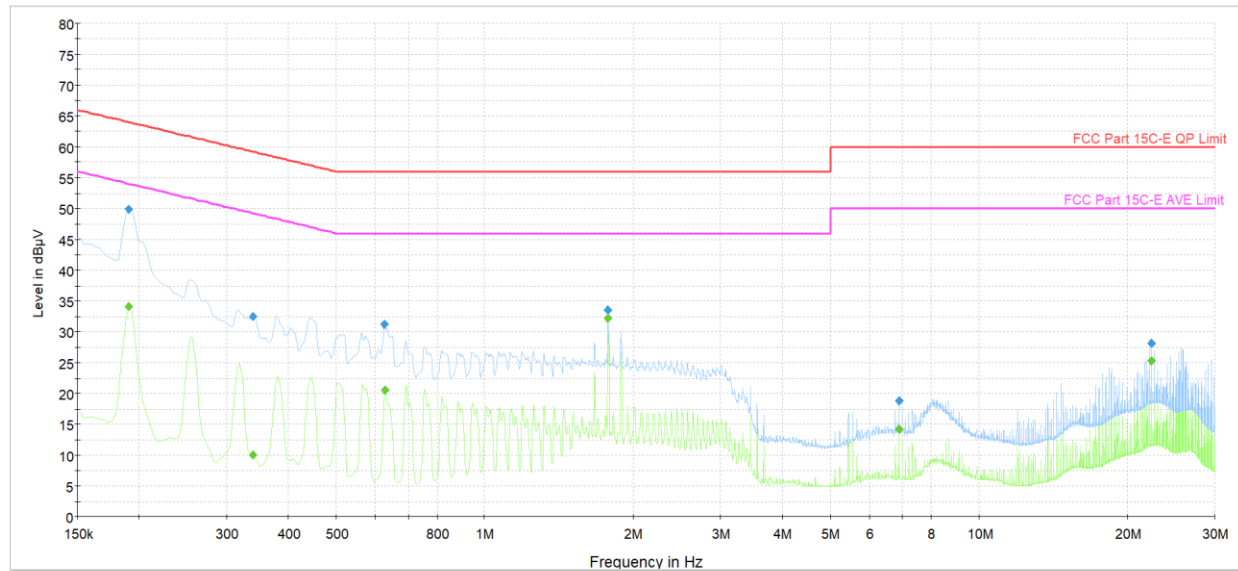
Plot 7-40. AC Line Conducted Plot with Bluetooth LE (N, 1Mbps ePA – Ch.19, with AC/DC Adapter + Laptop Charger)
