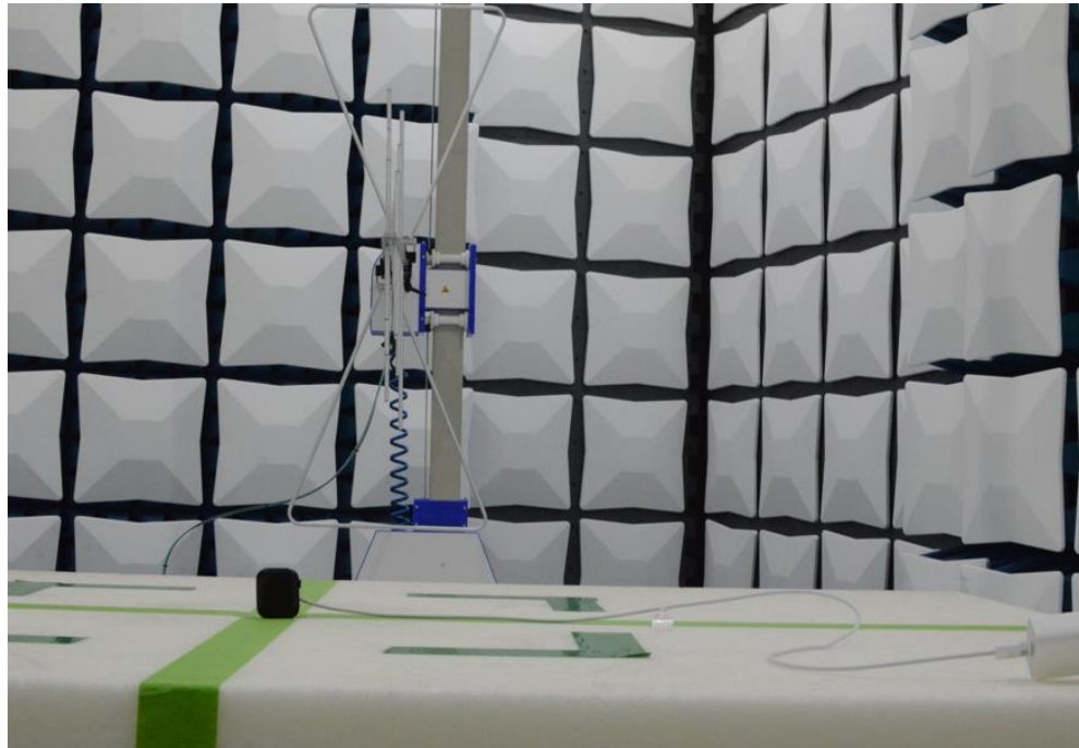
Figure 16: 30MHz-1GHz Test Setup (Rear View)
