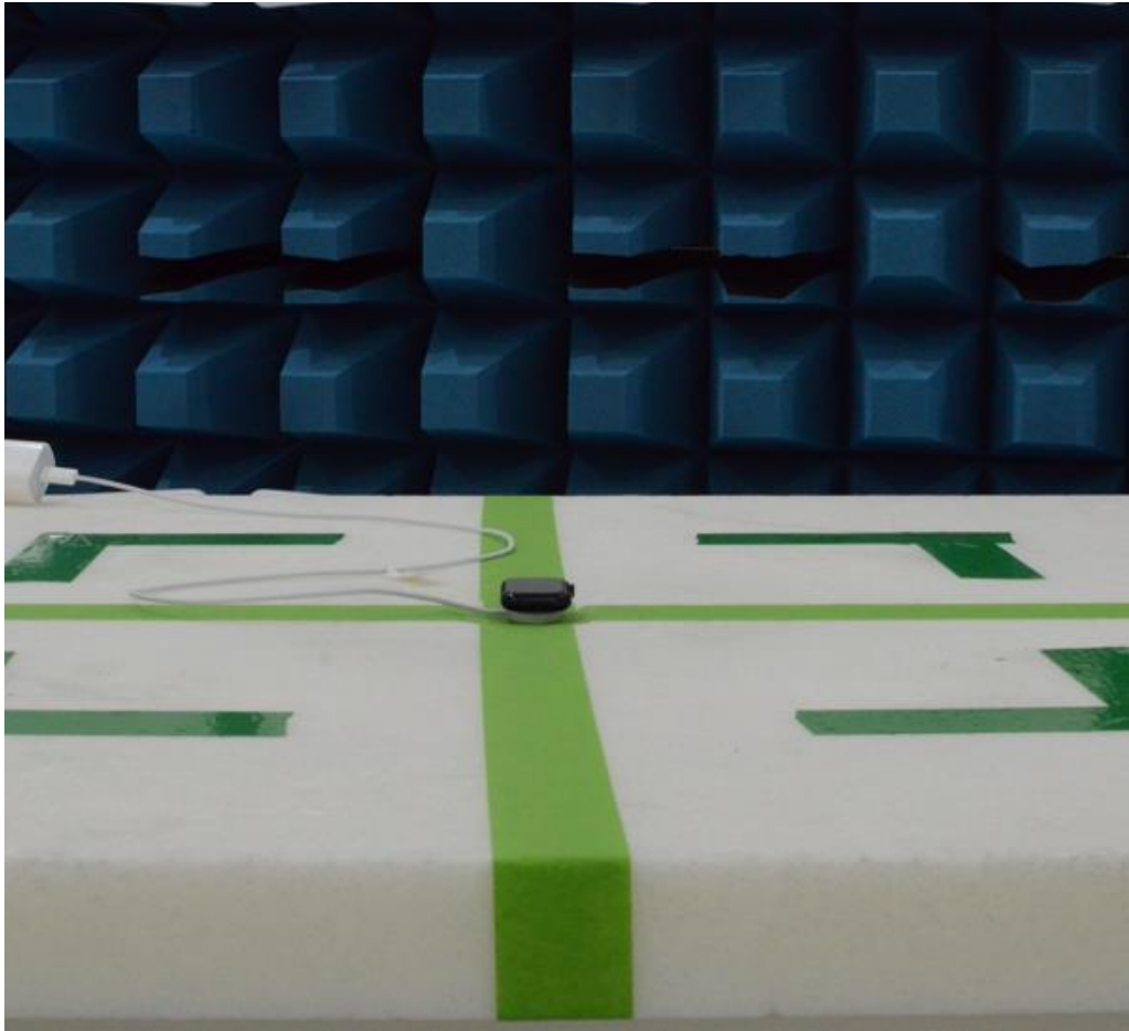
Figure 5: 1-18GHz Test Setup (Front View)
