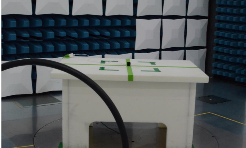
Figure 25: 9kHz-30MHz Test Setup (Front View)
