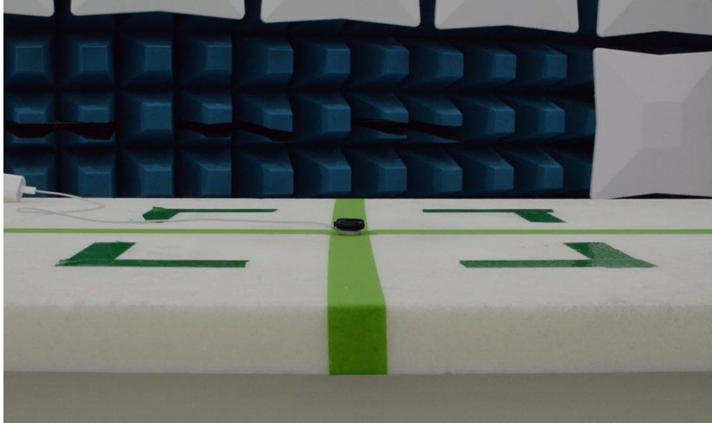
Figure 11: 30MHz-1GHz Test Setup (Front View)
