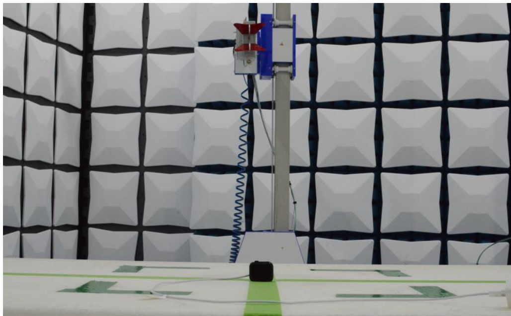
Figure 8: 1-18GHz Test Setup (Rear View)
