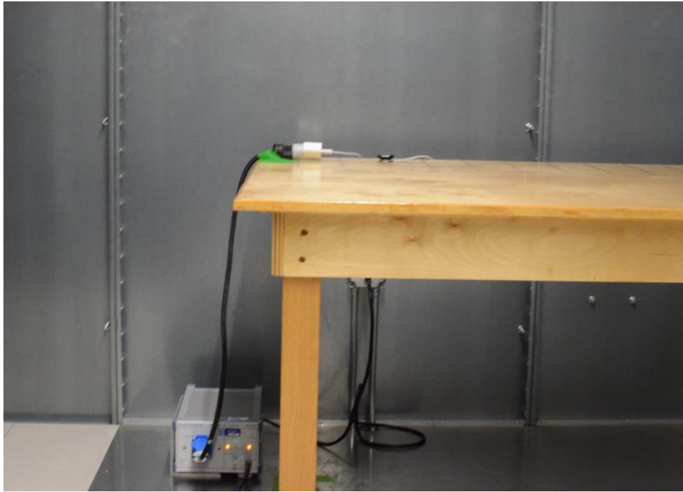
Figure 1: AC Line Conducted Emissions (Front View)
