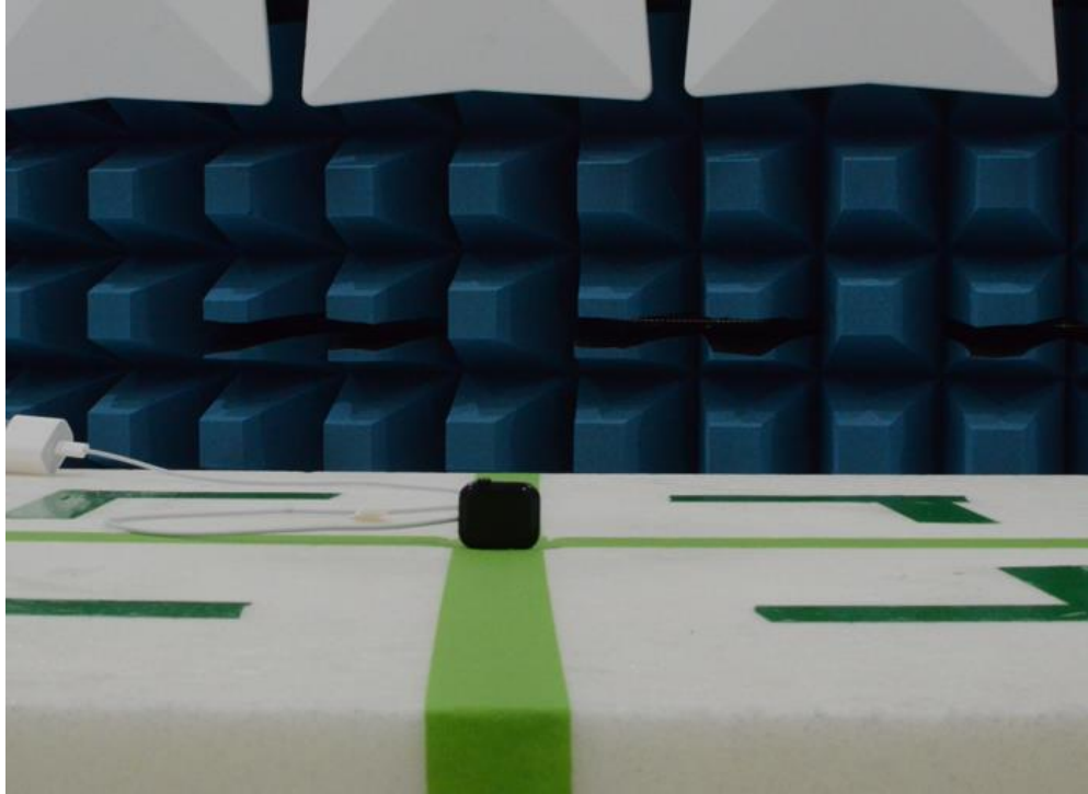
Figure 13: 30MHz-1GHz Test Setup (Front View)
