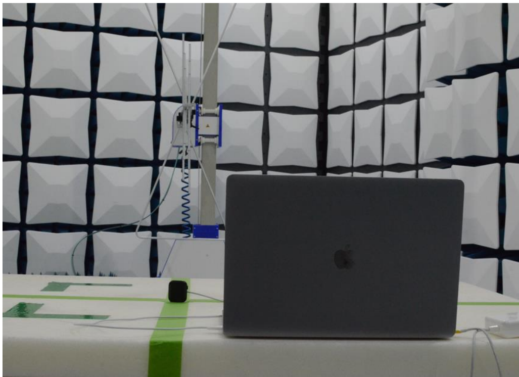
Figure 22: 30MHz-1GHz Test Setup (Rear View)
