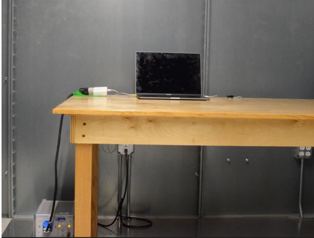
Figure 3: AC Line Conducted Emissions (Front View)
