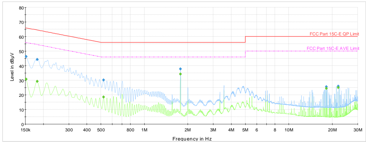
Plot 7-63. AC Line Conducted Plot with 802.11n – Ch.144 (L1), with AC/DC Adapter & magnetic charger
