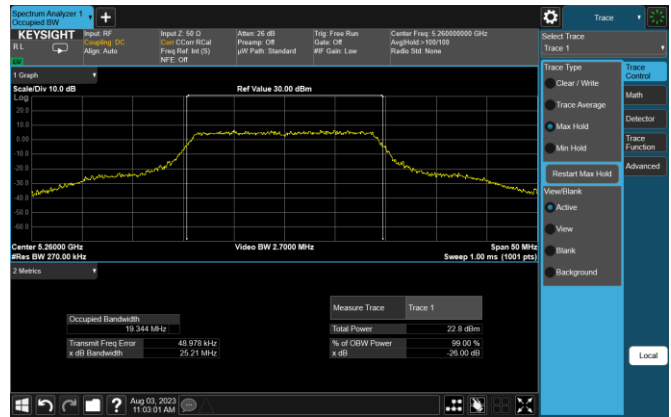
Plot 7-4. 26dB BW & 99% OBW (20MHz BW 802.11n – Ch. 52, MCS0)
