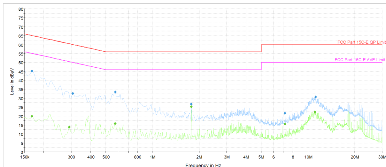
Plot 7-39. AC Line Conducted Plot with Bluetooth HDR (L1, 4Mbps ePA - Ch.38 with AC/DC Adapter + Laptop Charger)
