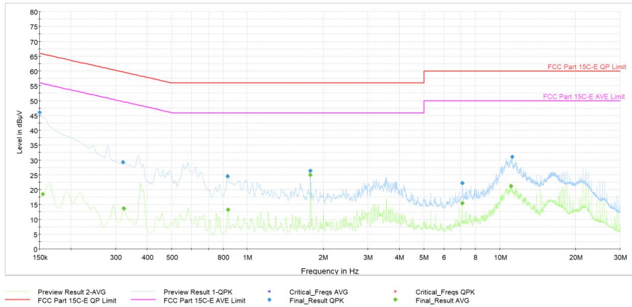
Plot 7-40. AC Line Conducted Plot with Bluetooth HDR (N, 4Mbps ePA - Ch.38 with AC/DC Adapter + Laptop Charger)
