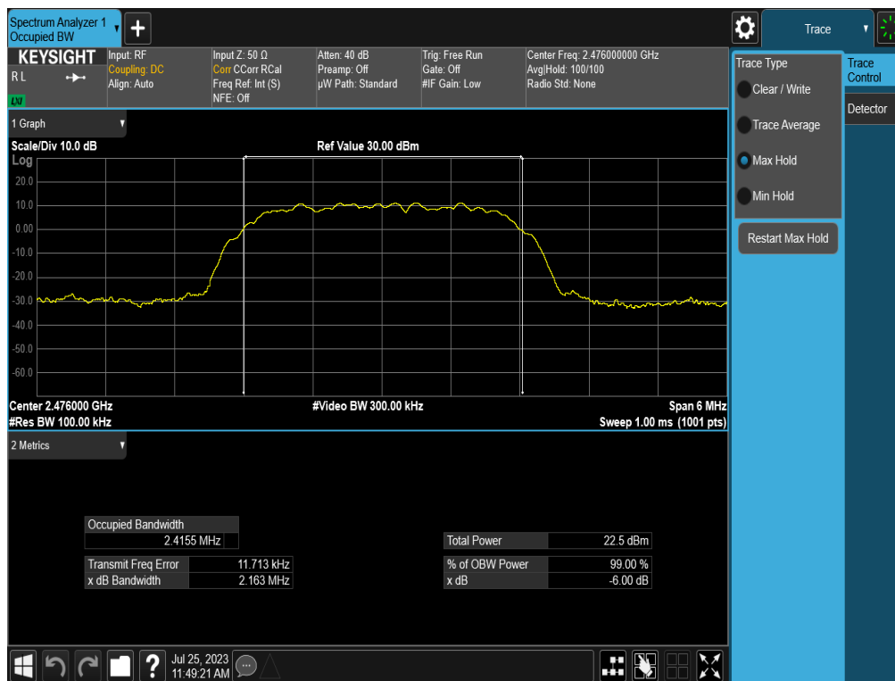
Plot 7-3. 6dB BW & 99% OBW Plot (Bluetooth (HDR4), 4Mbps, ePA – Ch. 73)
