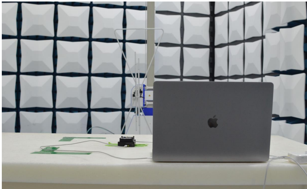
Figure 13: 30MHz-1GHz Test Setup (Rear View)
