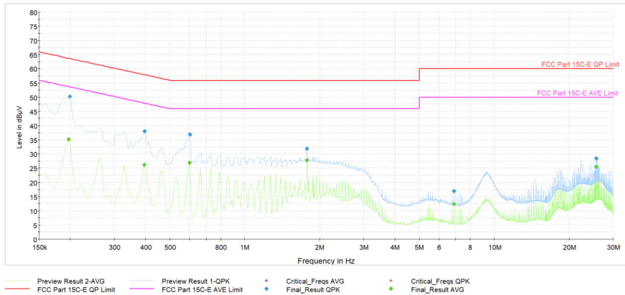
Plot 7-42. AC Line Conducted (Ch. 5, Config 409, Payload 4093 N, with PC via USB-C cable with magnetic charger)
