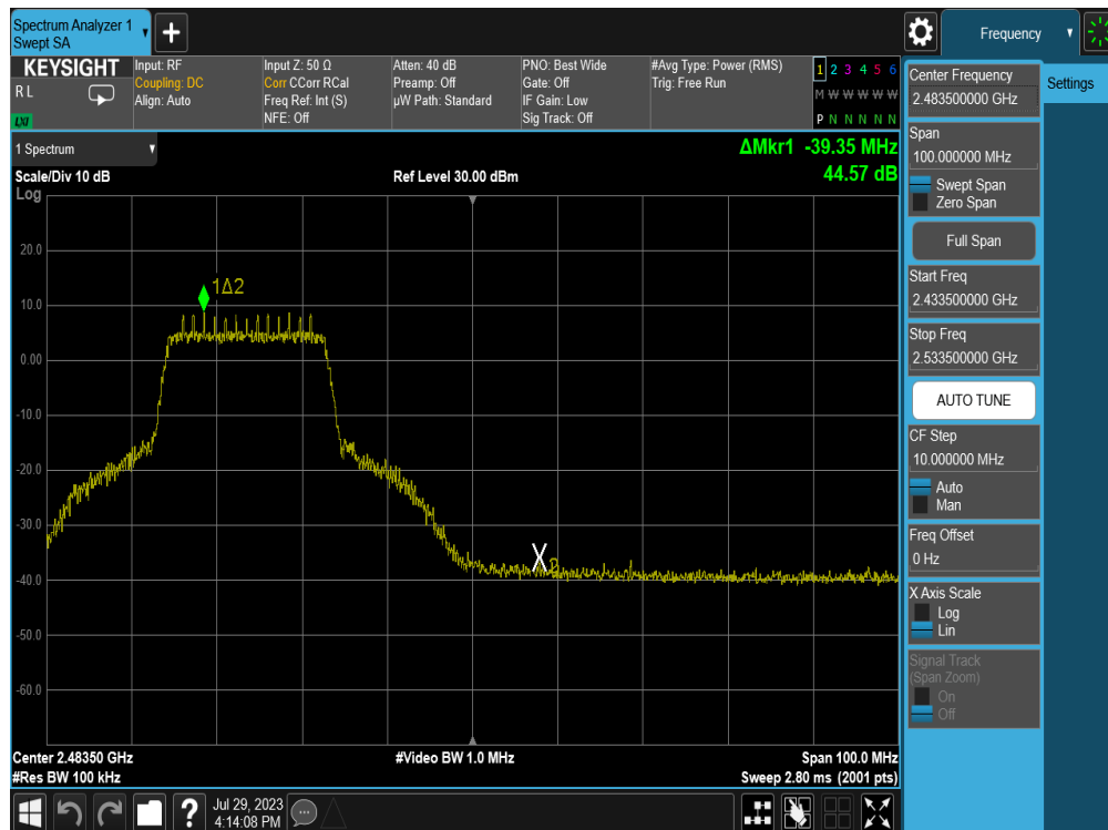
Plot 7-36. Band Edge Plot (802.11n (2.4GHz) – Ch. 10) – MCS0
