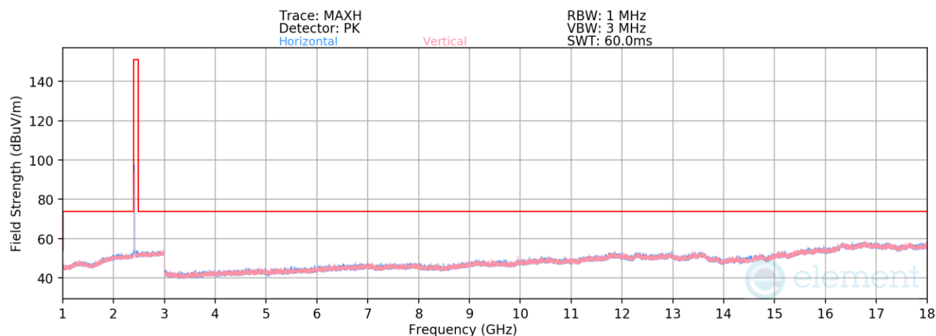
Plot 7-52. Radiated Spurious Emissions above 1GHz (802.11b – Ch. 1)
