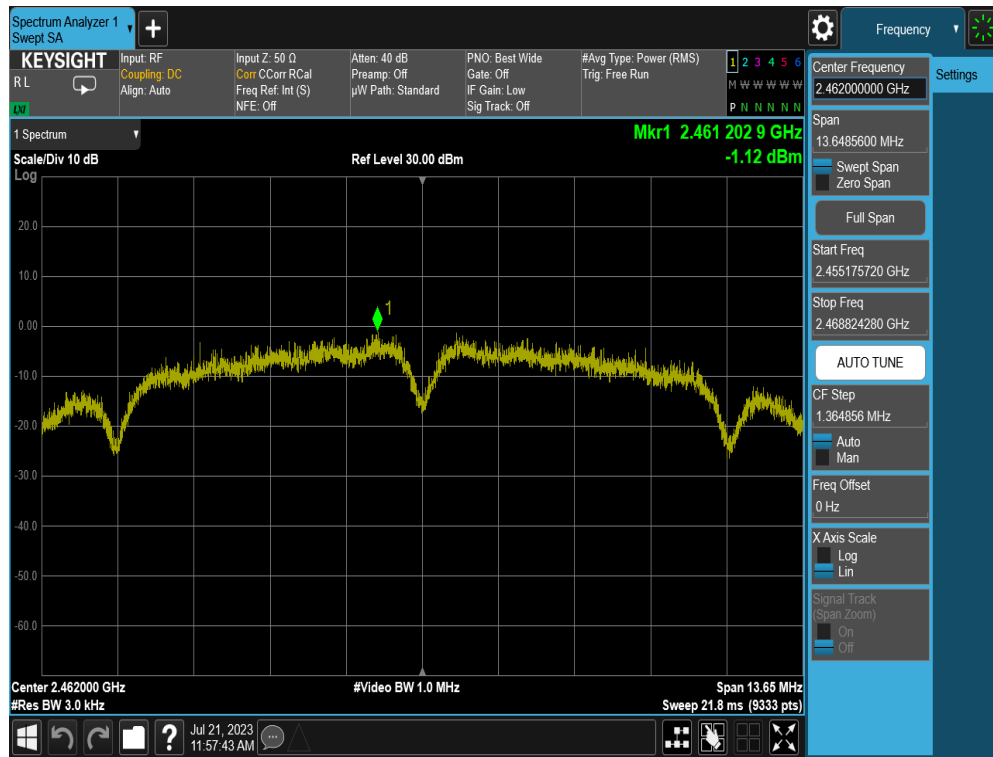
Plot 7-15. Power Spectral Density Plot (802.11b – Ch. 11) – 1Mbps
