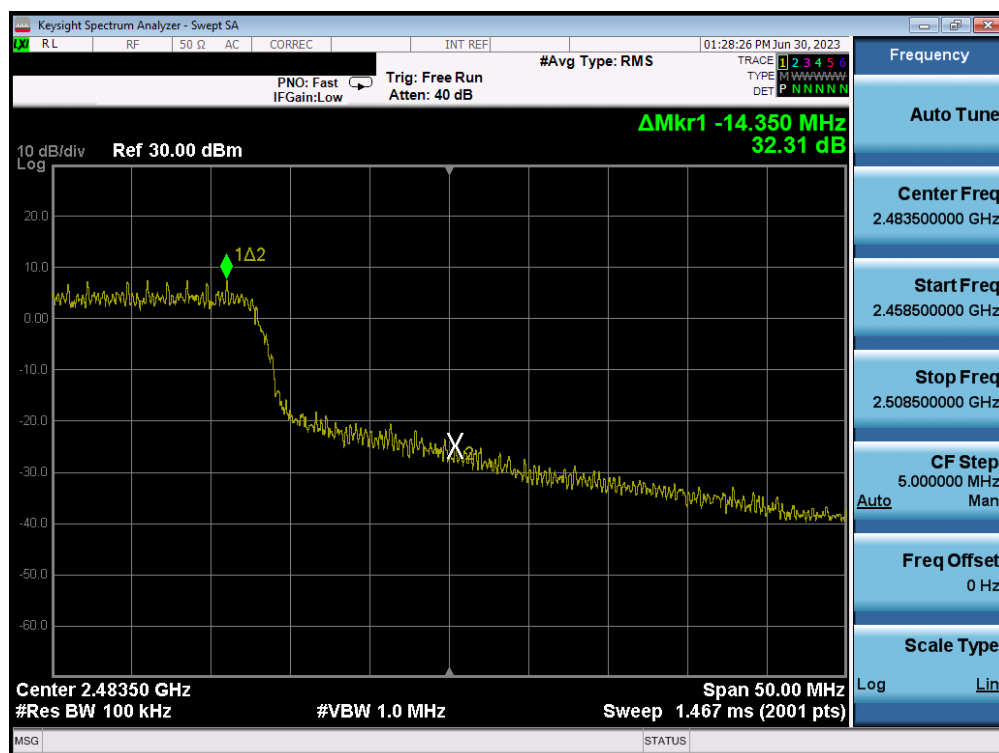
Plot 7-45. Band Edge Plot (802.11n (2.4GHz) – Ch. 13) – MCS7
