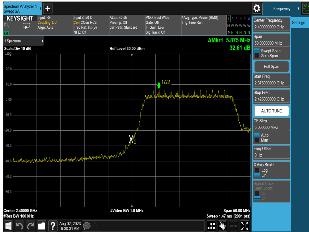
Plot 7-35. Band Edge Plot (802.11n (2.4GHz) – Ch. 2) – MCS0
