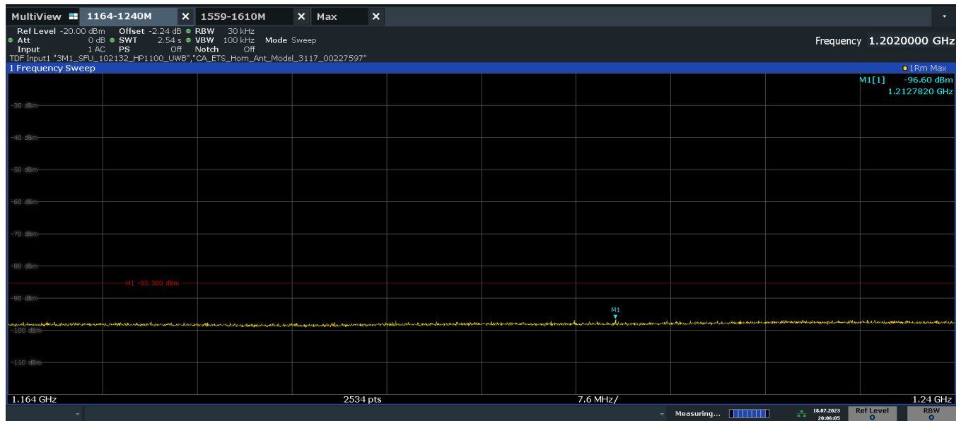
Plot 7-11. Radiated Spurious Emission 1164-1240MHz (Ch. 9, Config 0, Payload 125 Ant. Pol H)
