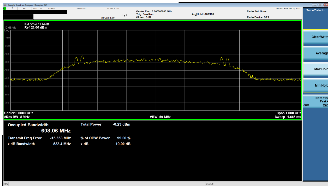
Plot 7-2. ISED 10dBc Bandwidth & 99% OBW (UWB, Ch. 9, Config 0/Payload 125)
