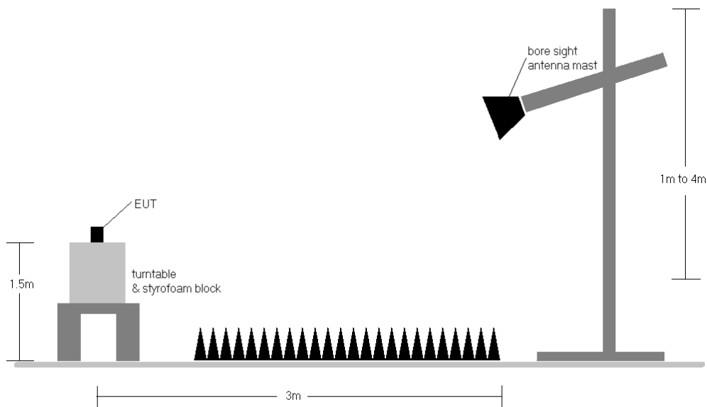
Figure 7-1. Test Setup
