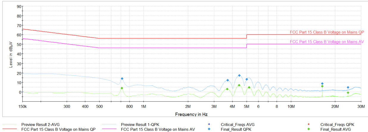
Plot 7-24. AC Line Conducted (Ch.9, Config 0, Payload 125, N, with AC/DC Adapter)
