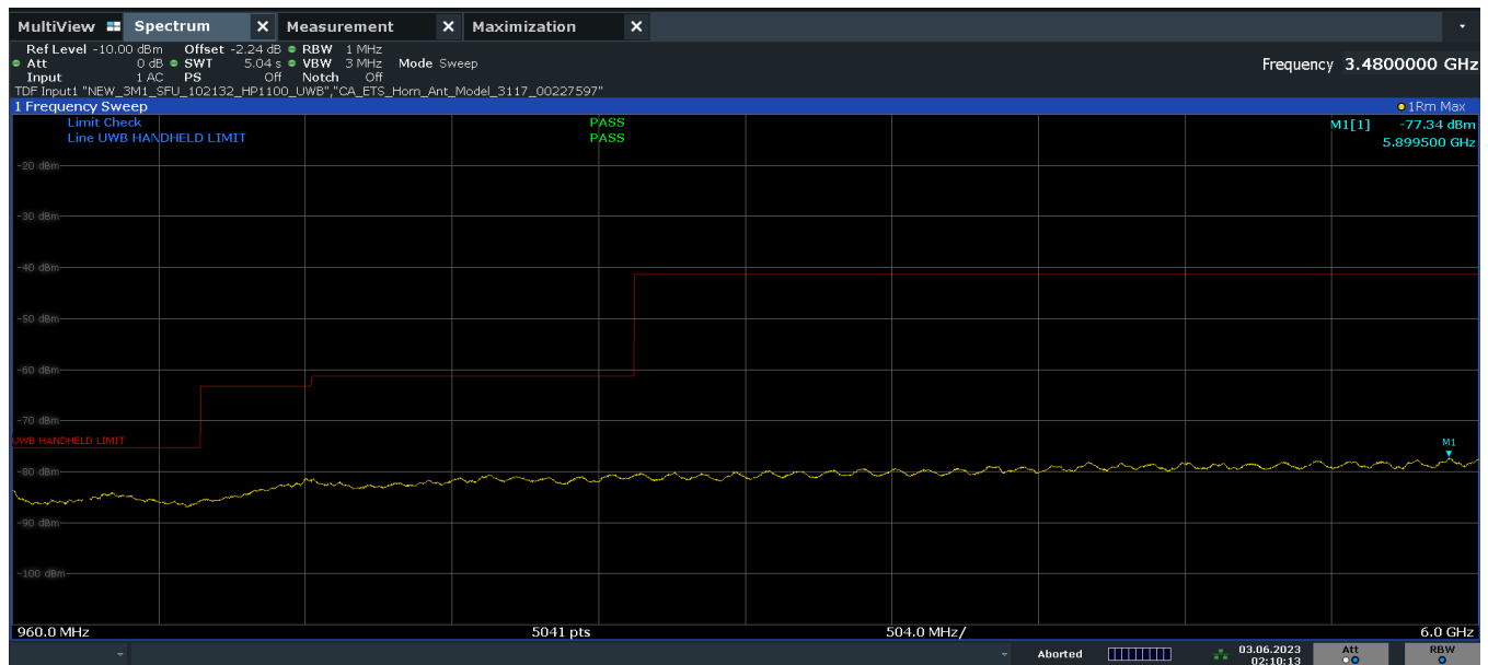
Plot 7-8. FCC Radiated Spurious Emission 960-6000MHz (Ch. 9, Config 0, Payload 125 Ant. Pol. V)
