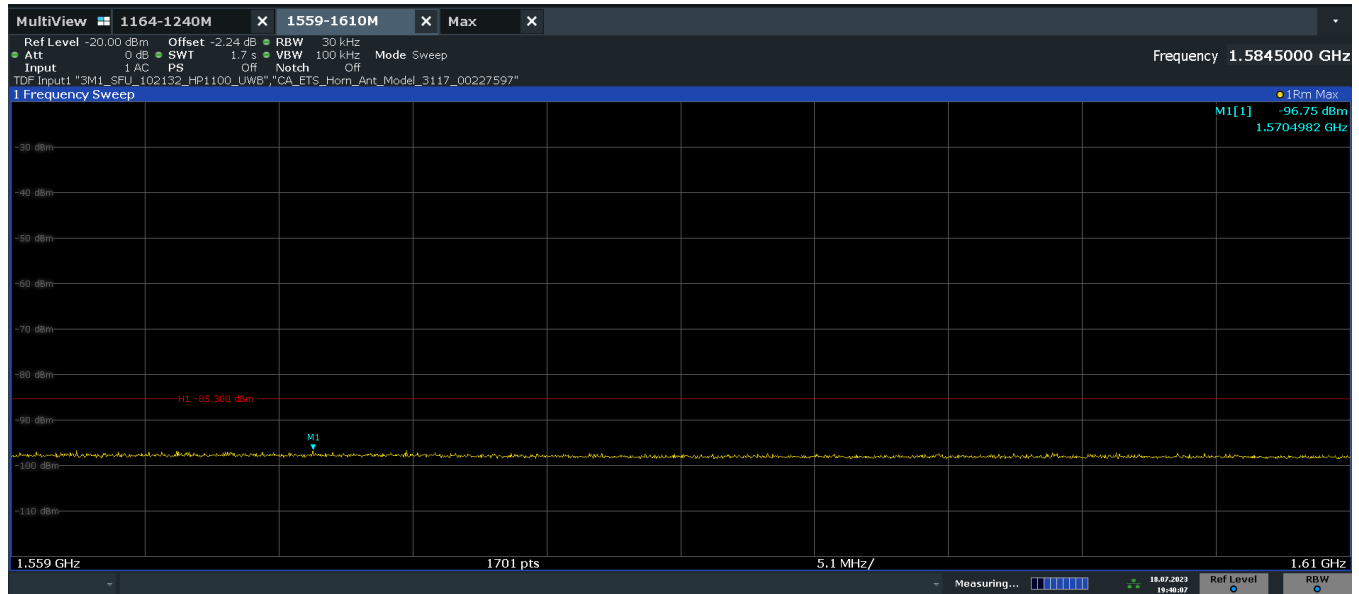
Plot 7-13. Radiated Spurious Emission 1559-1610MHz (Ch. 9, Config 0, Payload 125 Ant. Pol H)
