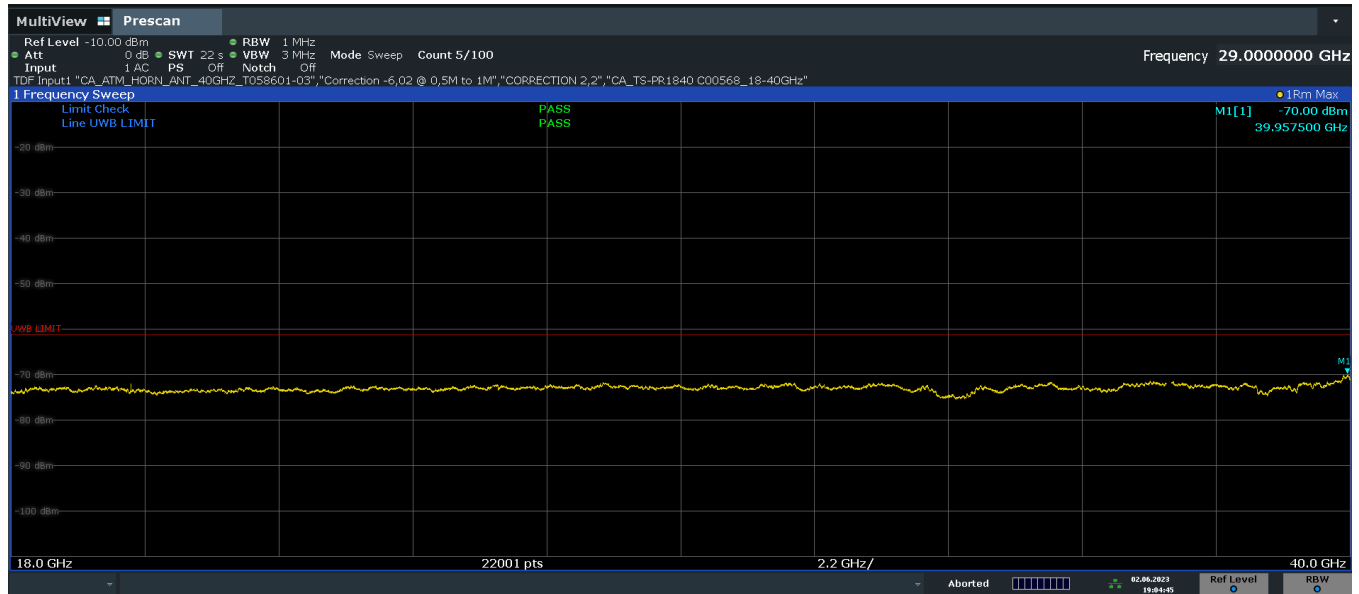
Plot 7-20. Radiated Spurious Simultaneous Transmission 18-40GHz (Ch.9, Config 3, Payload 125)
