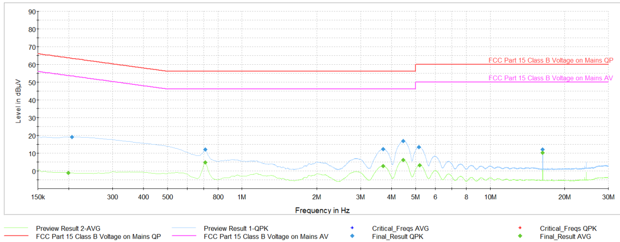
Plot 7-23. AC Line Conducted (Ch.9, Config 0, Payload 125, L1, with AC/DC Adapter)
