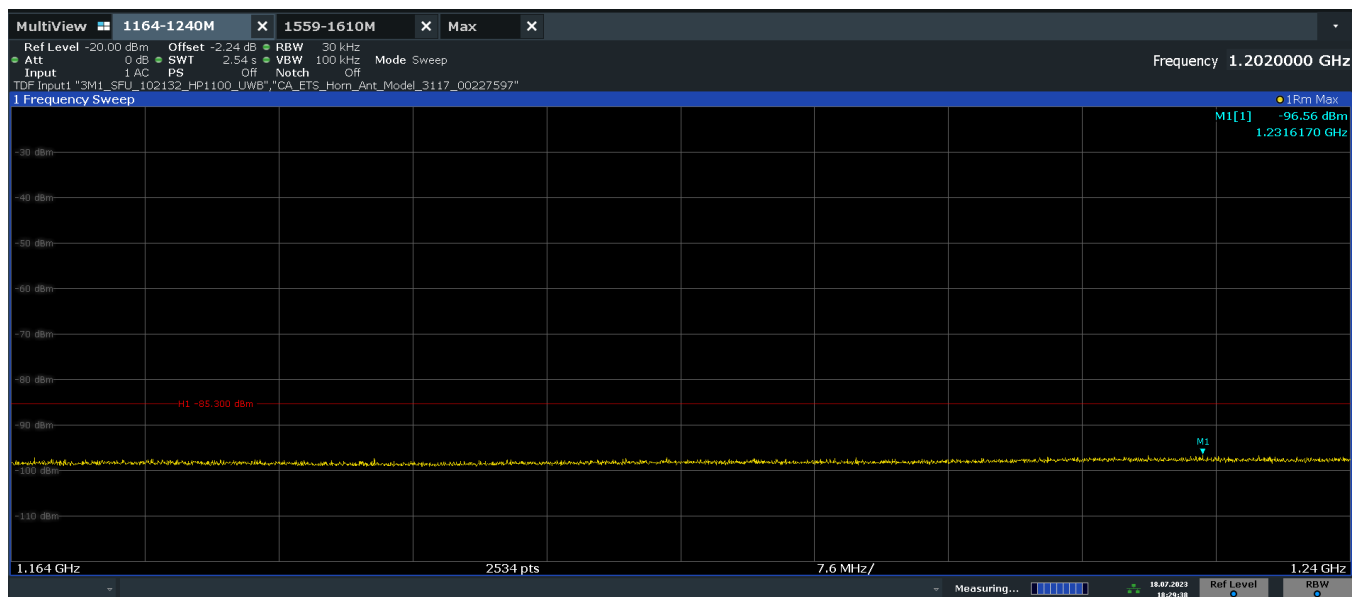
Plot 7-12. Radiated Spurious Emission 1164-1240MHz (Ch. 9, Config 0, Payload 125 Ant. Pol V)
