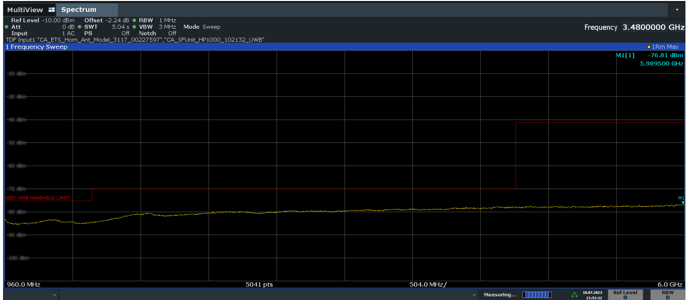
Plot 7-9. ISED Radiated Spurious Emission 960-6000MHz (Ch. 9, Config 0, Payload 125 Ant. Pol. H)
