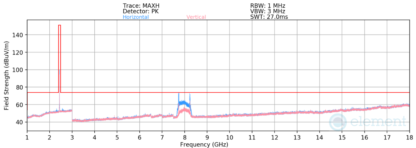
Plot 7-19. Radiated Spurious Simultaneous Transmission 1-18GHz (Ch.9, Config 3, Payload 125)
