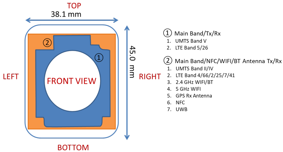
Figure B-1 DUT Antenna Locations
