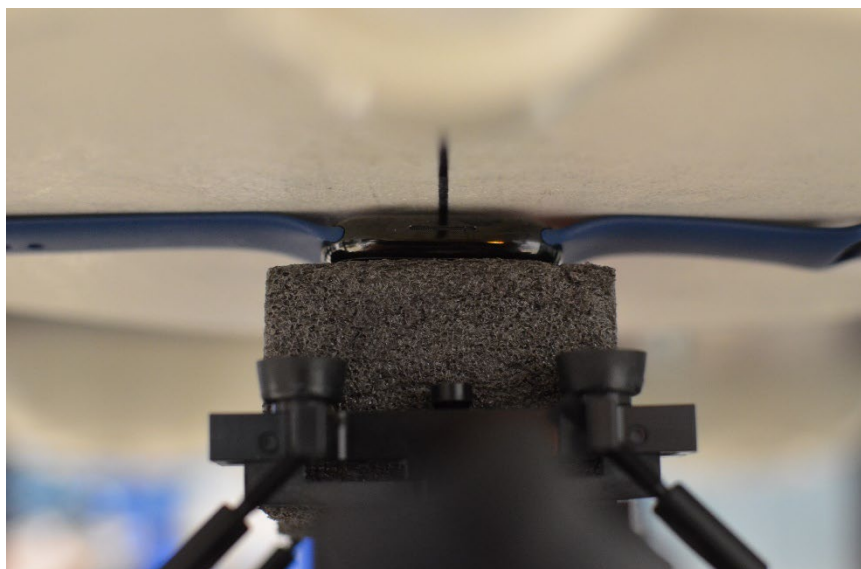
SAR Test Setup Photo 13: Stainless Steel with Sport Wristband, Extremity, Back Side at 0.0 cm
