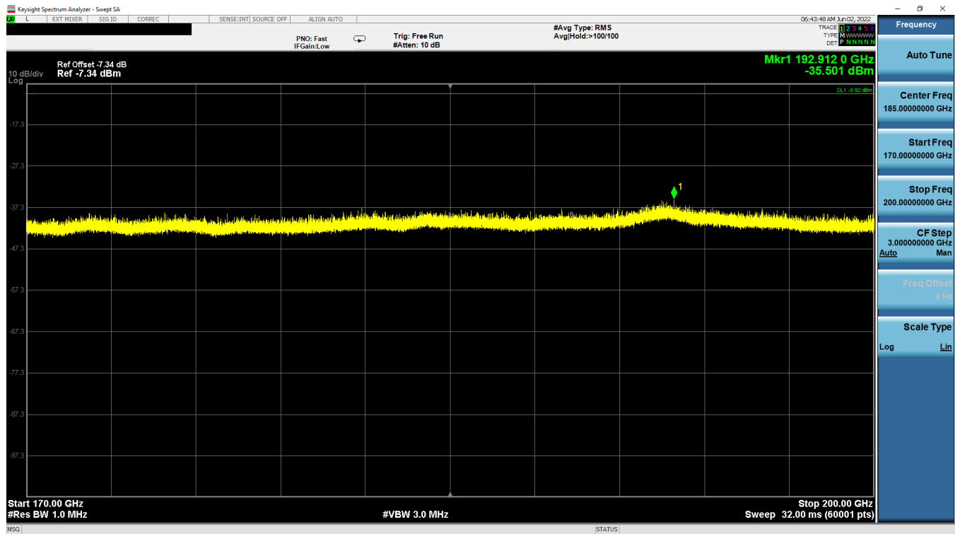
Plot 6-7. Radiated Spurious Emissions 170GHz – 200GHz (Mode 1)
