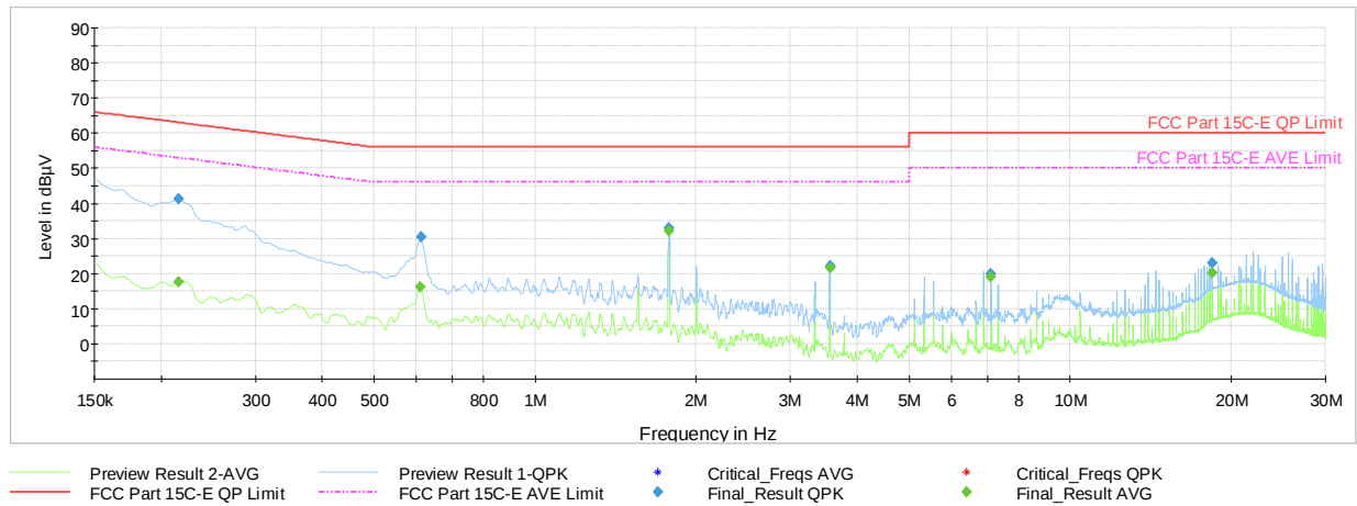
Plot 7-42. AC Line Conducted (Ch. 5, Config 0, Payload 125 N, with PC via USB-C cable with magnetic charger)
