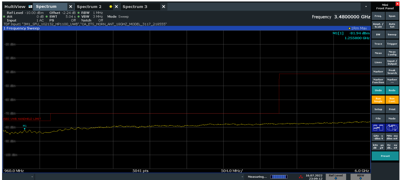
Plot 7-17. ISSED Radiated Spurious Emission 960-6000MHz (Ch. 5, Config 0, Payload 125 Ant. Pol. H)
