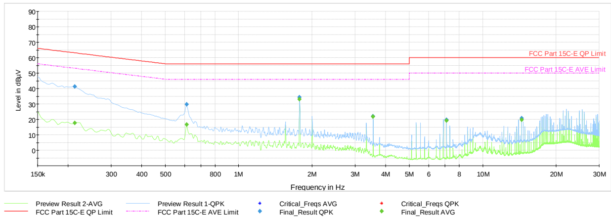
Plot 7-41. AC Line Conducted (Ch. 5, Config 0, Payload 125 L1, with PC via USB-C cable with magnetic charger)
