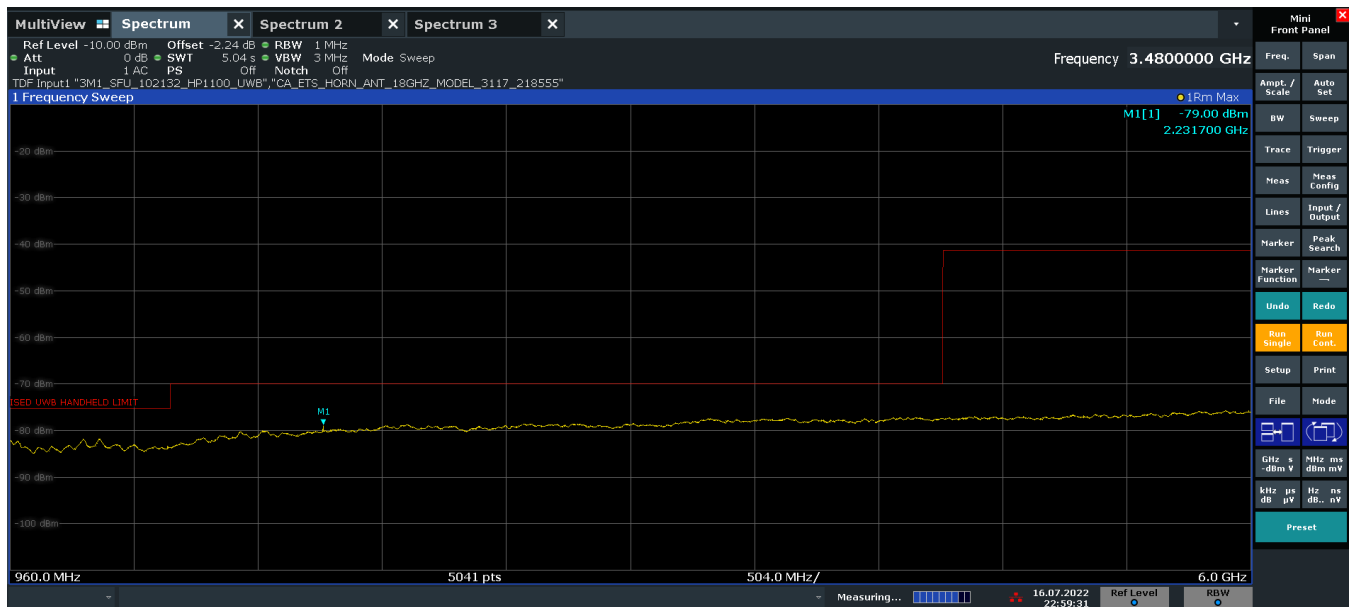
Plot 7-18. ISSED Radiated Spurious Emission 960-6000MHz (Ch. 5, Config 0, Payload 125 Ant. Pol. V)
